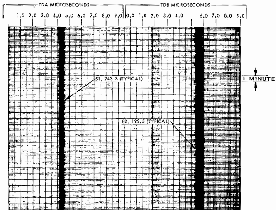
Figure 3-11A. Monitor Station TD Recording
