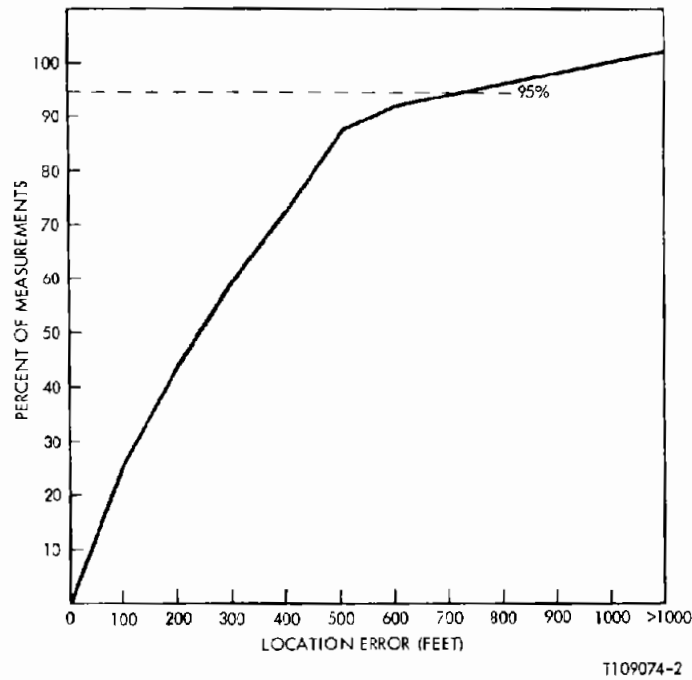
Figure 6-20B. Cumulative Location Error (System Simulation) (Random Route Tests #20001 - 20005)
