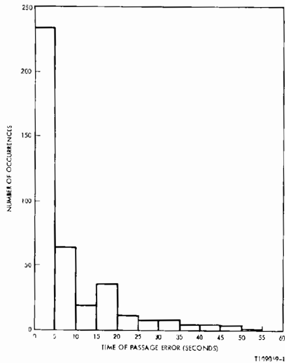
Figure 10A. Time of Passage Error Histogram (Fixed Route Tests (All) Except #10016 and 10017)
