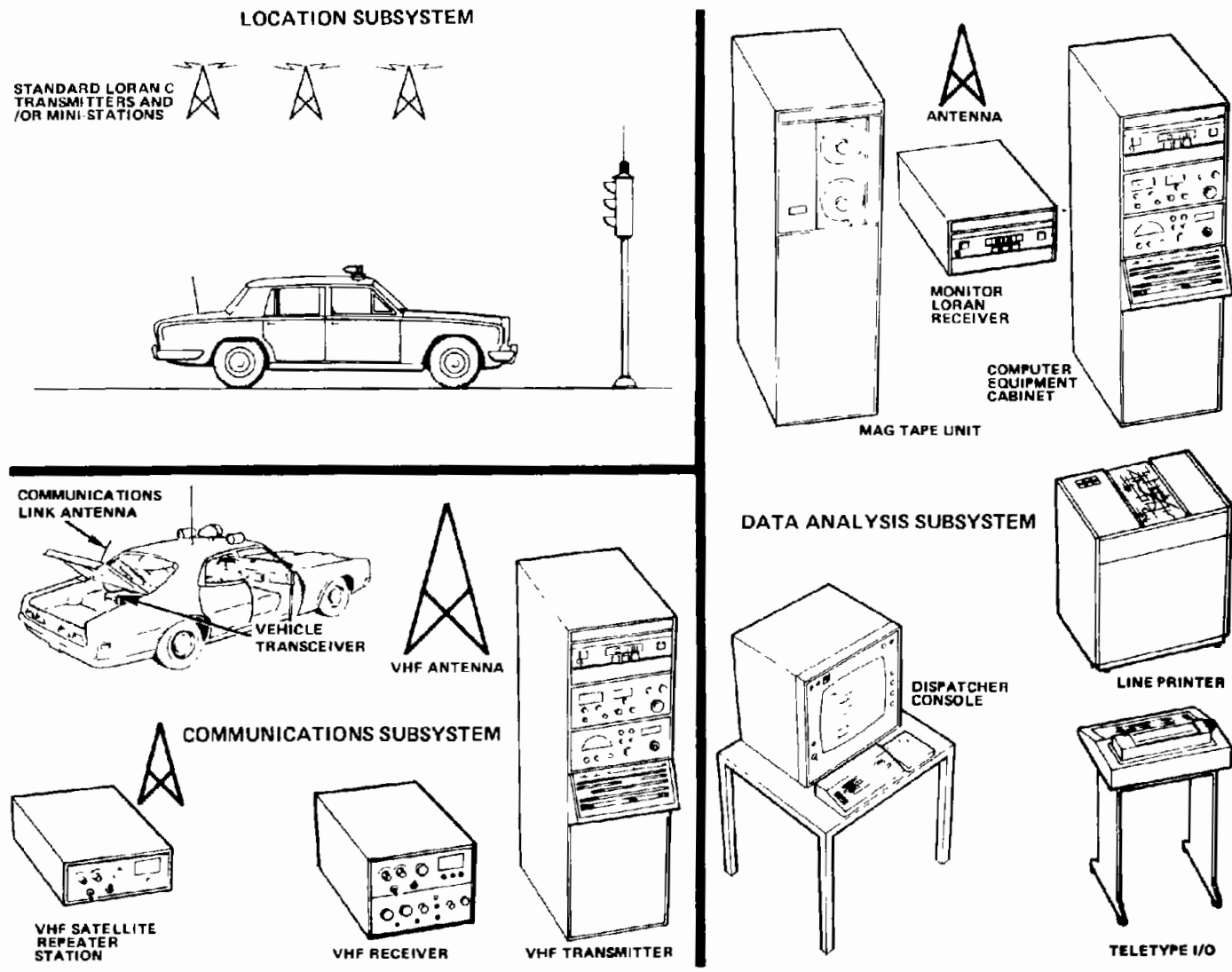
Figure 1-5. LORAN AVM System Components
