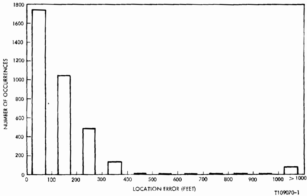
Figure 6-11A. Location Accuracy Histogram (System Simulation With 5% Missing Data) (Fixed Route Tests (All) Except #10016 and 10017)
