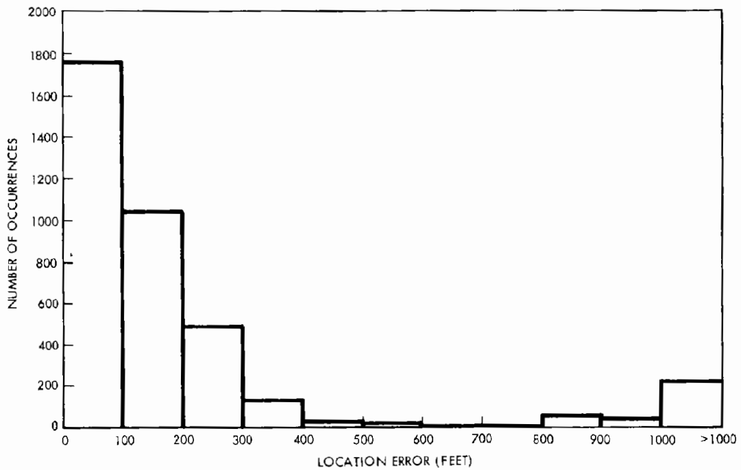
Figure 6-7A. Location Accuracy Histogram (System Simulation With 5% Missing Data) (Fixed Route Tests #10012 - 10047)
