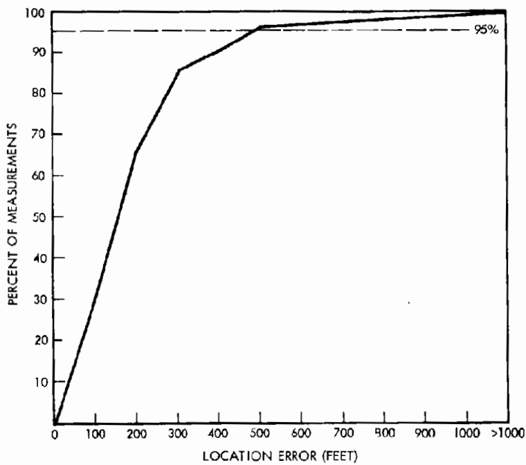
Figure 6-23A. Location Accuracy Histogram (System Simulation and Improved Software) (Random Route Tests #20001 - 20005)
