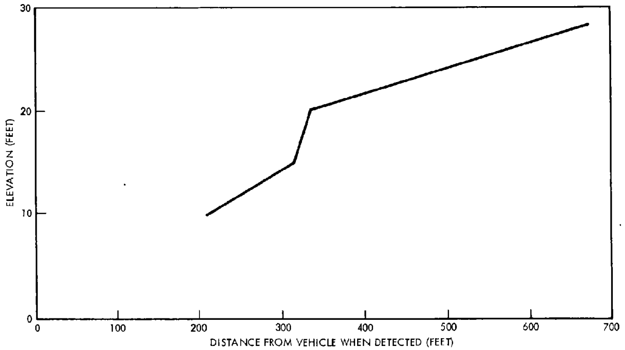
Figure 6-31A. Augmentor Detection Distance (In Traffic) Vs. Elevation
