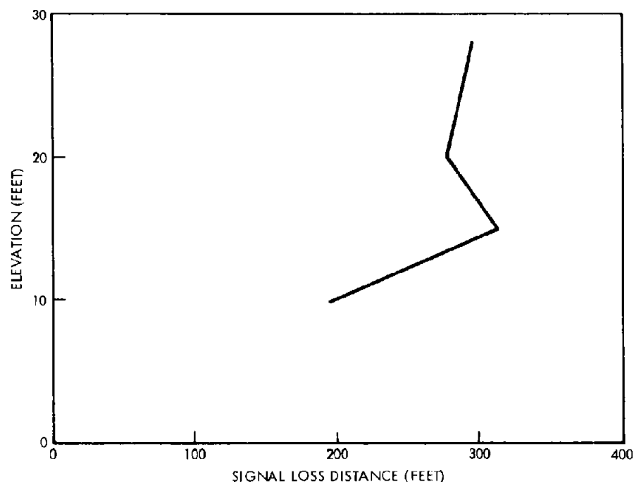
Figure 6-31B. Augmentor Signal Loss Distance (In Traffic) Vs. Elevation
