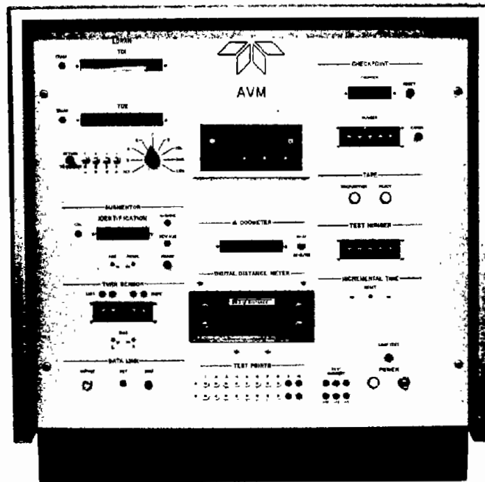
Figure 3-8. LAVM Test Console
