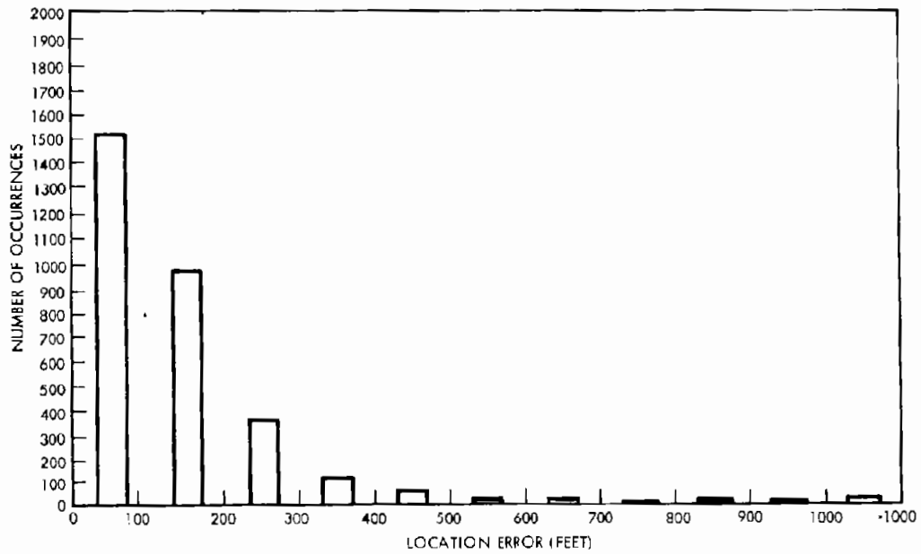
Figure 6-4A. Location Subsystem Histogram (Fixed Route Tests (All) #10012 - 10047)
