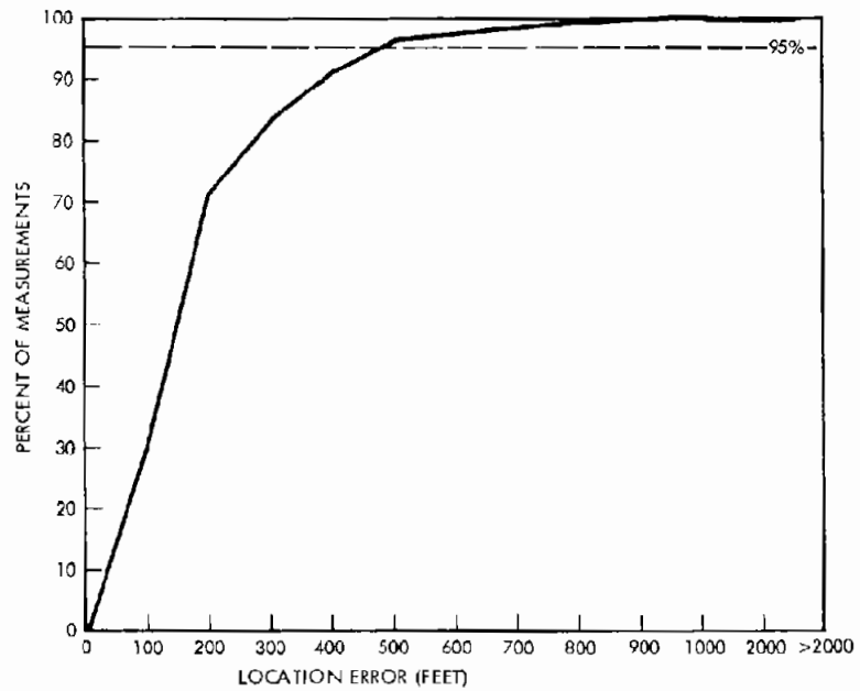
Figure 6-22A. Location Accuracy Histogram (System Simulation With 5% Missing Data and Improved Software) (Random Route Tests #20001 - 20005)
