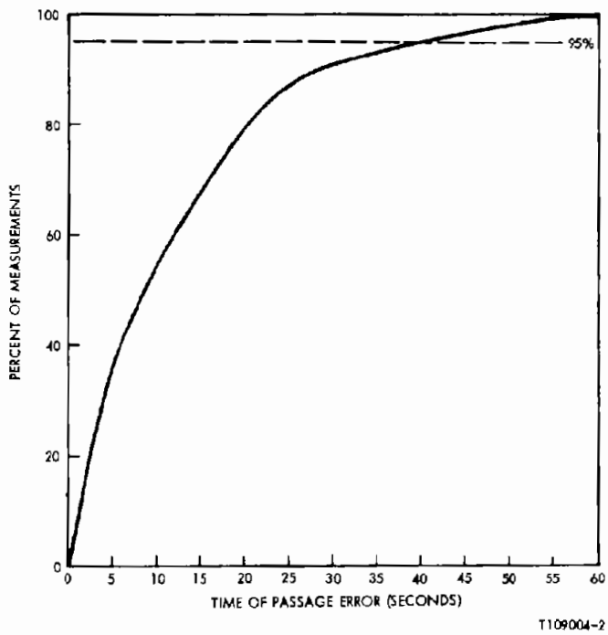
Figure 6-16B. Time of Passage Cumulative Error (Stop Time Points)
