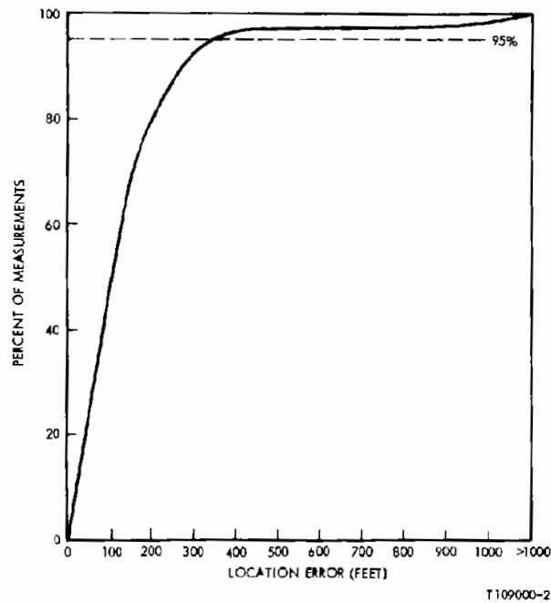
Figure 6-9B. Cumulative Location Error (System Simulation) (Fixed Route Tests (All) Less #10016 and 10017)
