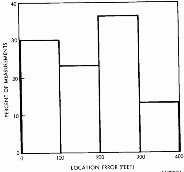
Figure 6-24A. LORAN Only Test - Location Accuracy Histogram (32 Second Fixed Polling)
