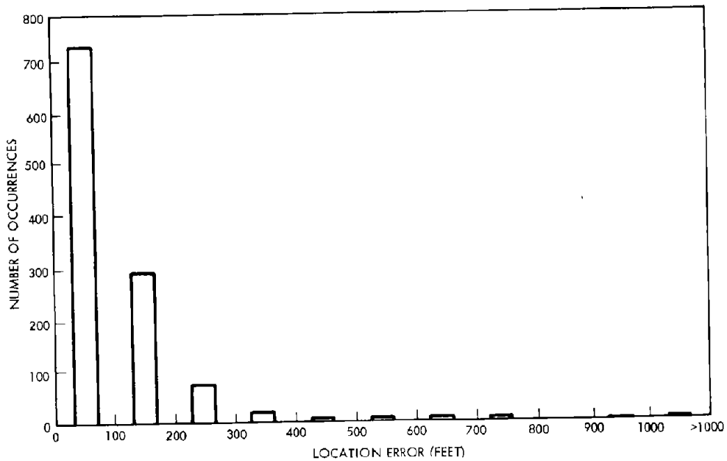
Figure 6-3A. Location Accuracy Histogram (System Simulation) (Fixed Route Tests #10001 - 10012) December 1976
