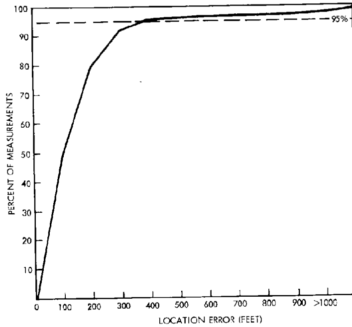
Figure 6-8B. Location Subsystem Cumulative Error (Fixed Route Tests (All) Less #10016 and 10017)
