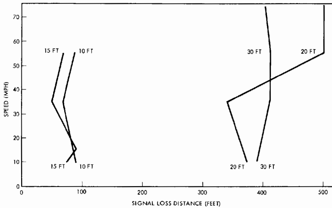
Figure 6-27B. Vehicle Speed Vs. Signal Loss Distance
