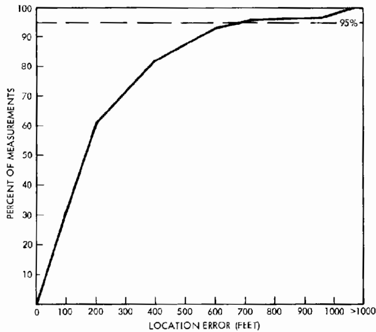
Figure 6-21A. Location Accuracy Histogram (System Simulation With 5% Missing Data) (Random Route Tests #20001 - 20005)
