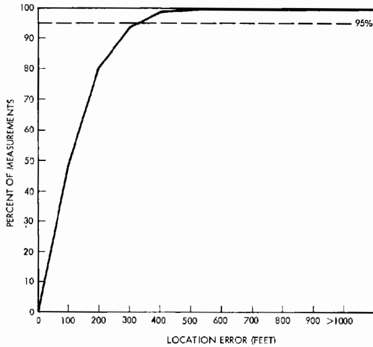
Figure 6-12B. Location Subsystem Cumulative Error (Fixed Route Tests #10026 - 10047)
