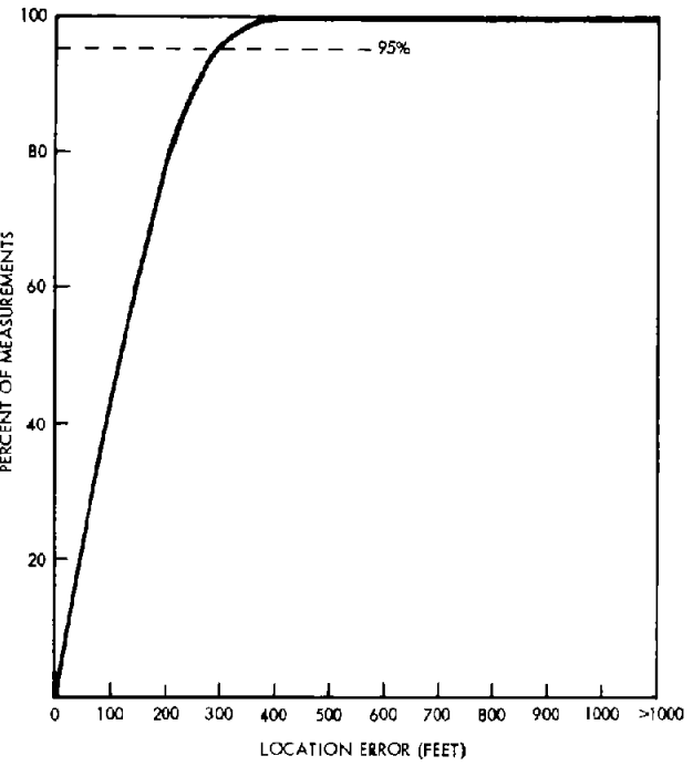
Figure 6-13B. Cumulative Location Error (System Simulation) (Fixed Route Tests #10026 - 10047)
