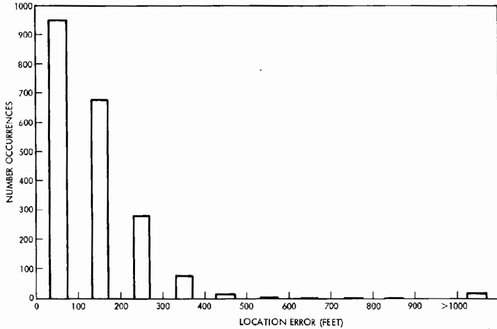
Figure 6-12A. Location Subsystem Error Histogram (Fixed Route Tests #10026 - 10047)
