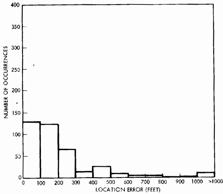
Figure 6-21A. Location Accuracy Histogram (System Simulation With 5% Missing Data) (Random Route Tests #20001 - 20005)
