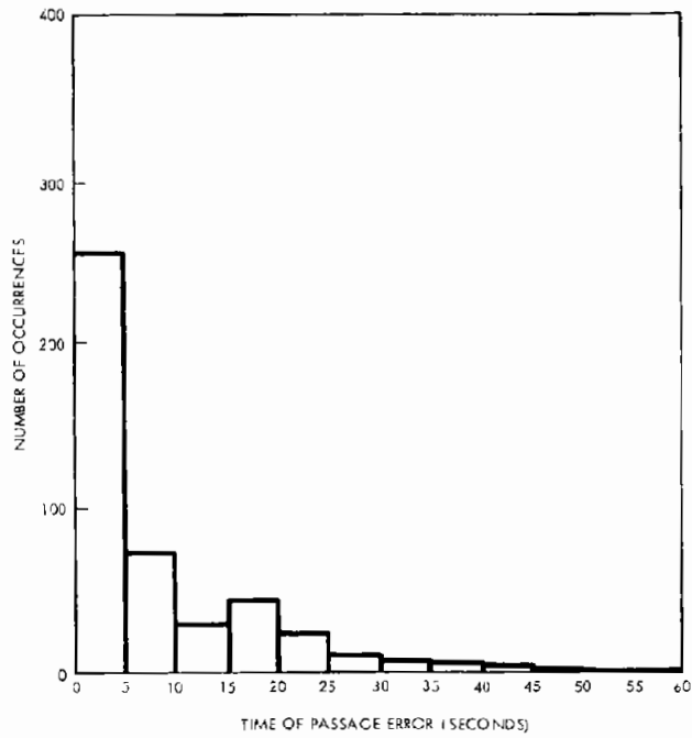
Figure 6-6A. Time of Passage Error Histogram (Test 10012 - 10047)
