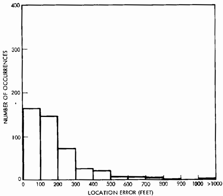
Figure 6-23A. Location Accuracy Histogram (System Simulation and Improved Software) (Random Route Tests #20001 - 20005)
