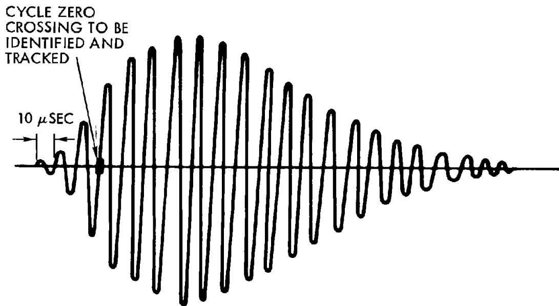
Figure 2-3b. LORAN-C Signal Format
