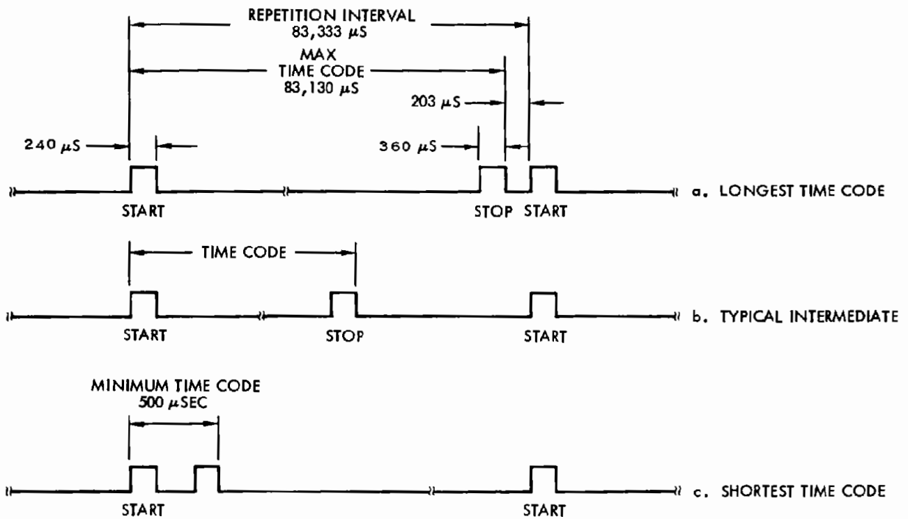
Figure 2-28. Augmentor Timing Code
