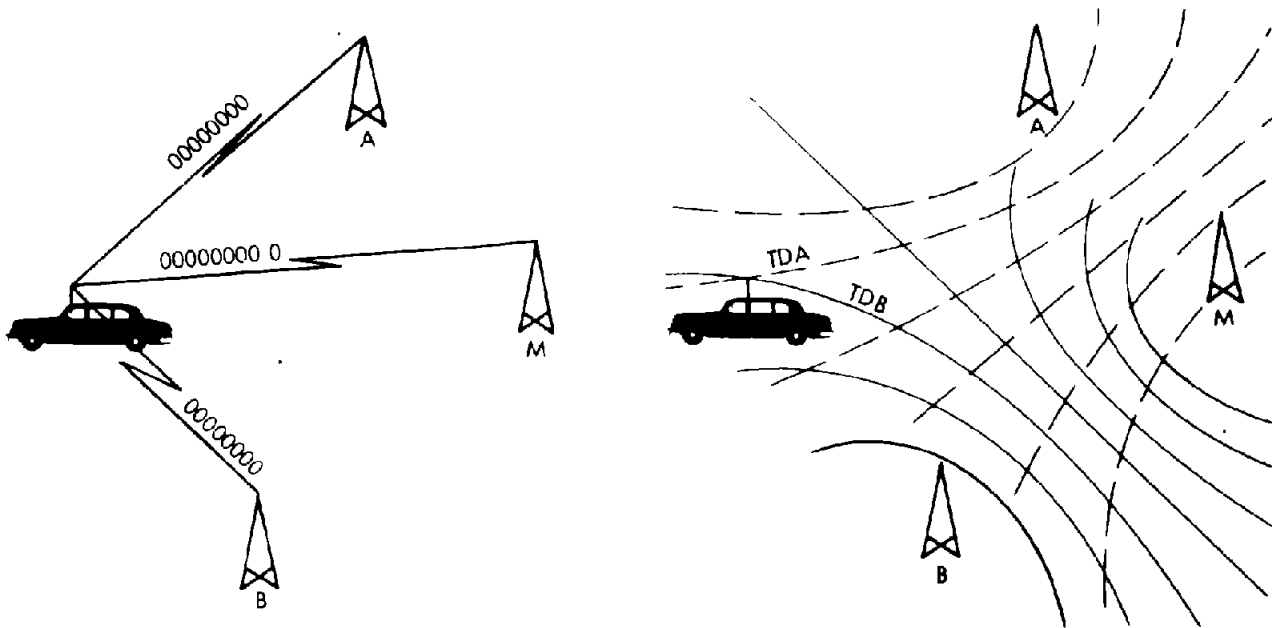
Figure 1-1. Hyperbolic Fix Geometry
