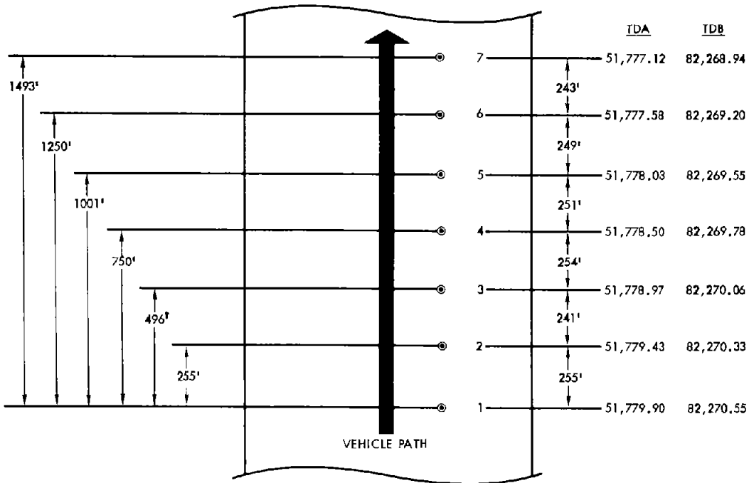
Figure 6-25. Runway Path and Checkpoint Diagram
