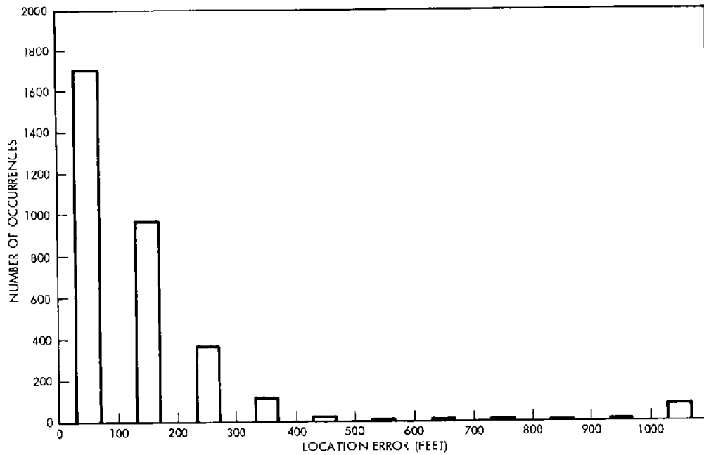
Figure 6-8A. Location Subsystem Histogram (Fixed Route Tests (All) Less #10016 and 10017)
