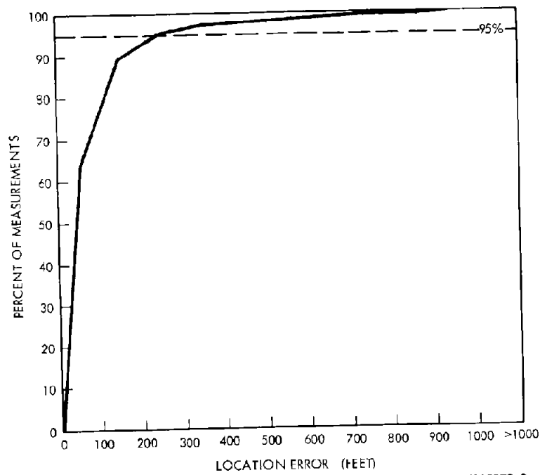
Figure 6-3B. Cumulative Location Error (System Simulation) (Fixed Route Tests #10001 - 10012) December 1976
