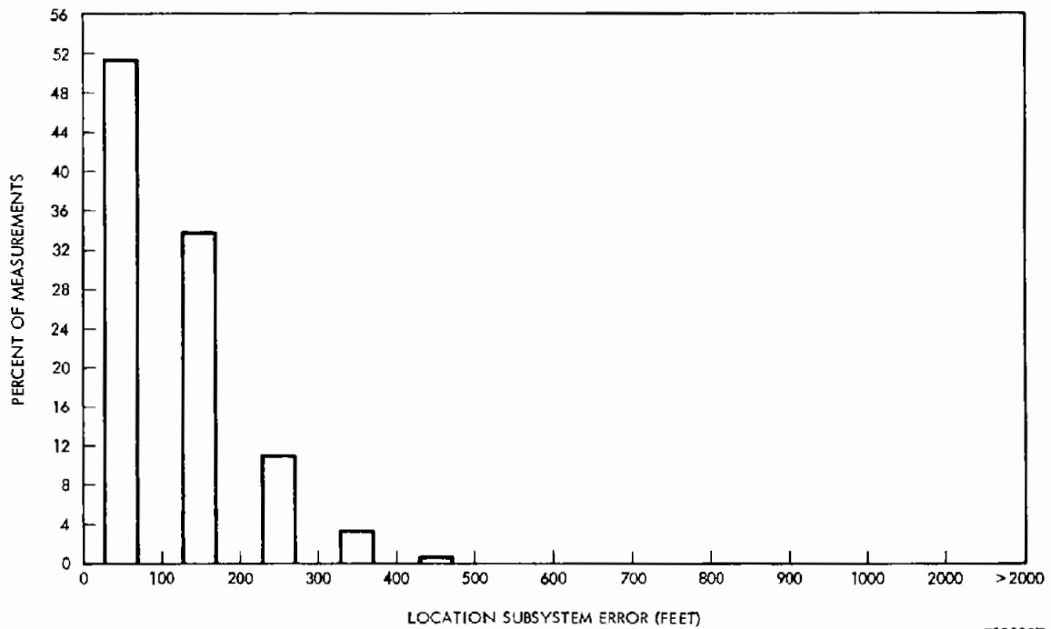
Figure 6-36. Location Subsystem Nighttime Accuracy (Fixed Route Tests #10026 - 10047)
