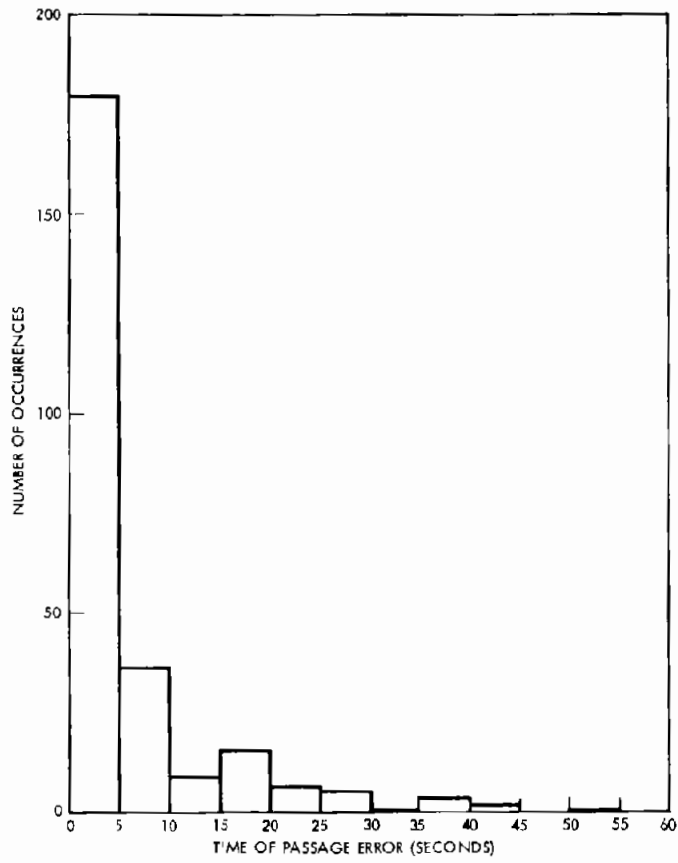
Figure 6-14A. Time of Passage Histogram (Fixed Route Tests #10026 - 10047)
