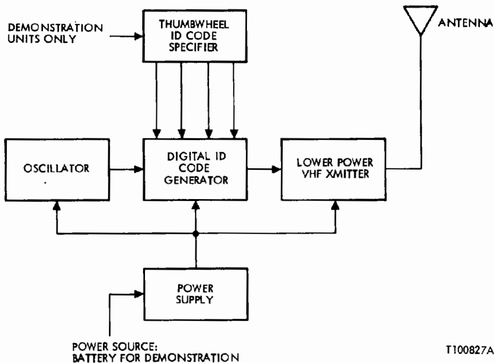
Figure 1-8. Block Diagram of Augmentor
