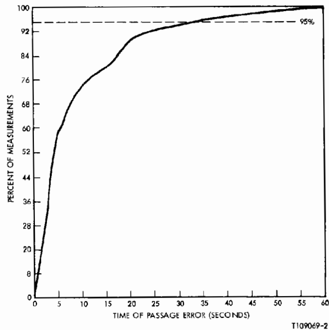
Figure 6-10B. Time of Passage Cumulative Error (Fixed Route Tests (All) Except #10016 and 10017)
