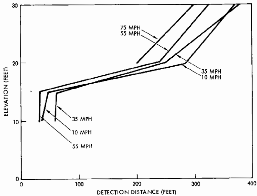
Figure 6-28A. Augmentor Elevation Vs. Detection Distance
