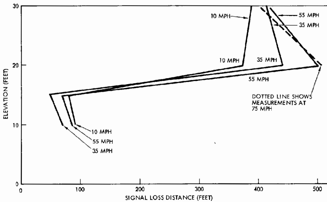
Figure 6-28B. Elevation Vs. Loss Distance
