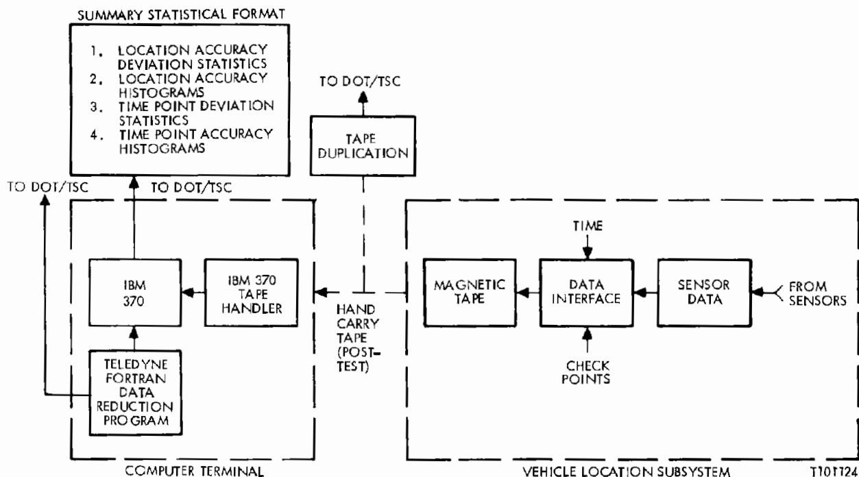
Figure 5-1. Data Handling Flow
