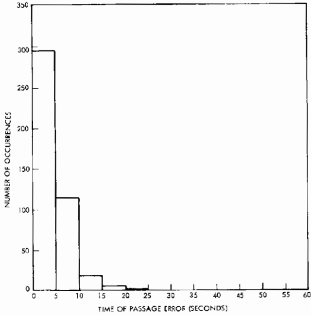
Figure 6-17A. Time of Passage Histogram (All Points - Dead Time Removed)
