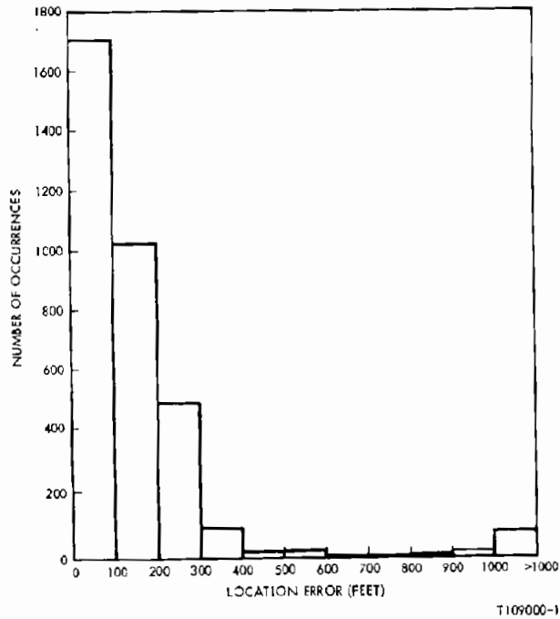
Figure 6-9A. Location Accuracy Histogram (System Simulation) (Fixed Route Tests (All) Less #10016 and 10017)
