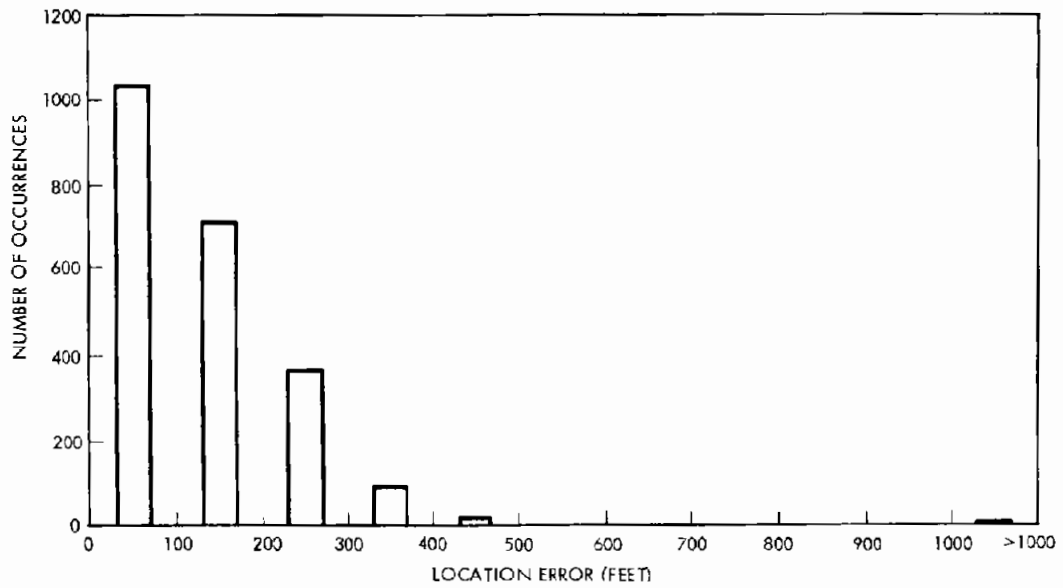
Figure 6-15A. Location Accuracy Histogram (System Simulation With 5% Missing Data) (Fixed Route Tests #10026 - 10047)
