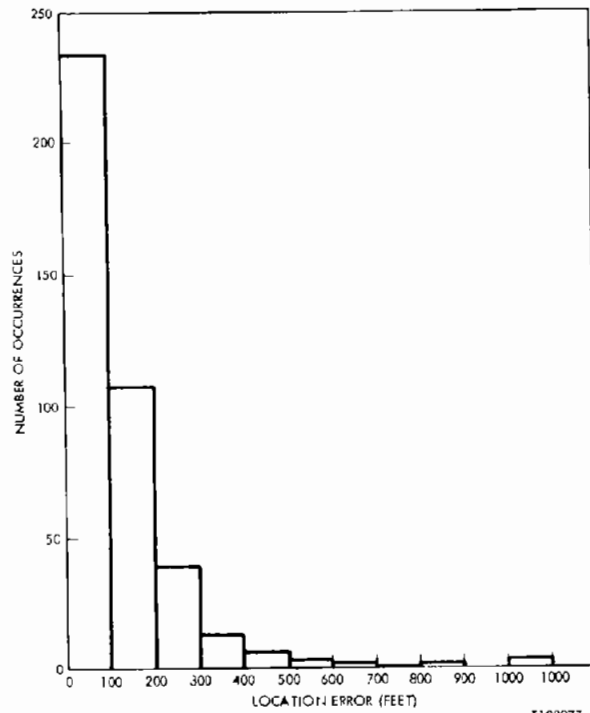
Figure 6-19A. Location Subsystem Histogram (Random Route Tests #20001 - 20005)
