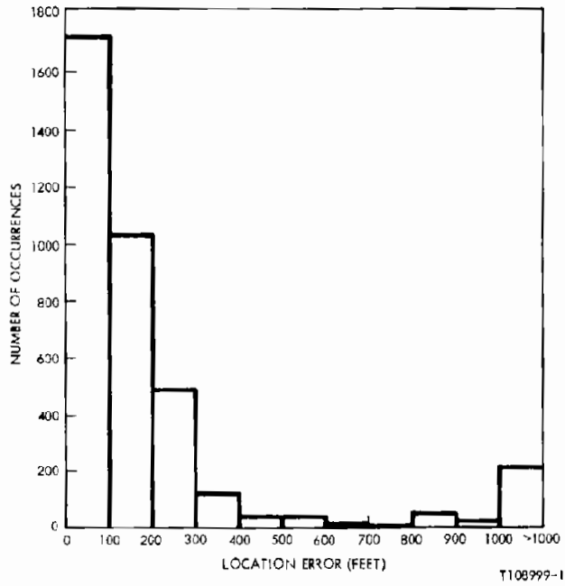
Figure 6-5A. Location Accuracy Histogram (System Simulation) (Fixed Route Tests #10012 - 10047)
