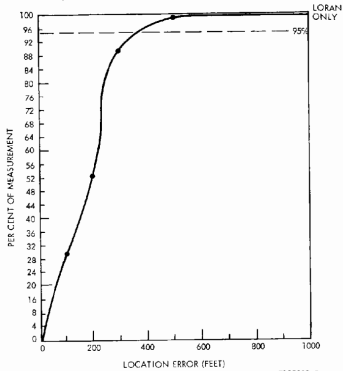
Figure 6-24B. LORAN Only Test - Location Cumulative Error (32 Second Polling)
