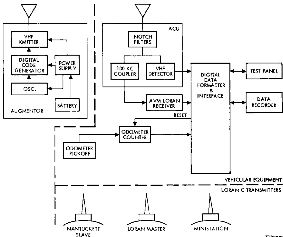
Figure 1-6. Location Subsystem
