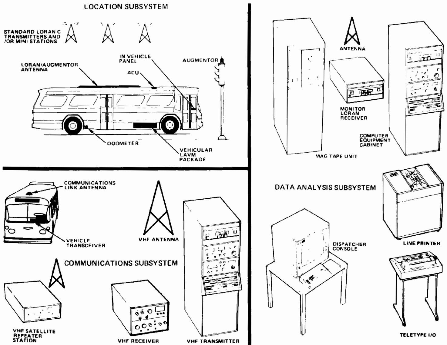
Figure 2-4. LAVM System
