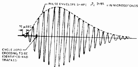
Figure 1-3. LORAN-C Pulse
