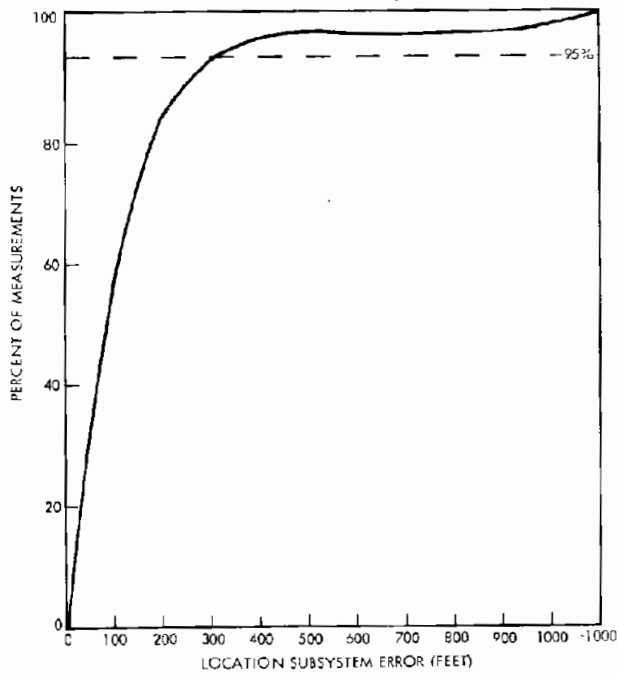
Figure 6-2B. Location Subsystem Cumulative Error (Fixed Route Tests #10001 - 10012) December 1976
