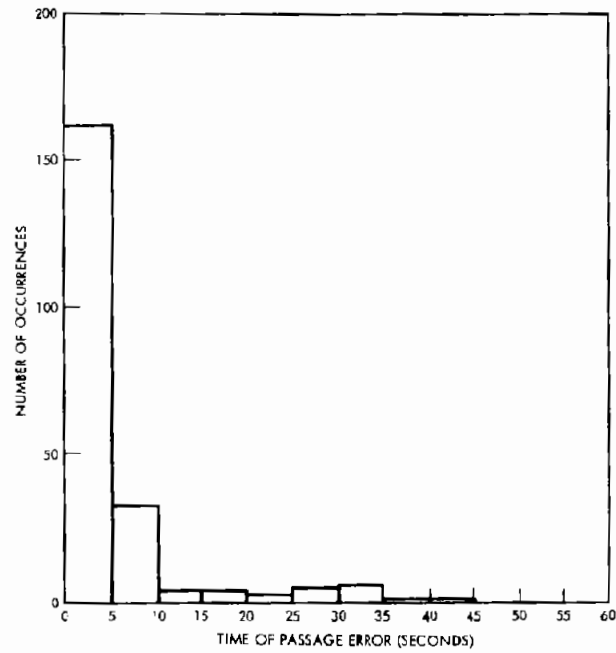
Figure 6-18A. Time of Passage Histogram (No Stop Time Points)
