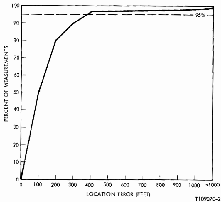
Figure 6-11B. Cumulative Location Error (System Simulation With 5% Missing Data) (Fixed Route Tests (All) Except #10016 and 10017)
