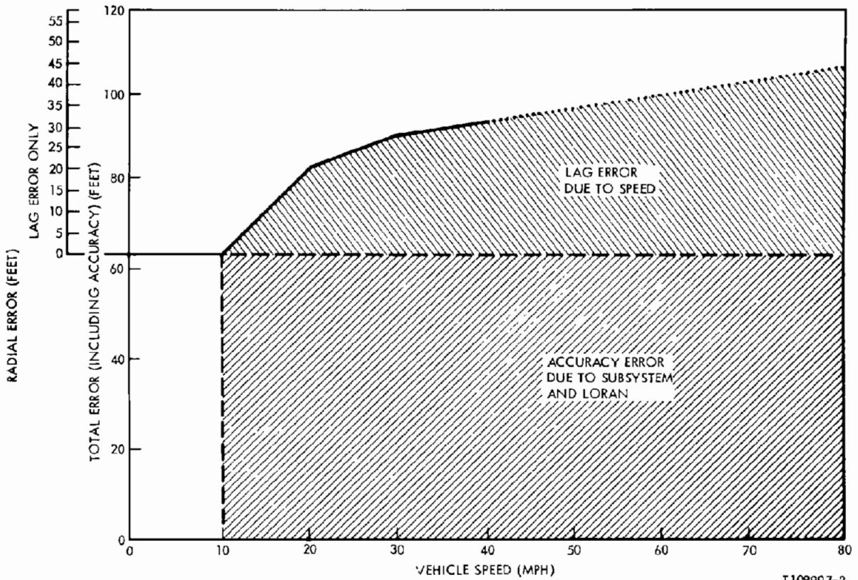
Figure 6-26. LORAN Speed/Lag Tests - Radial Error vs Speed
