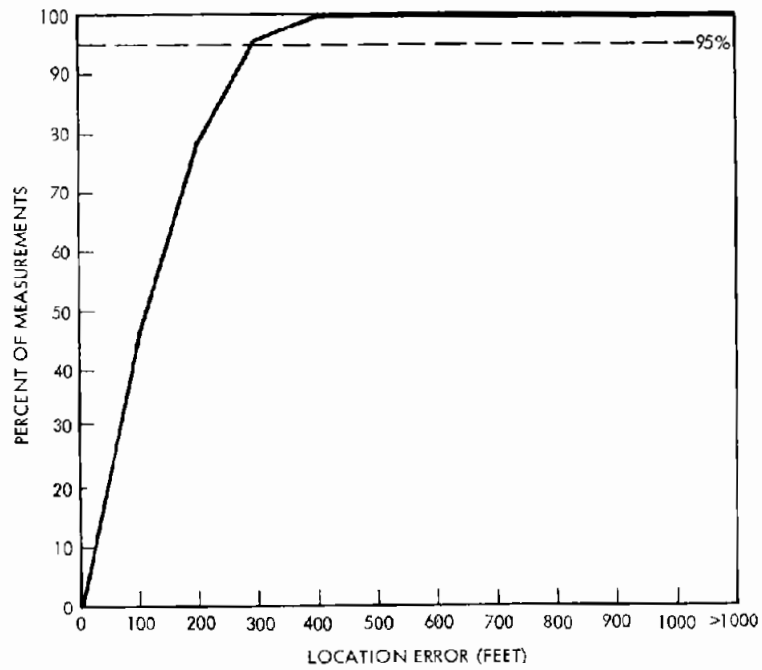
Figure 6-15B. Cumulative Location Error (System Simulation With 5% Missing Data) (Fixed Route Tests #10026 - 10047)
