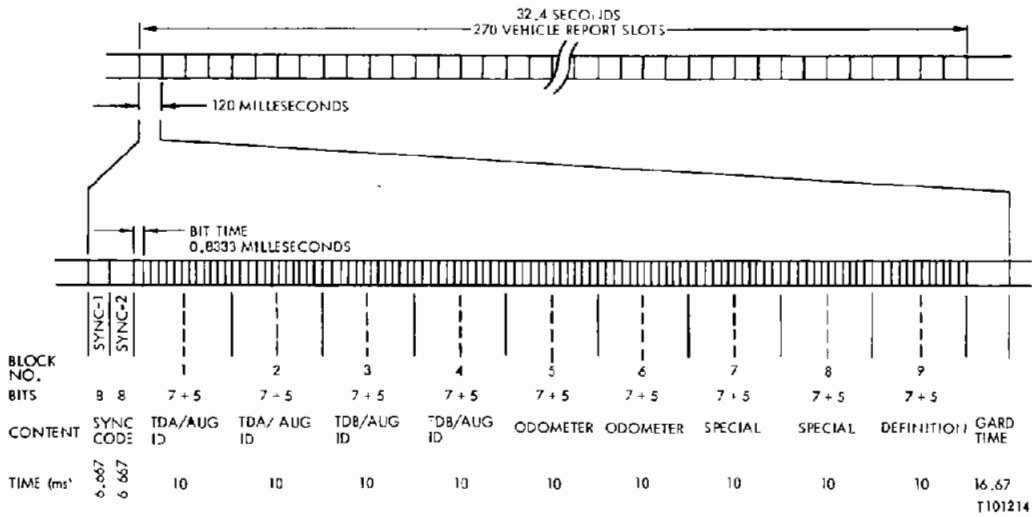
Figure 2-9. Vehicle Transmission Sequence
