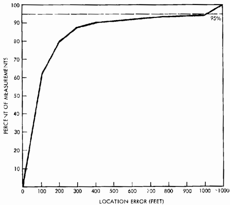
Figure 6-4B. Location Subsystem Cumulative Error (Fixed Route Tests (All) #10012 - 10047)
