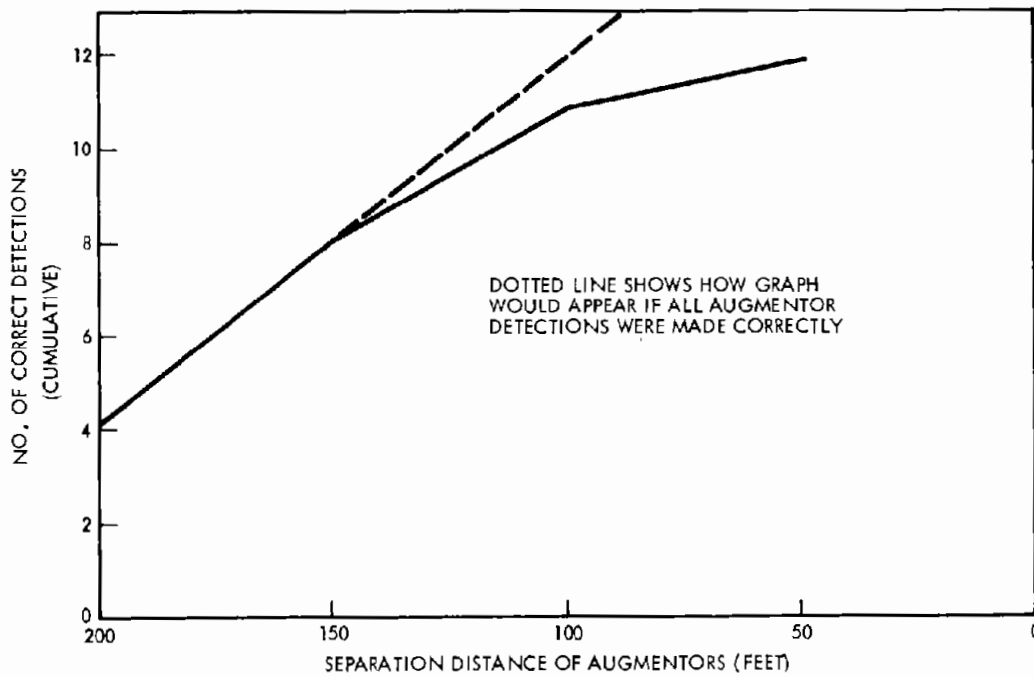
Figure 6-30. Augmentor Separation Distance vs. Number of Correct Detections (Cumulative)
