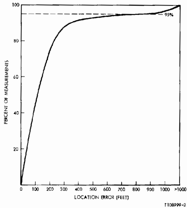
Figure 6-5B. Cumulative Location Error (System Simulation) (Fixed Route Tests #10012 - 10047)
