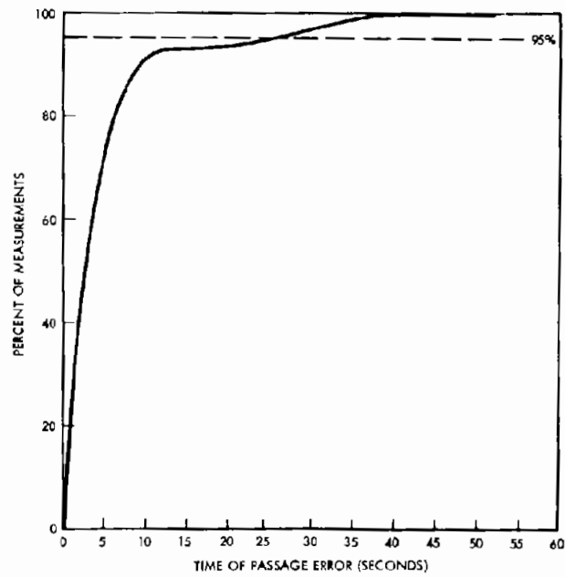
Figure 6-18B. Time of Passage Cumulative Error (No Stop Time Points)
