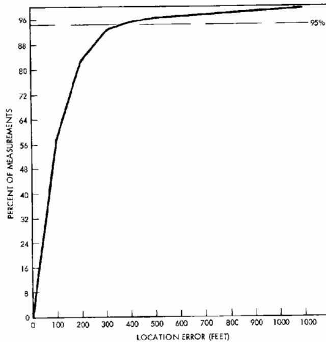
Figure 6-19A. Location Subsystem Histogram (Random Route Tests #20001 - 20005)
