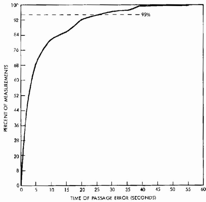
Figure 6-14B. Time of Passage Cumulative Error (Fixed Route Tests #10026 - 10047)
