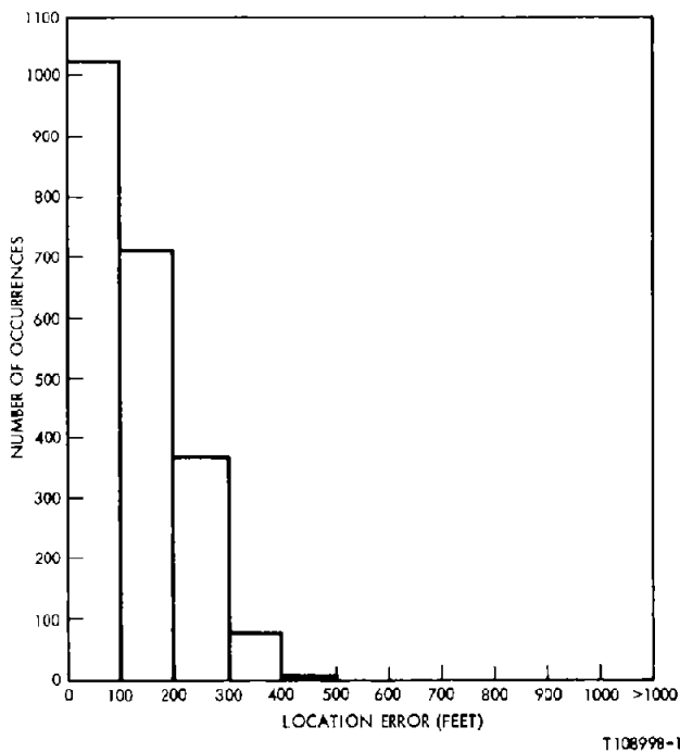
Figure 6-13A. Location Accuracy Histogram (System Simulation) (Fixed Route Tests #10026 - 10047)
