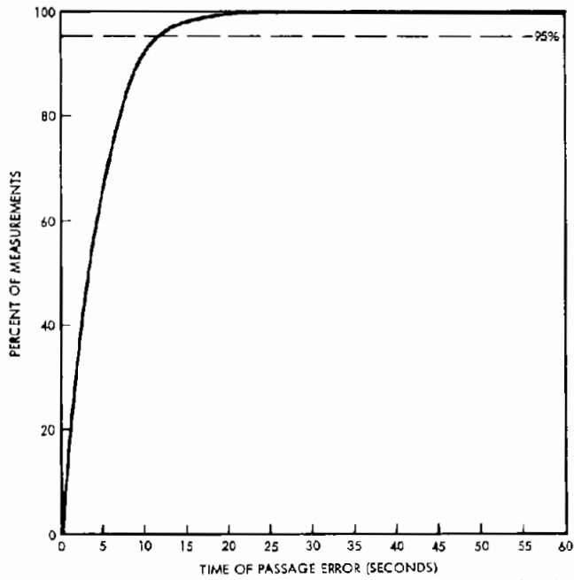
Figure 6-17B. Time of Passage Cumulative Error (All Points - Dead Time Removed)
