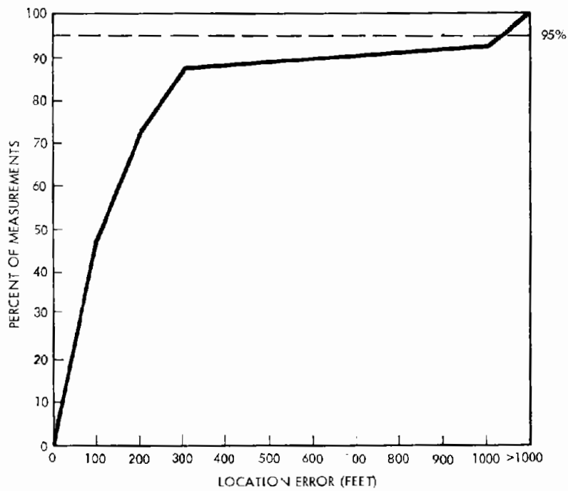
Figure 6-7B. Cumulative Location Error (System Simulation With 5% Missing Data) (Fixed Route Tests #10012 - 10047)
