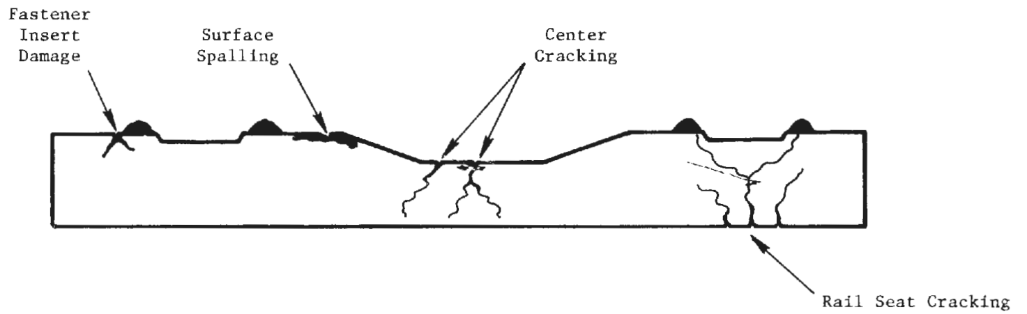
FIGURE 3-1. TYPICAL TIE/FASTENER FAILURE MODES
