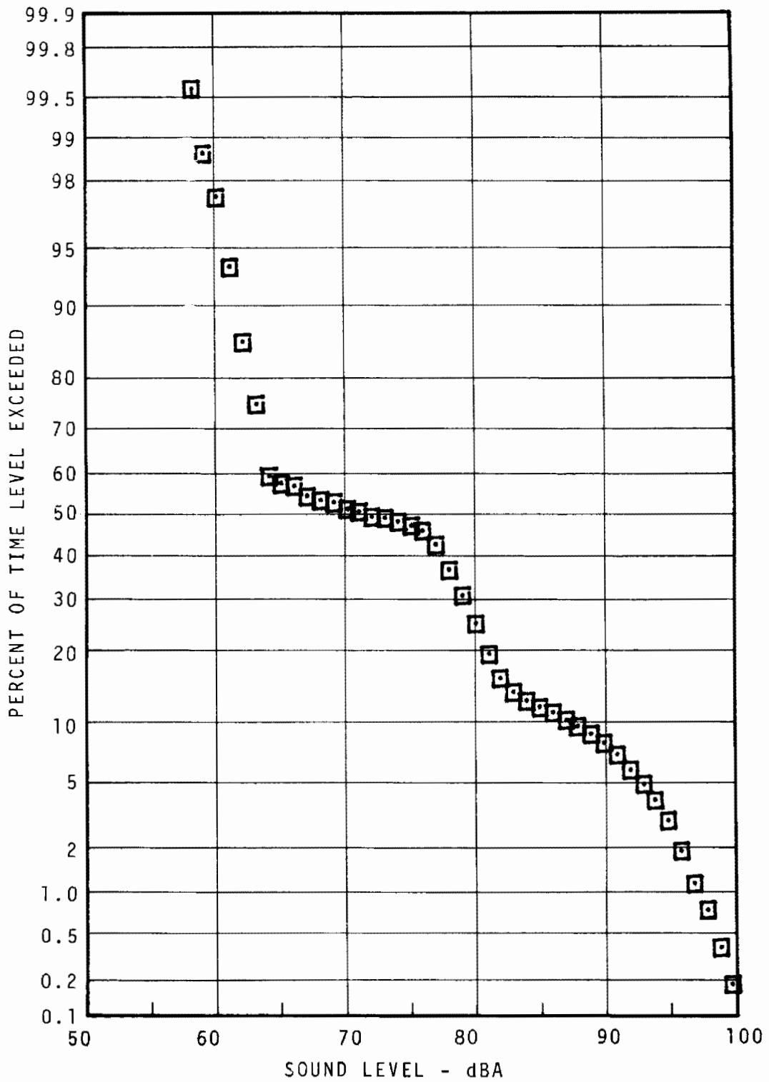
FIGURE 7.69 - 5TH STREET STATION PLATFORM STATISTICAL DISTRIBUTION - DAYTIME
