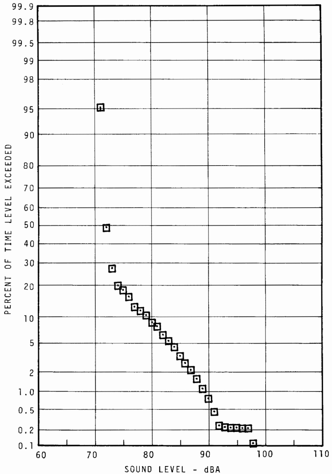
FIGURE 7.82 - YORK-DAUPHIN STATION PLATFORM STATISTICAL DISTRIBUTION - DAYTIME
