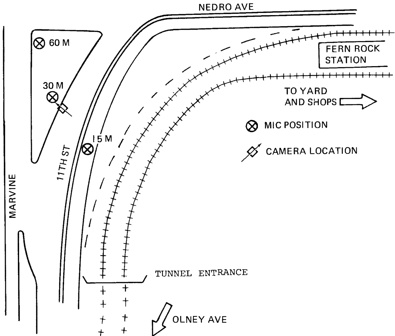
FIGURE 5.13 - WAYSIDE MEASUREMENT LOCATION, 11TH STREET, FERN ROCK
