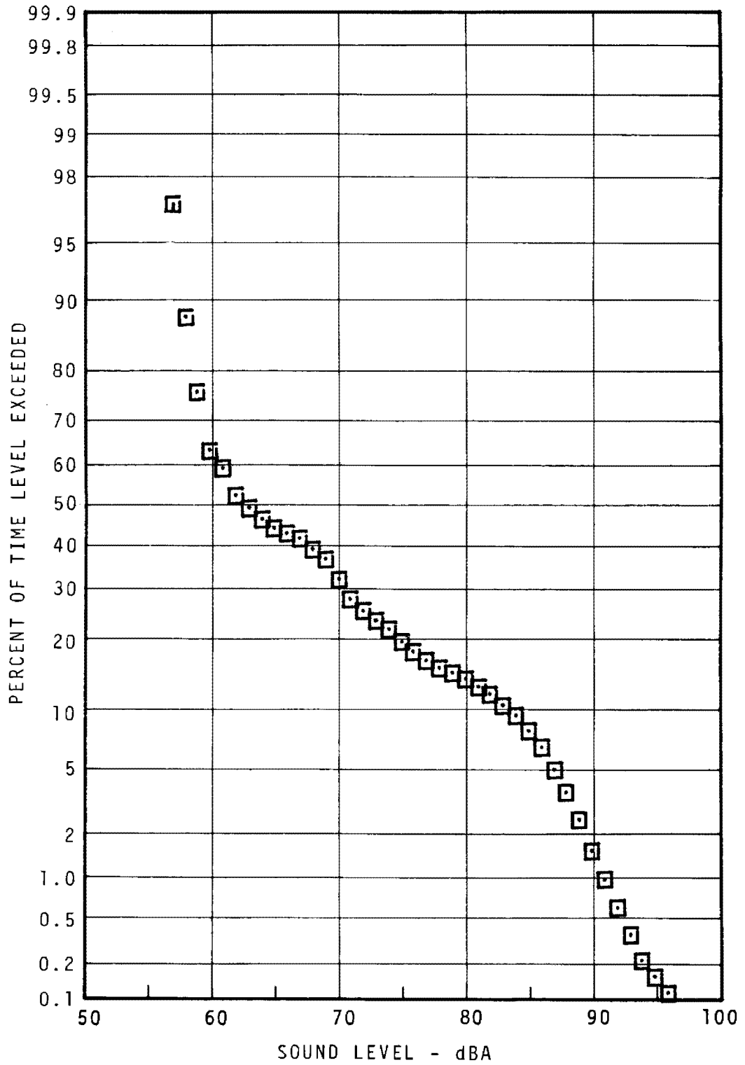
FIGURE 5.62 - PATTISON AVENUE STATION PLATFORM STATISTICAL DISTRIBUTION DAYTIME
