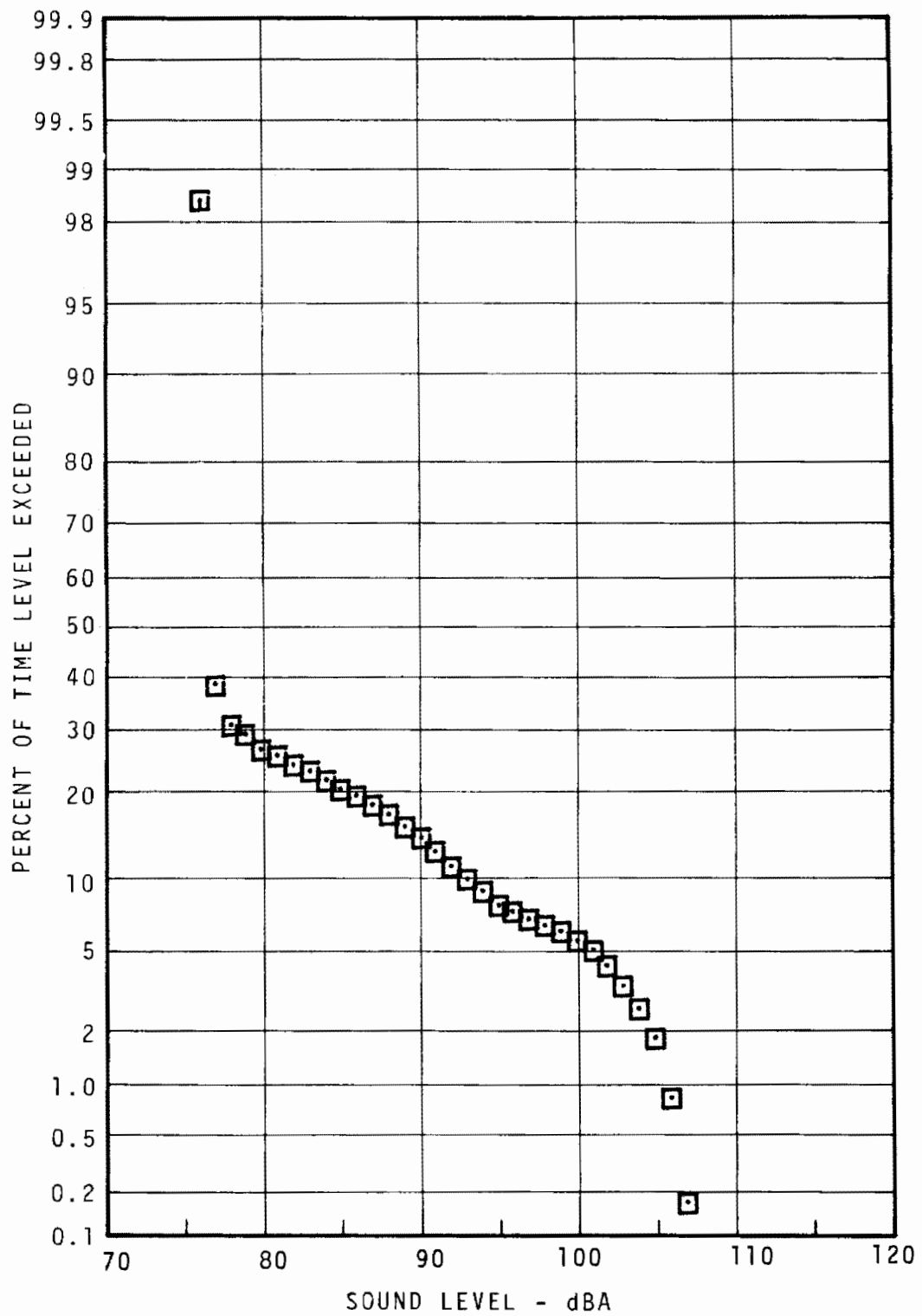
FIGURE 5.33 - SUSQUEHANNA-DAUPHIN STATION PLATFORM STATISTICAL DISTRIBUTION RUSH HOUR
