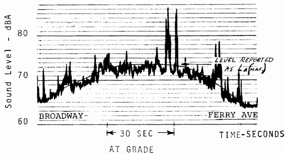
FIGURE 4.4. METHOD OF DETERMINING L_A(\text{Max}) AND T_5
