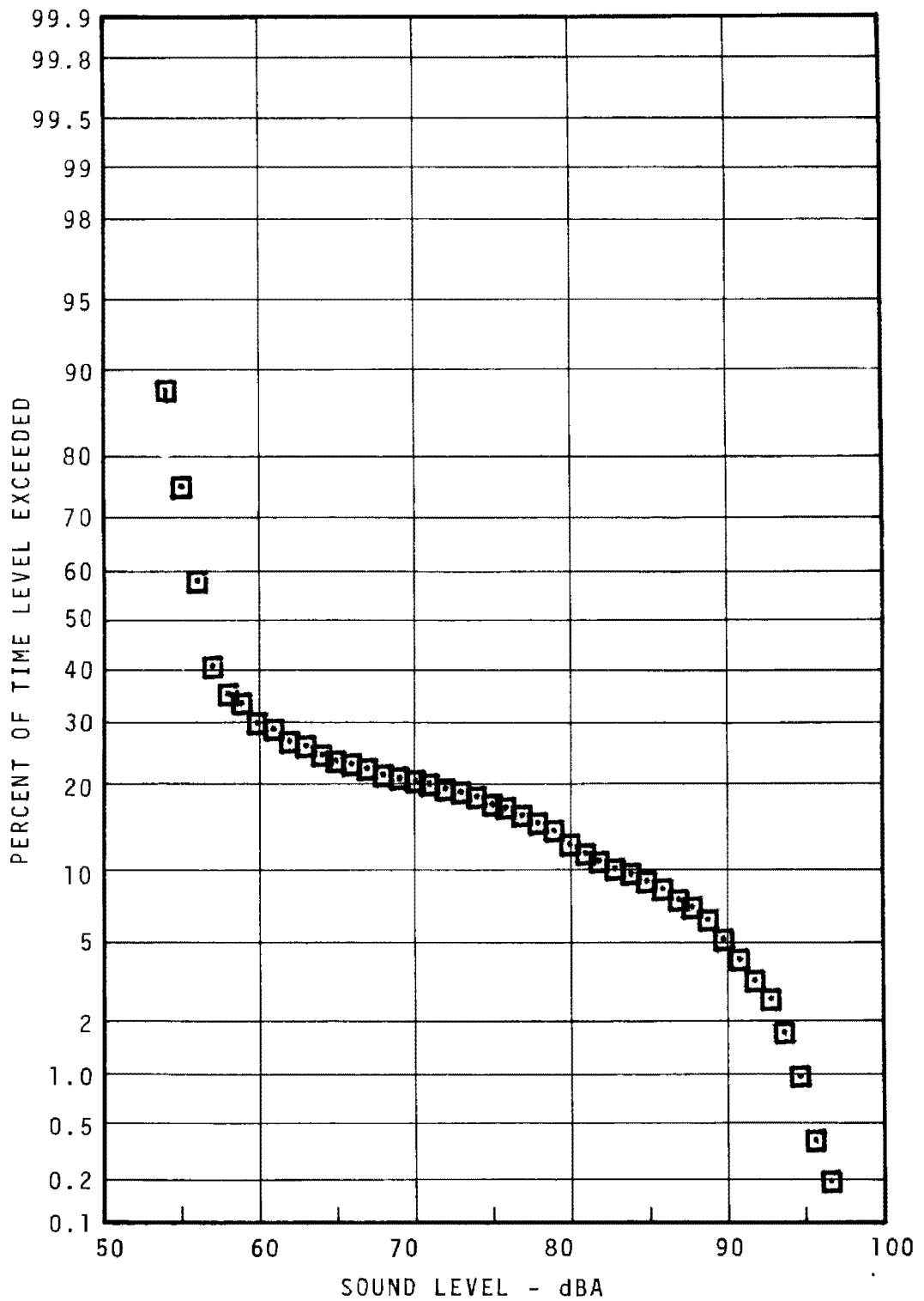
FIGURE 7.71 - 5TH STREET STATION PLATFORM STATISTICAL DISTRIBUTION - EVENING
