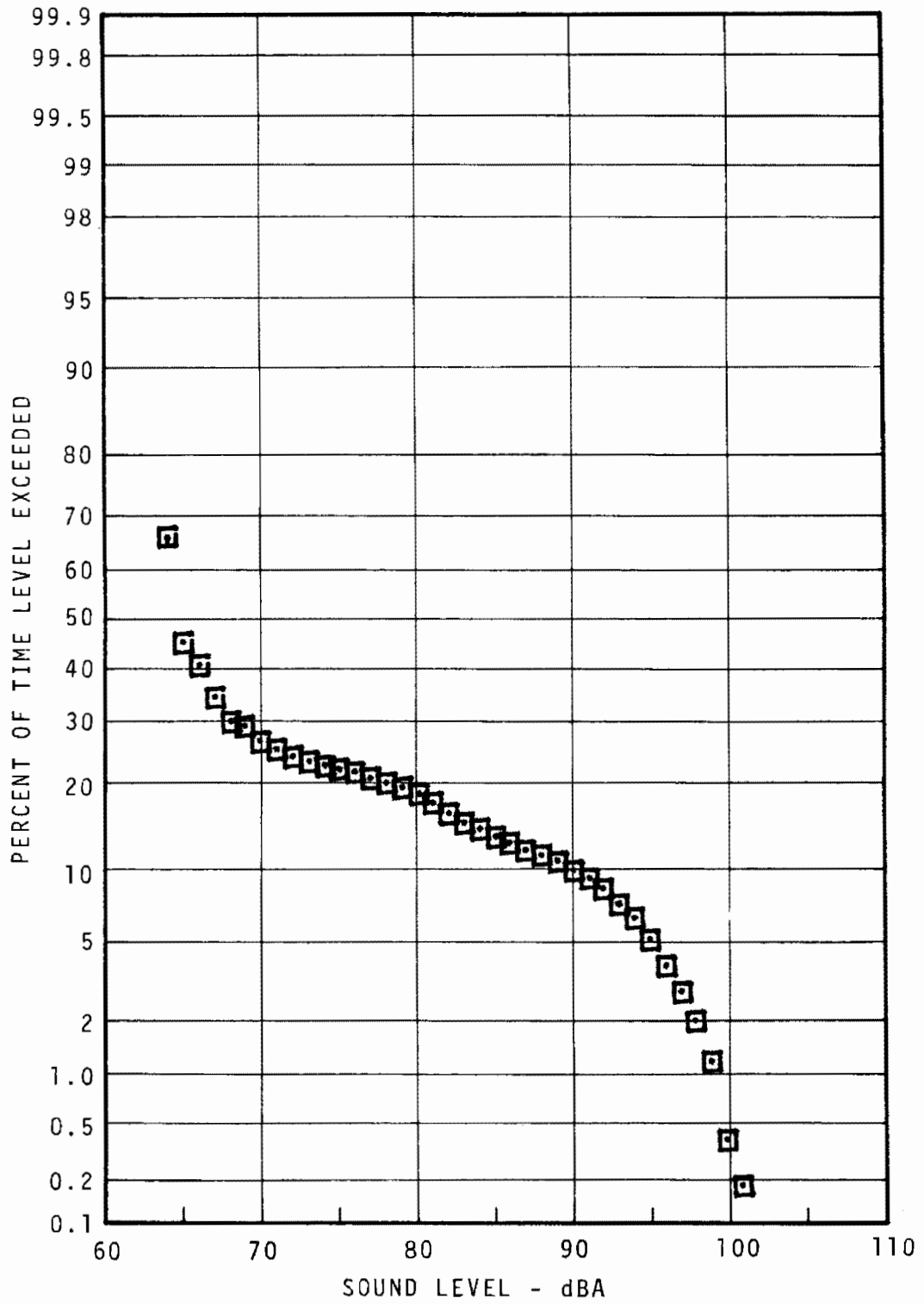
FIGURE 7.60 - 34TH STREET STATION PLATFORM STATISTICAL DISTRIBUTION - DAYTIME
