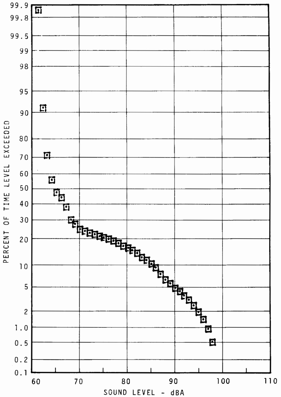
FIGURE 7.75 - 2ND STREET STATION PLATFORM STATISTICAL DISTRIBUTION - DAYTIME
