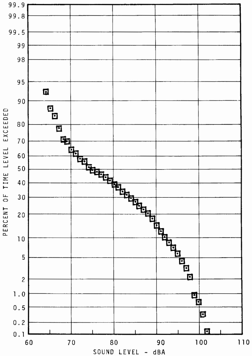
FIGURE 7.63 - 30TH STREET STATION PLATFORM STATISTICAL DISTRIBUTION - DAYTIME
