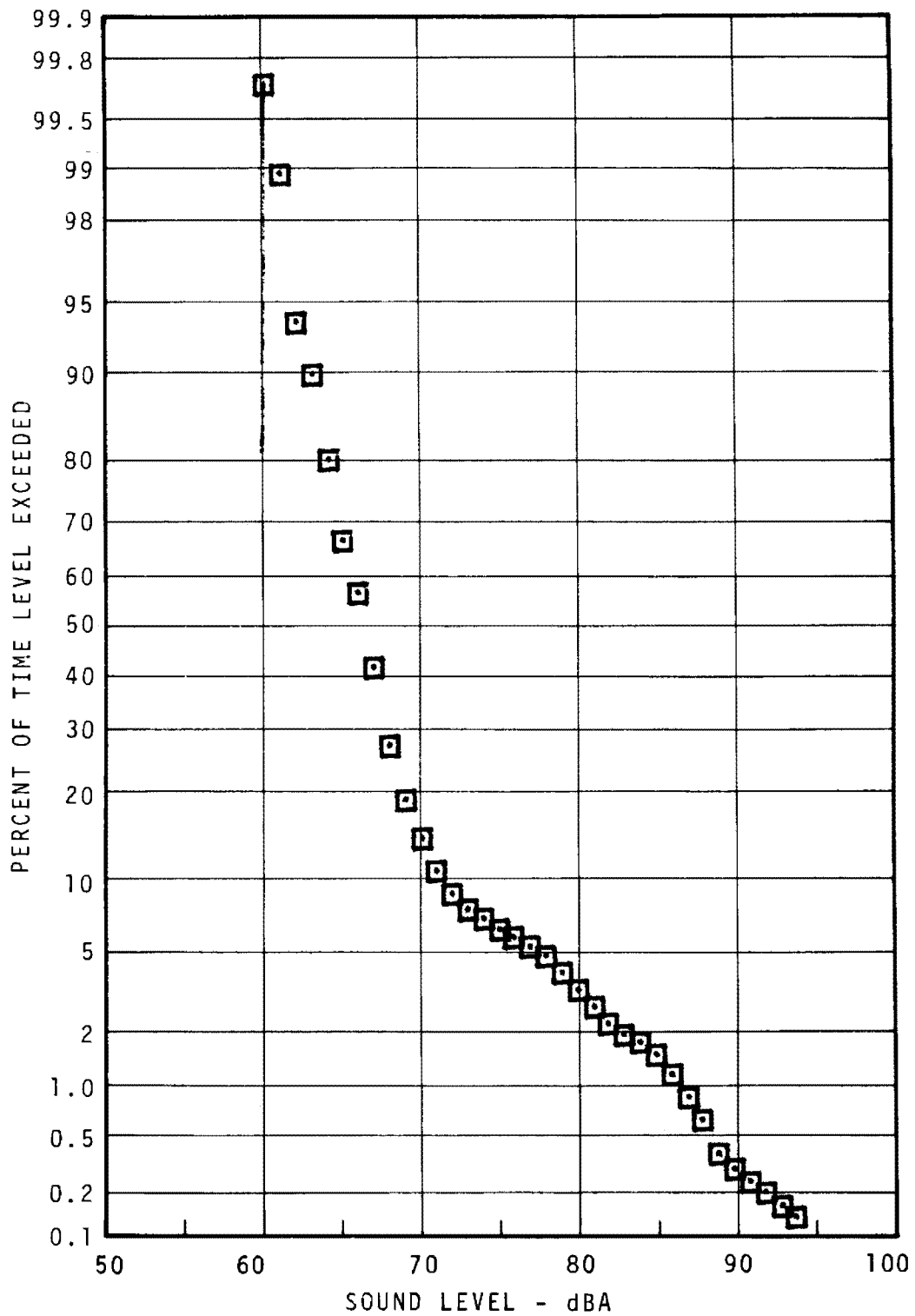
FIGURE 7.91 - BRIDGE STREET STATION PLATFORM STATISTICAL DISTRIBUTION - EVENING
