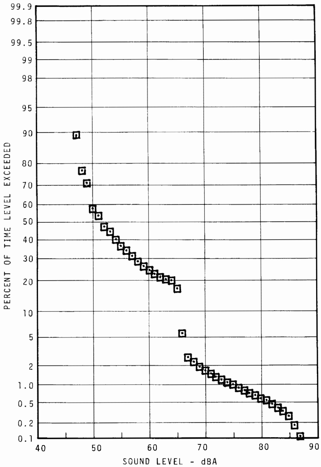
FIGURE 5.9 - 10th AND NEDRO, FERN ROCK COMMUNITY STATISTICAL DISTRIBUTION - 25M - NIGHT
