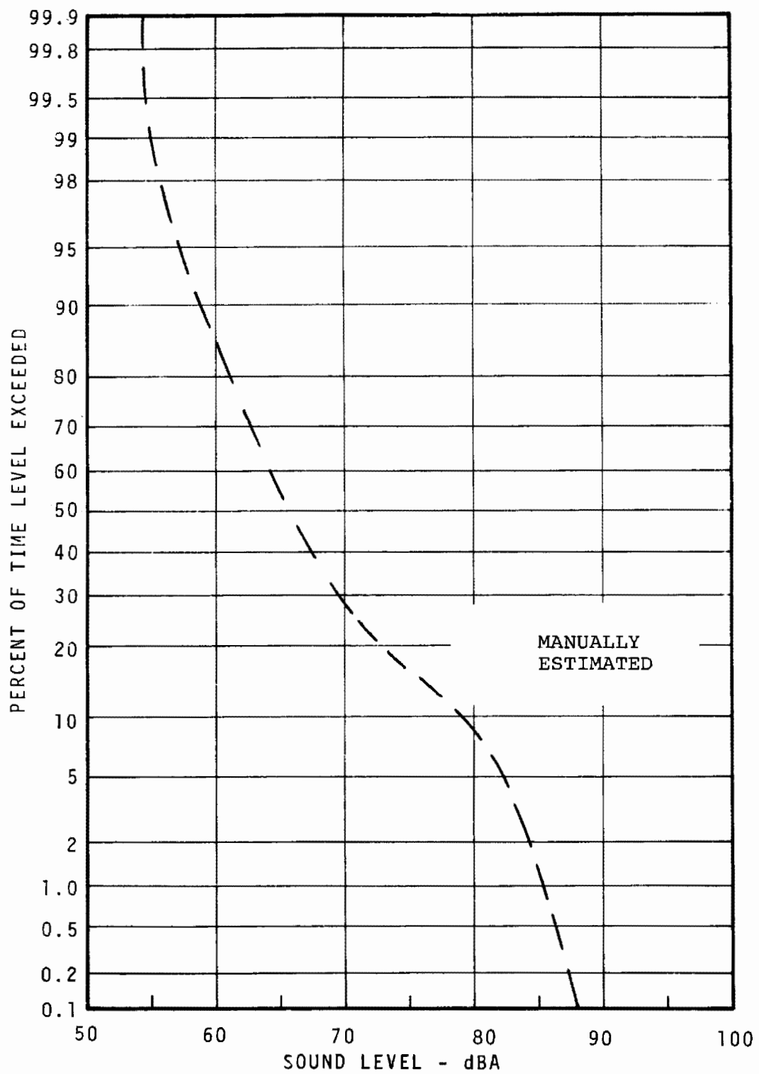
FIGURE 7.33 - SOMERSET COMMUNITY STATISTICAL DISTRIBUTION - 15M - DAYTIME
