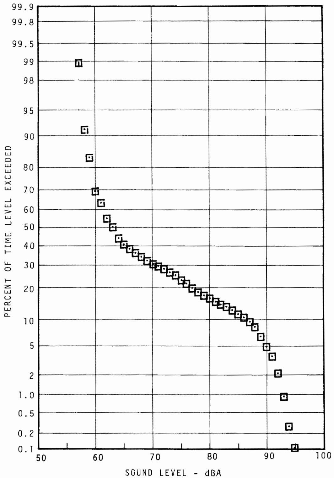
FIGURE 5.59 -SNYDER AVENUE STATION PLATFORM STATISTICAL DISTRIBUTION DAYTIME
