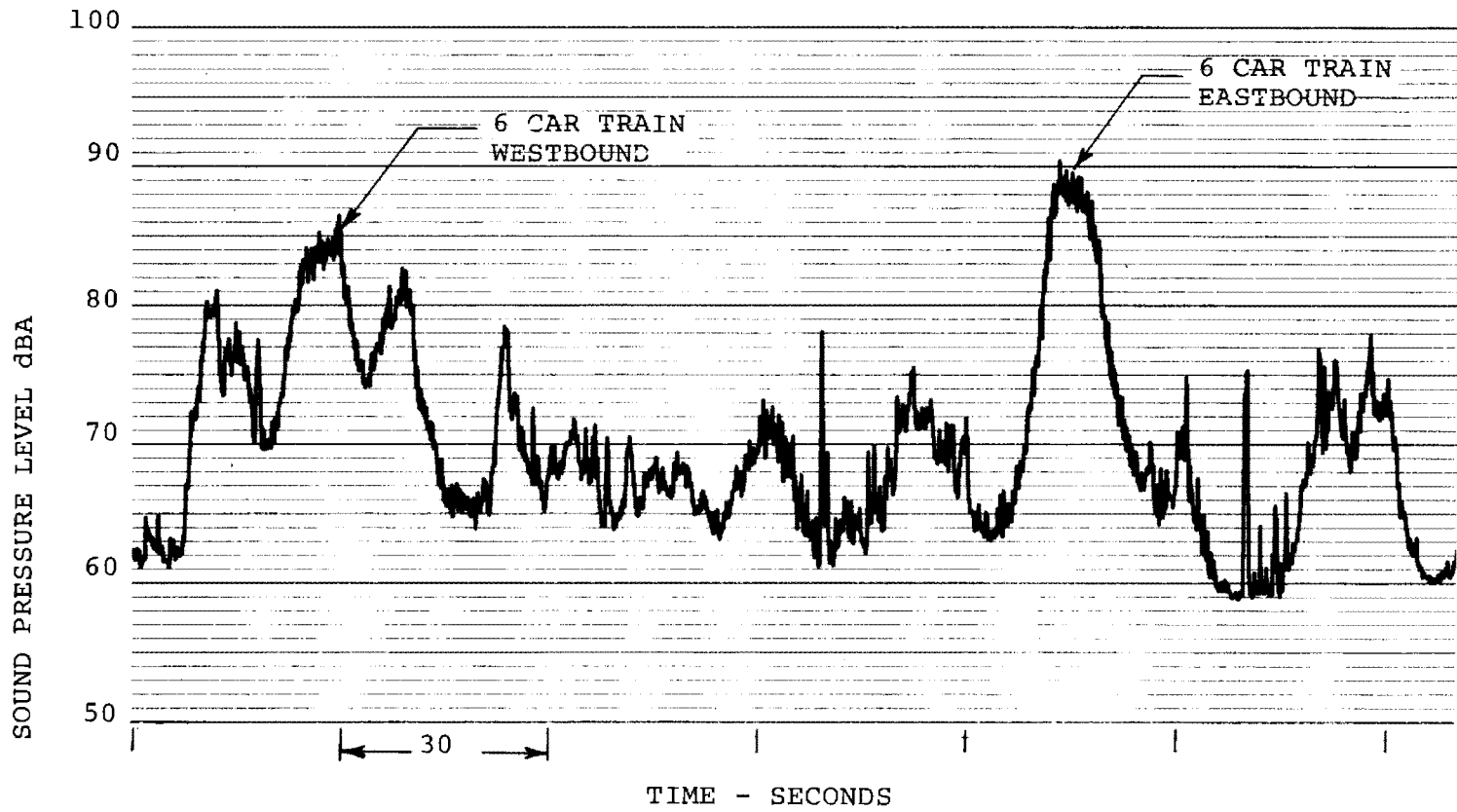
FIGURE 7.23 - TYPICAL NOISE TIMEHISTORY, 54TH AND MARKET COMMUNITY, 15M.
