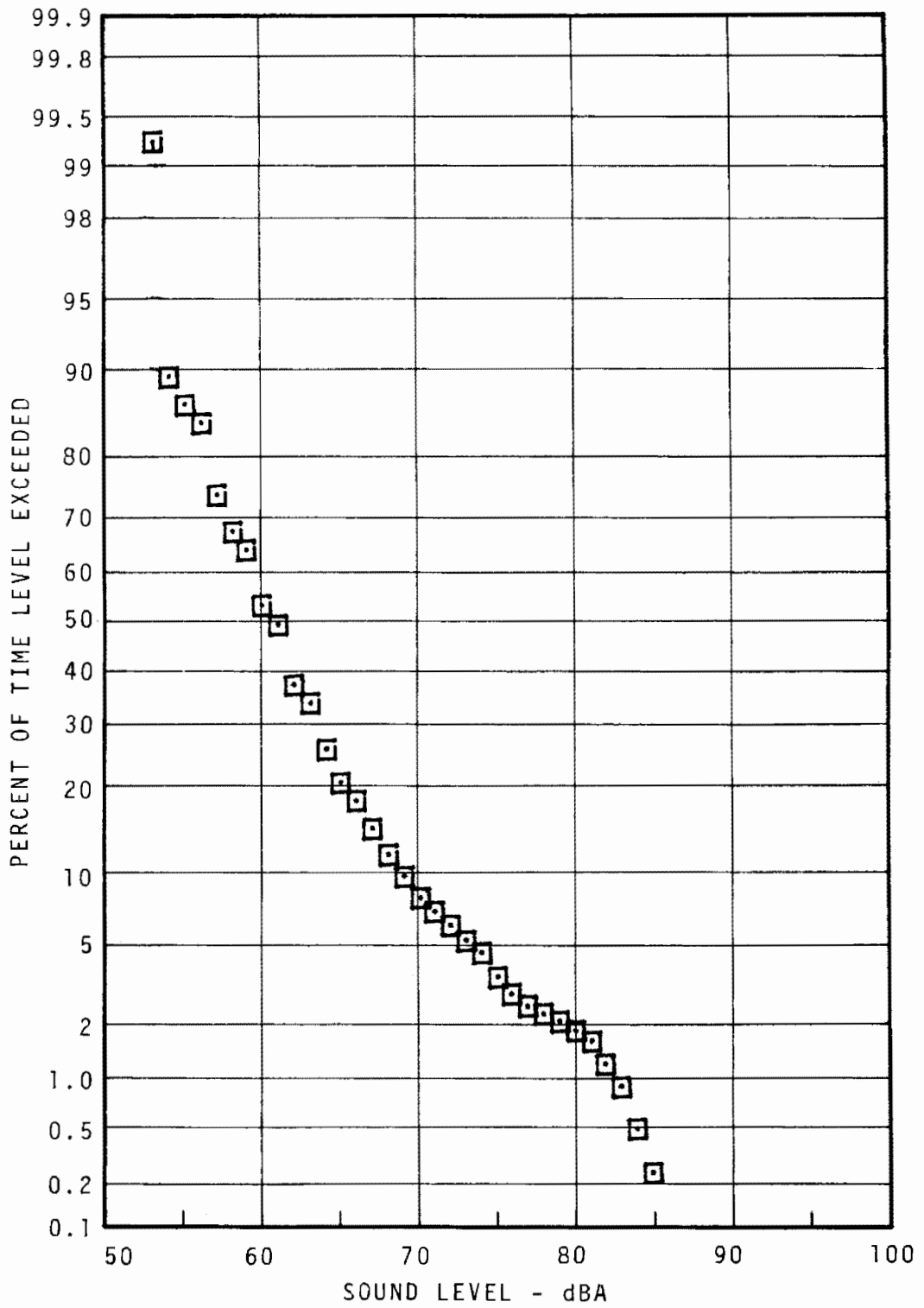
FIGURE 7.35 - SOMERSET COMMUNITY STATISTICAL DISTRIBUTION - 15M - EVENING
