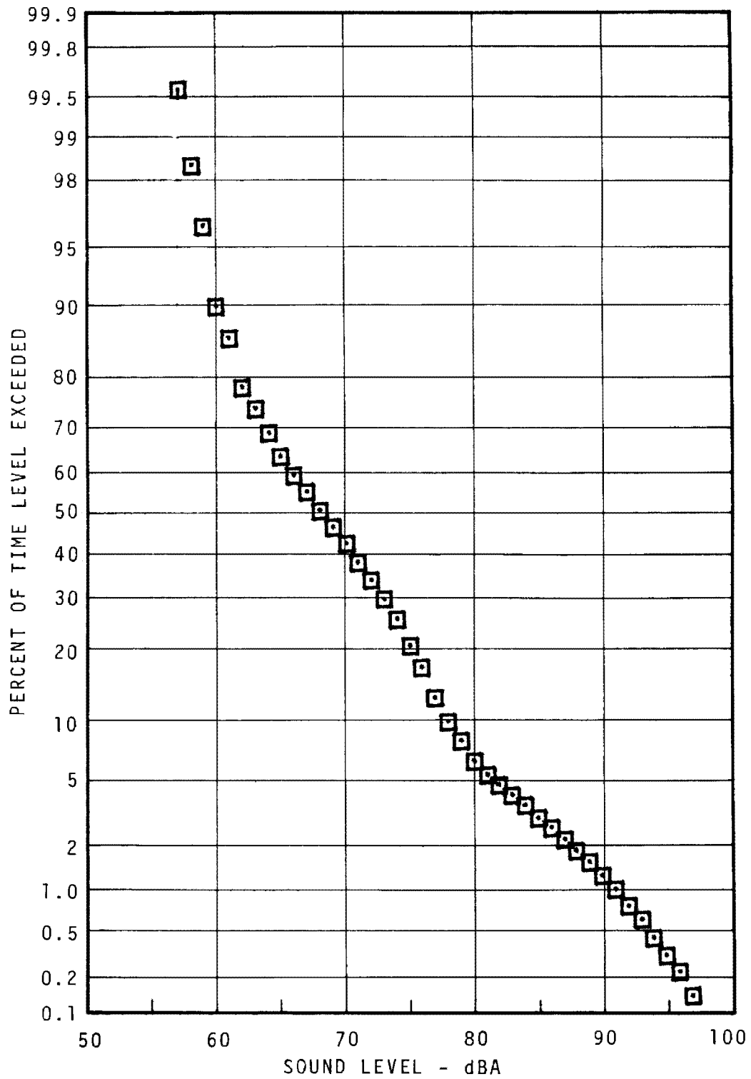
FIGURE 7.4 - 69TH ST. COMMUNITY STATISTICAL DISTRIBUTION - 15M - DAYTIME
