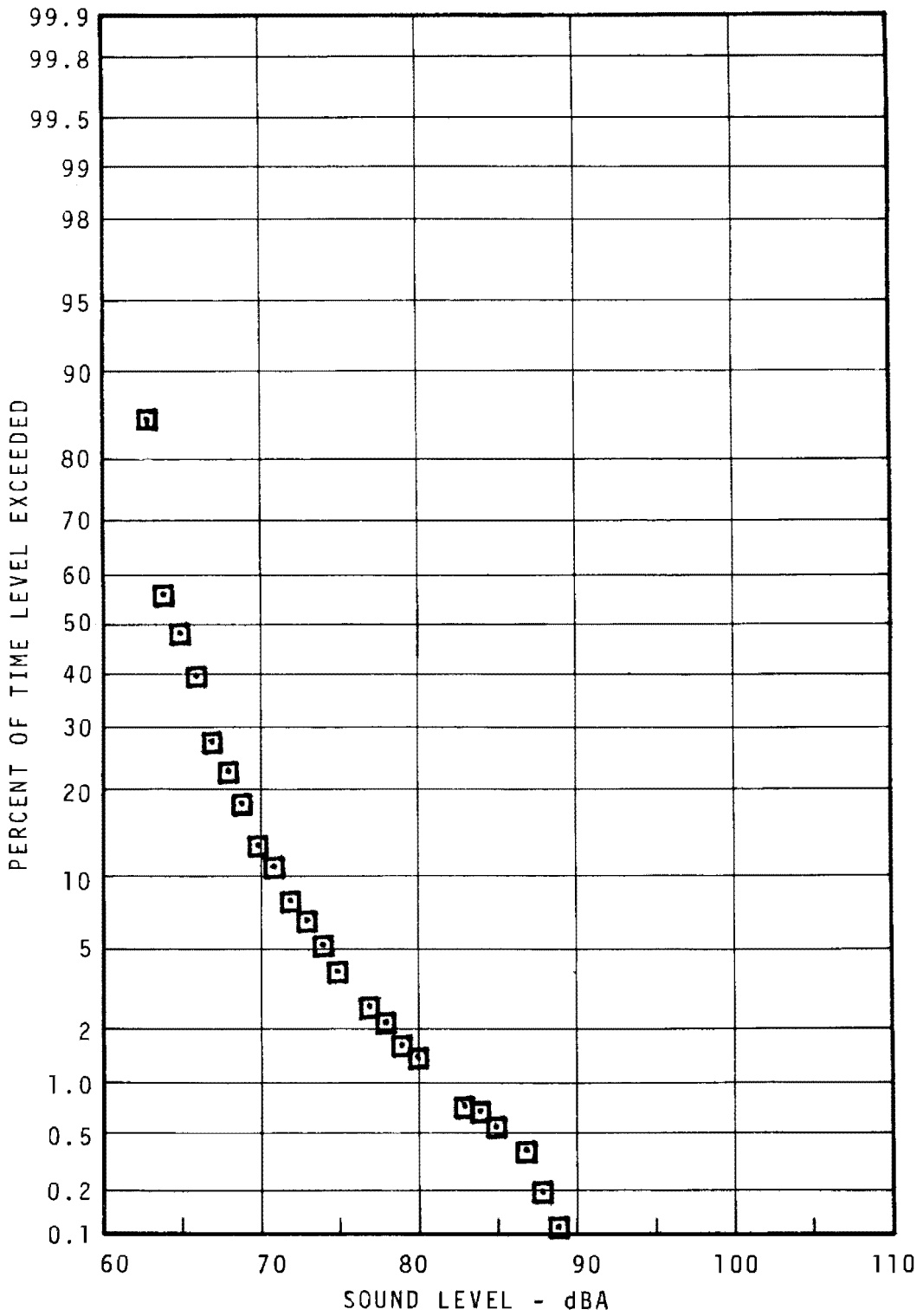
FIGURE 7.30 - YORK-DAUPHIN COMMUNITY STATISTICAL DISTRIBUTION - 120M - DAYTIME
