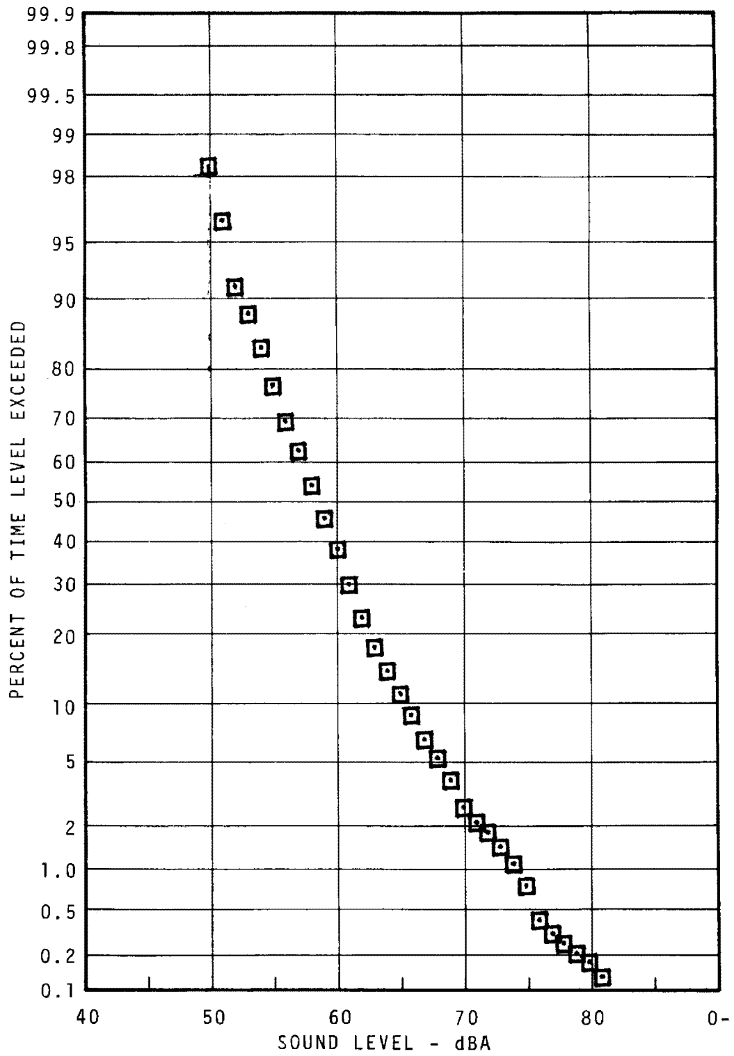
FIGURE 7.15 - MILLBOURNE COMMUNITY STATISTICAL DISTRIBUTION - 60M - DAYTIME
