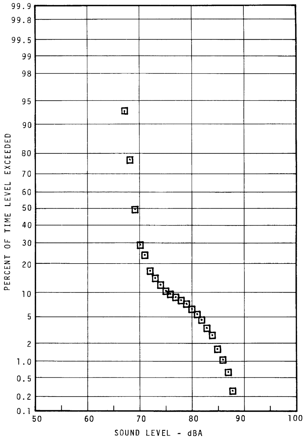
FIGURE 7.51 - 52ND STREET STATION PLATFORM STATISTICAL DISTRIBUTION - DAYTIME
