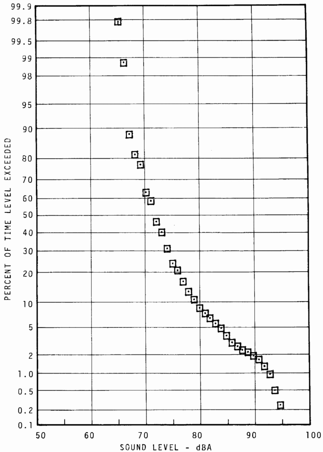
FIGURE 7.27 - YORK-DAUPHIN COMMUNITY STATISTICAL DISTRIBUTION - 15M - EVENING
