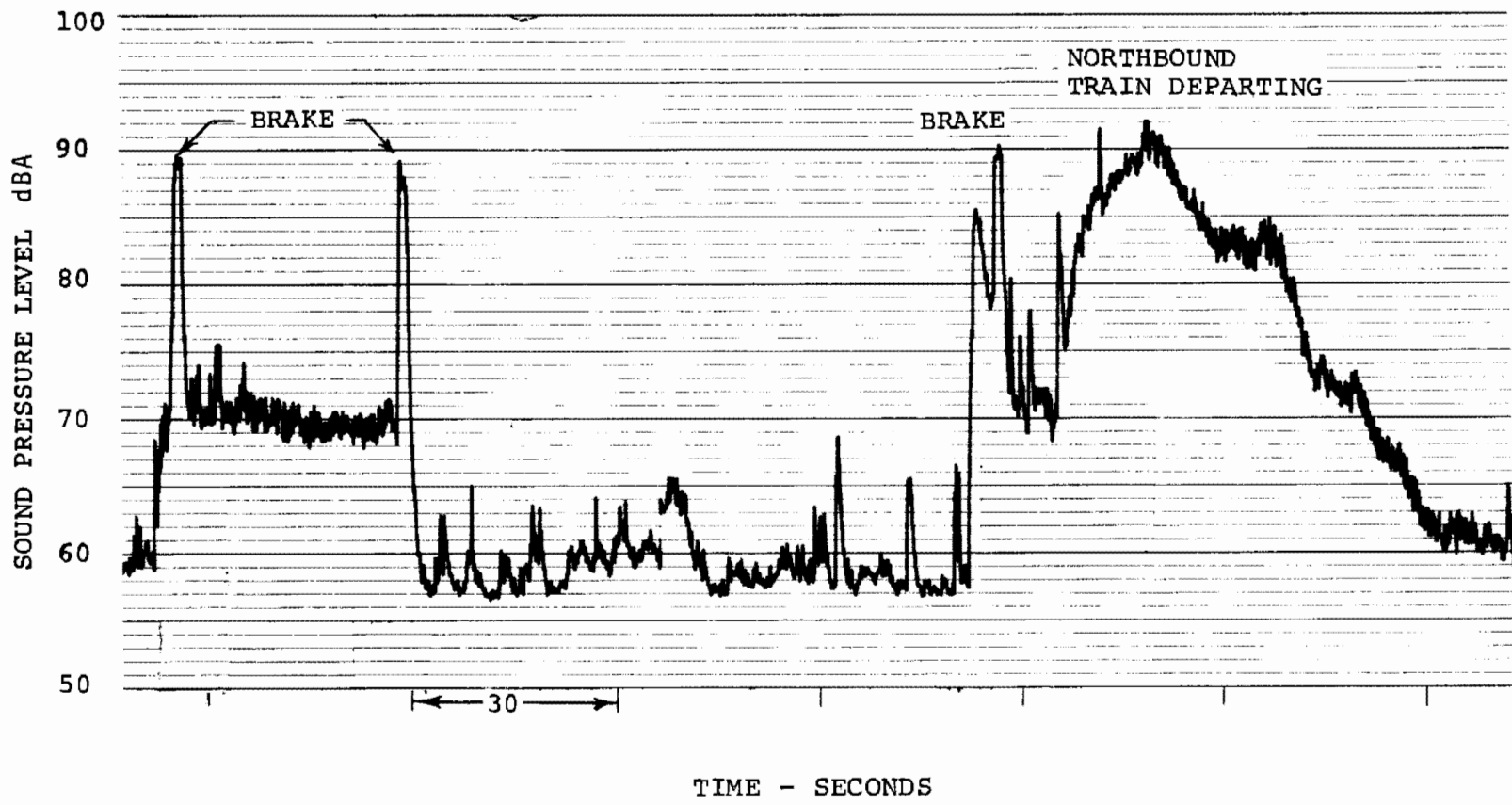
FIGURE 5.66 - TYPICAL TIME HISTORY, PATTISON AVE. STATION
