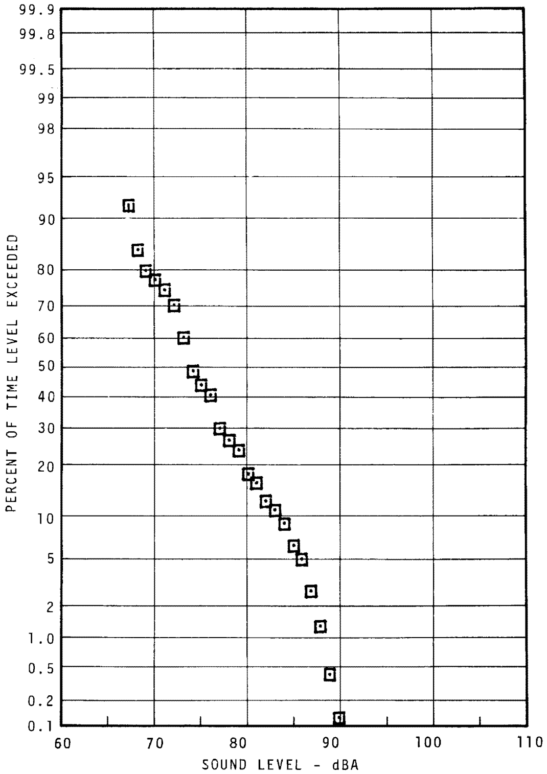
FIGURE 7.98 - 1960 BUDD IN-CAR (OPERATOR BOOTH) STATISTICAL DISTRIBUTION - BRIDGE STREET TO 69TH STREET
