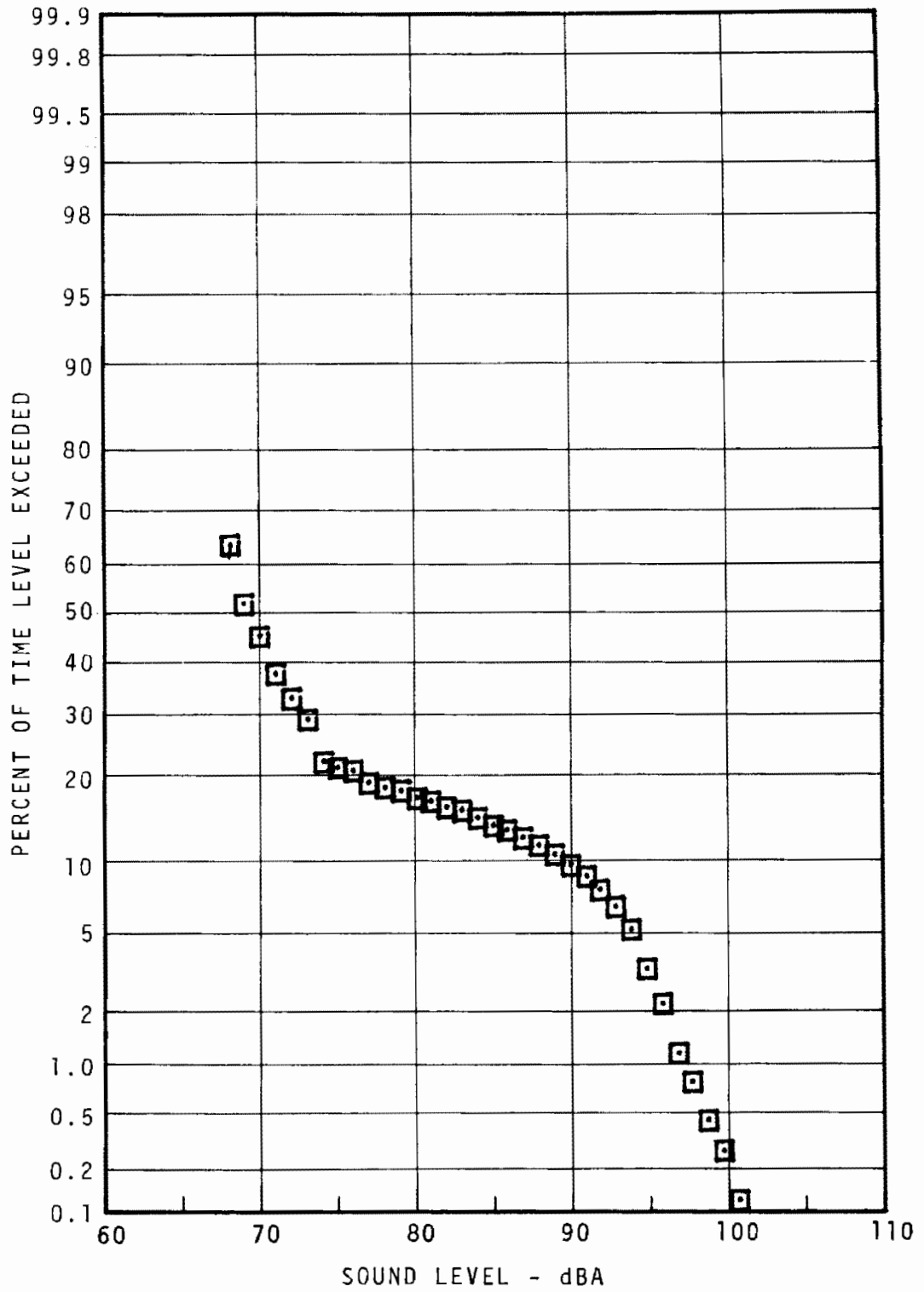
FIGURE 5.32. - SUSQUEHANNA-DAUPHIN STATION PLATFORM STATISTICAL DISTRIBUTION DAYTIME
