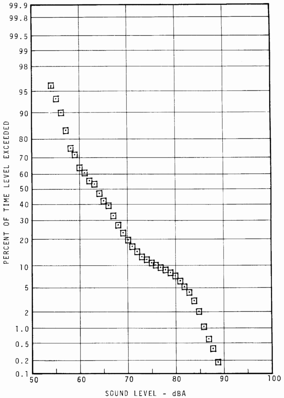
FIGURE 5.26 - FERN ROCK STATION PLATFORM STATISTICAL DISTRIBUTION DAYTIME
