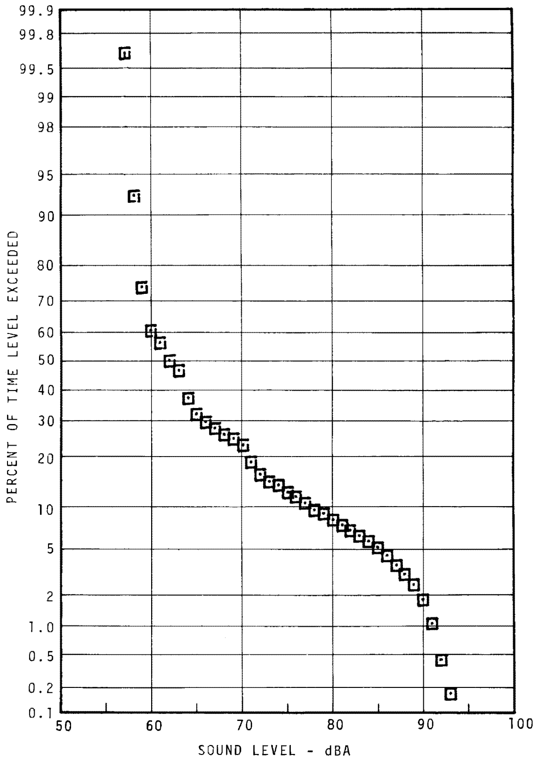
FIGURE 5.64 - PATTISON AVENUE STATION PLATFORM STATISTICAL DISTRIBUTION EVENING
