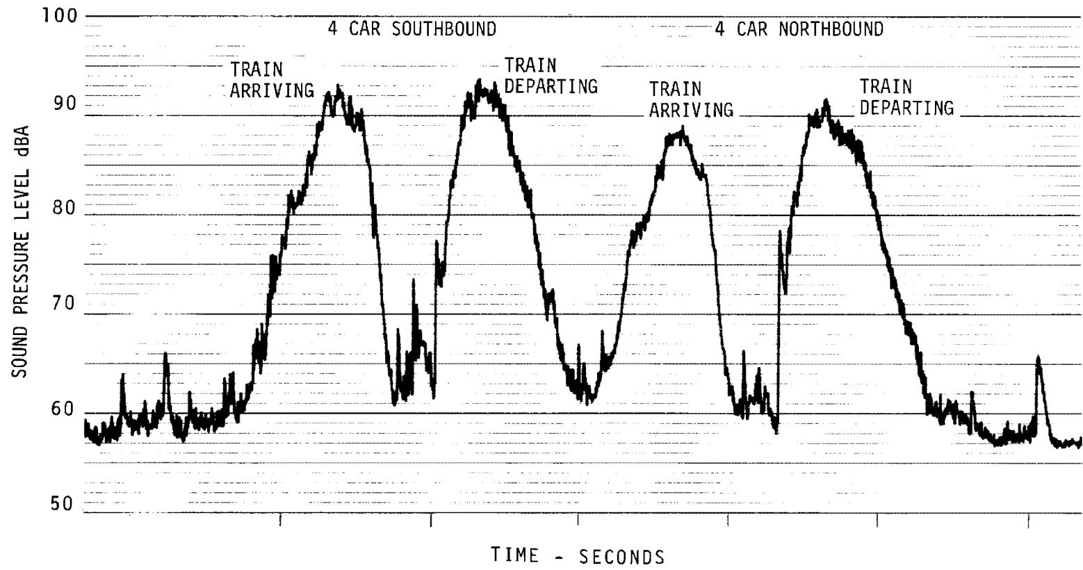
FIGURE 5.40 - TYPICAL TIME HISTORY, SPRING GARDEN STATION (BROAD) LOCAL TRACK
