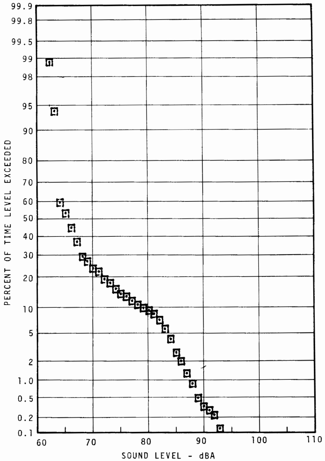
FIGURE 7.78 - BERKS STATION PLATFORM STATISTICAL DISTRIBUTION - DAYTIME
