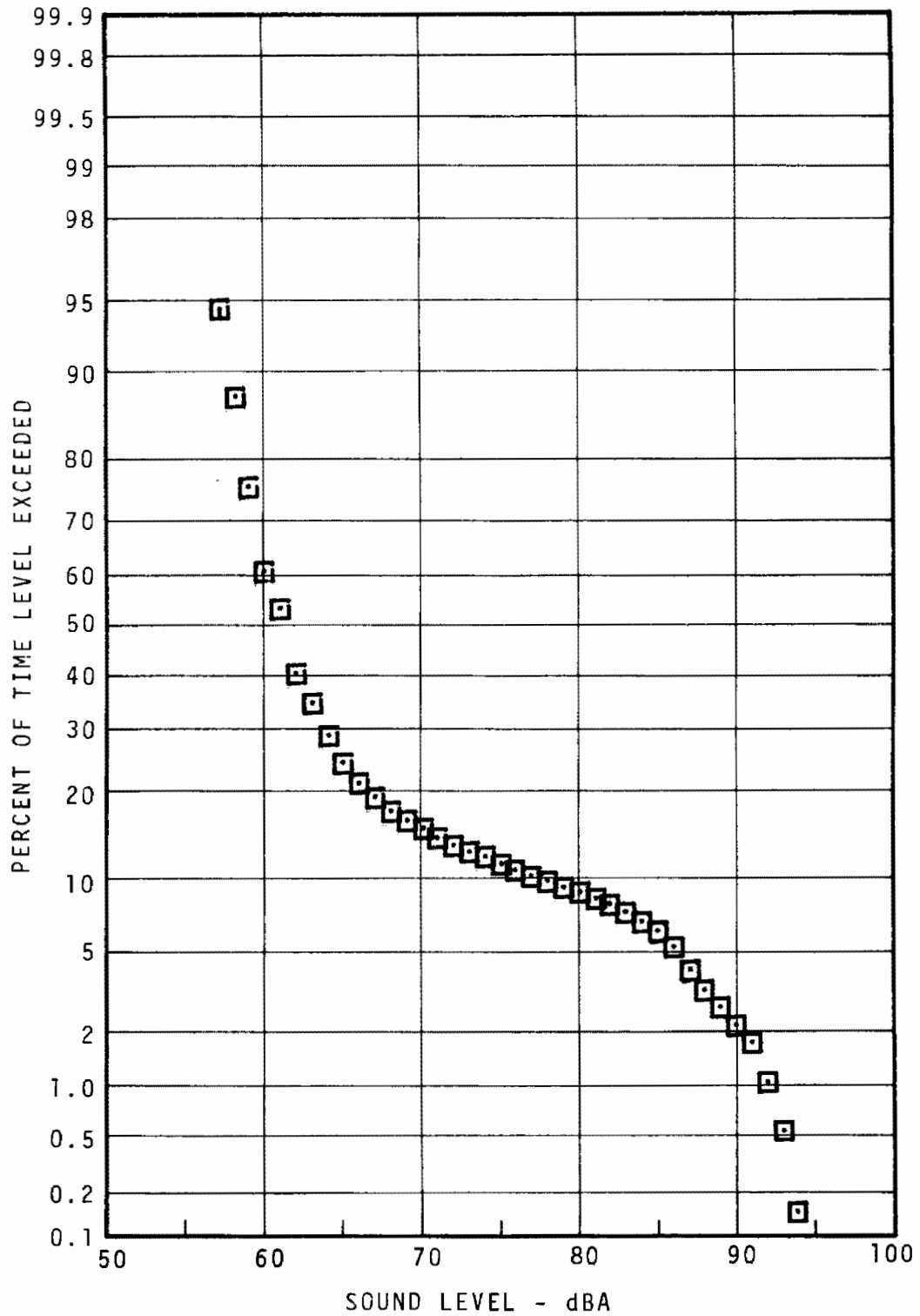
FIGURE 5.55 - WALNUT-LOCUST STATION PLATFORM STATISTICAL DISTRIBUTION EVENING
