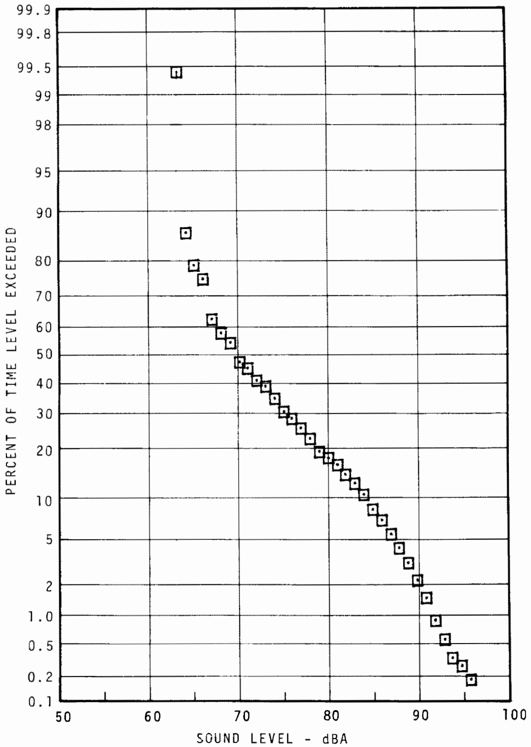
FIGURE 5.56 - WALNUT-LOCUST STATION PLATFORM STATISTICAL DISTRIBUTION NIGHT
