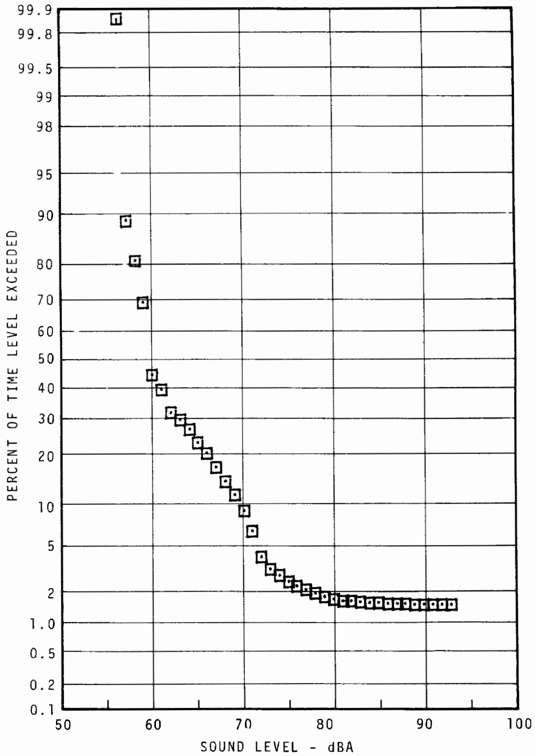
FIGURE 7.83 - YORK-DAUPHIN STATION PLATFORM STATISTICAL DISTRIBUTION - NIGHT
