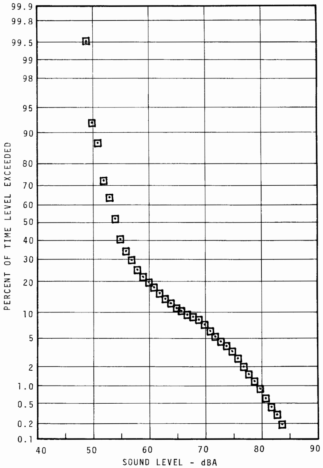
FIGURE 7.10 - MILLBOURNE COMMUNITY STATISTICAL DISTRIBUTION - 15M - DAYTIME
