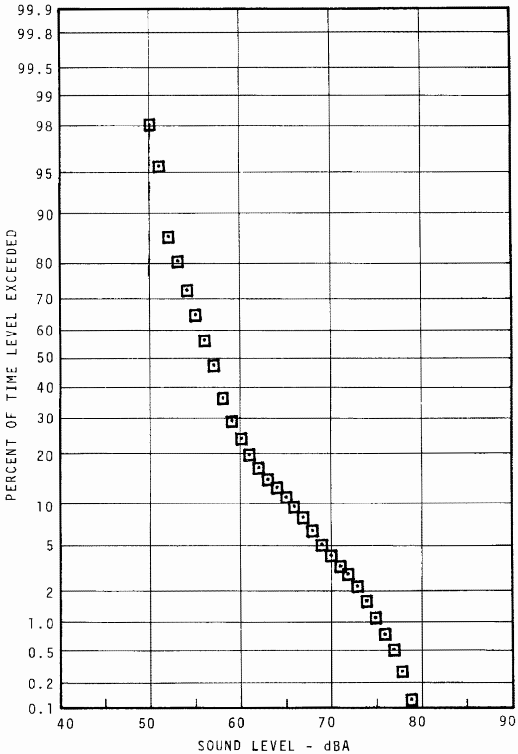
FIGURE 7.14 - MILLBOURNE COMMUNITY STATISTICAL DISTRIBUTION - 30M - DAYTIME
