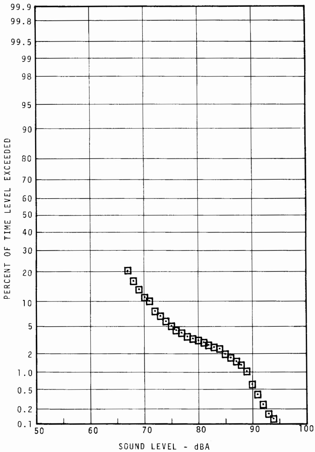
FIGURE 5.50 - CITY HALL STATION PLATFORM STATISTICAL DISTRIBUTION NIGHT
