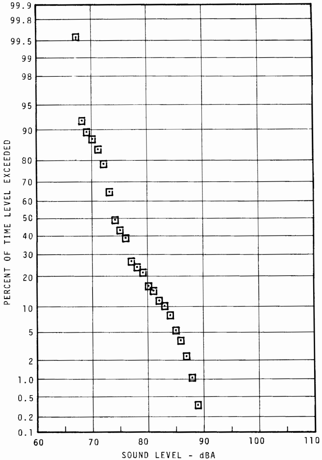
FIGURE 7.97 - 1960 BUDD IN-CAR (CENTER) STATISTICAL DISTRIBUTION BRIDGE STREET TO 69TH STREET
