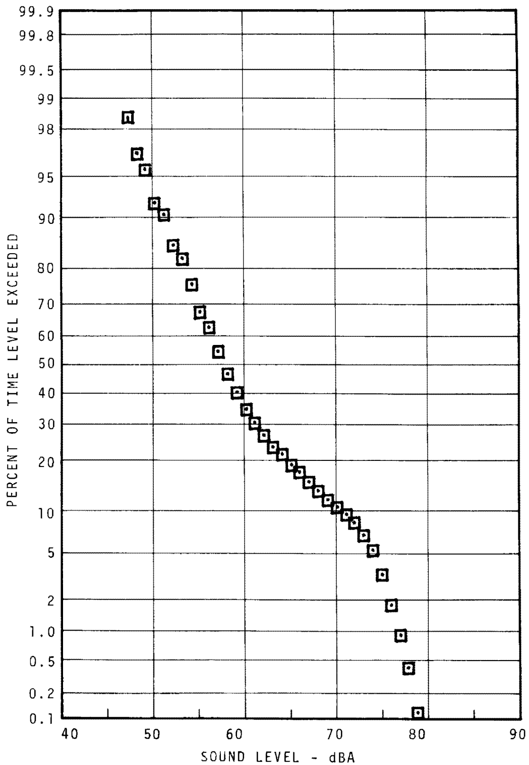
FIGURE 7.34 - SOMERSET COMMUNITY STATISTICAL DISTRIBUTION - 15M - RUSH HOUR
