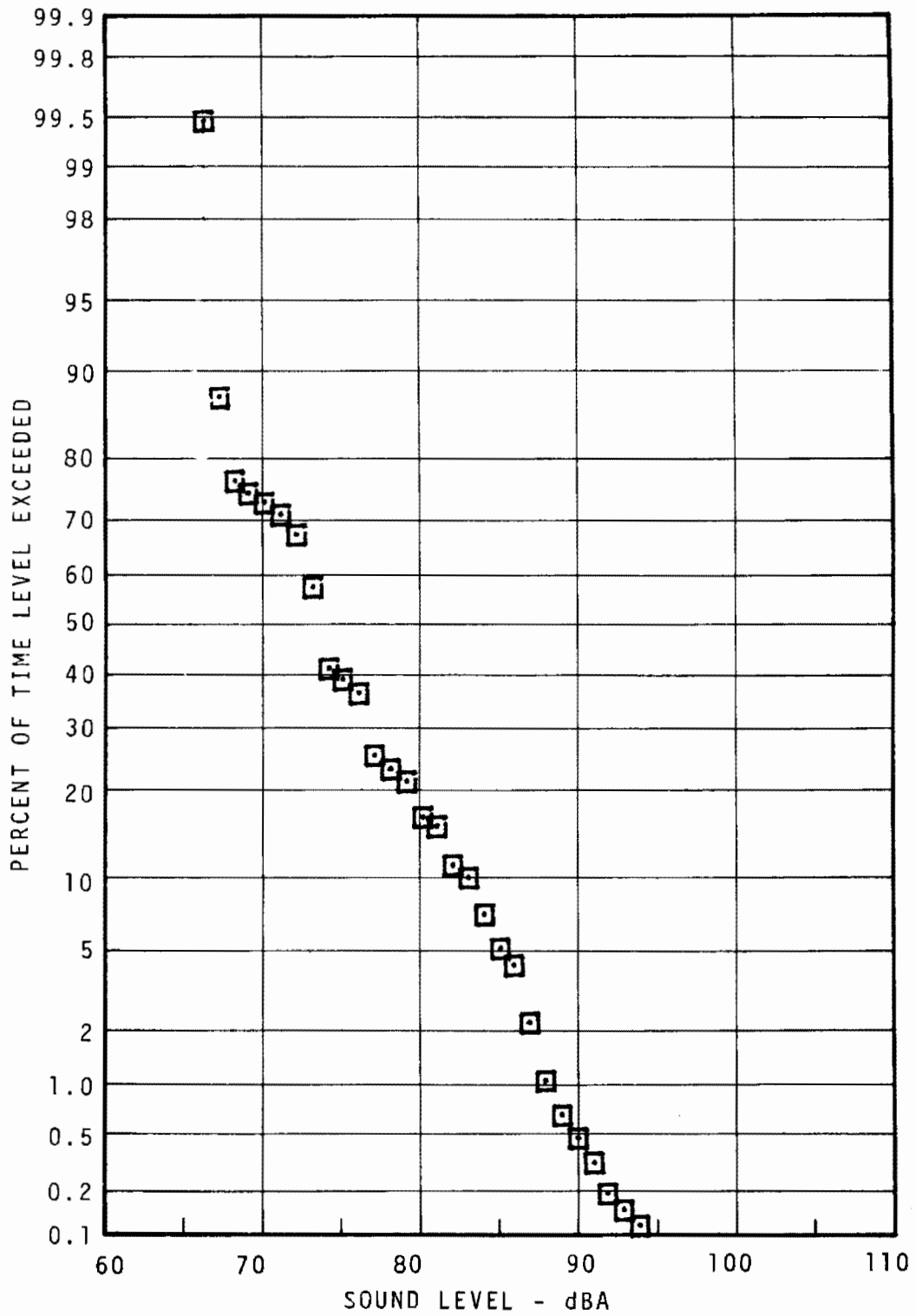
FIGURE 7.96 - 1960 BUDD IN-CAR (OPERATOR BOOTH) STATISTICAL DISTRIBUTION - 69TH STREET TO BRIDGE ST.
