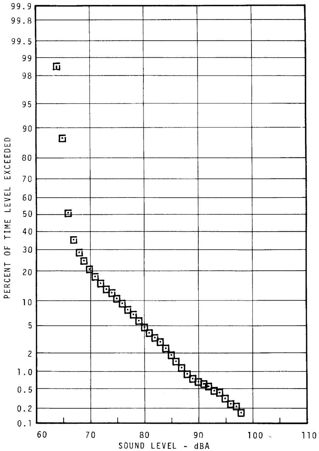
FIGURE 7.7- 69TH ST. COMMUNITY STATISTICAL DISTRIBUTION - 15M - NIGHT
