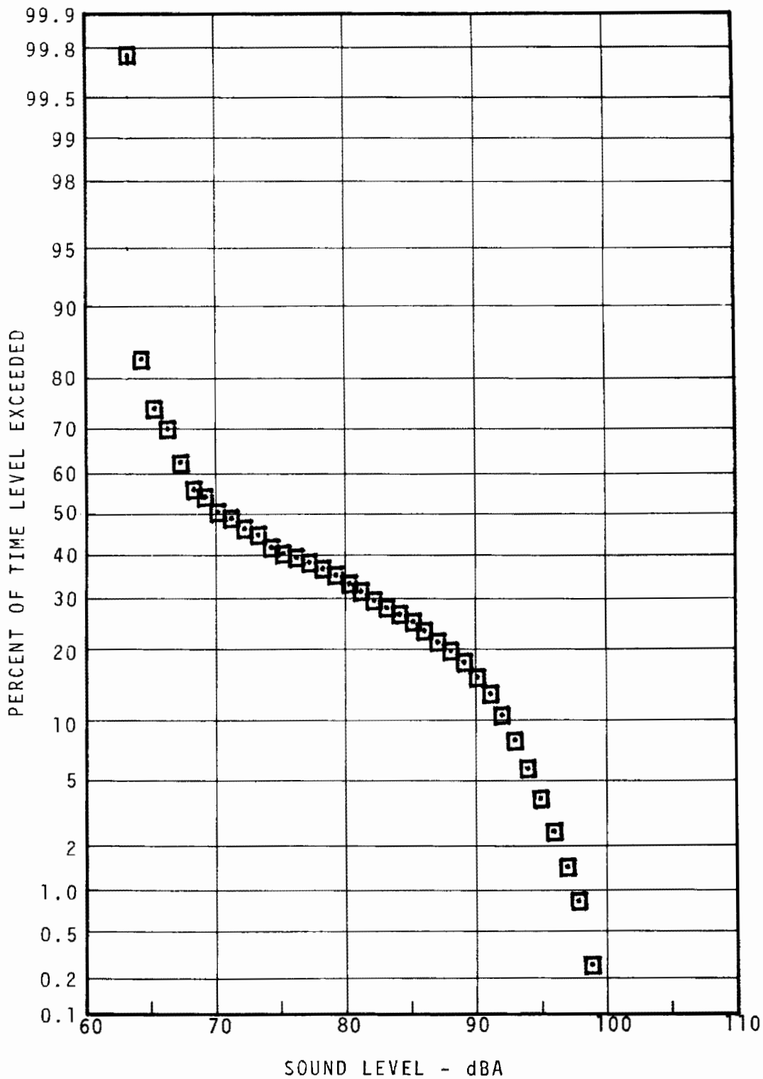
FIGURE 5.54 - WALNUT-LOCUST STATION PLATFORM STATISTICAL DISTRIBUTION RUSH HOUR
