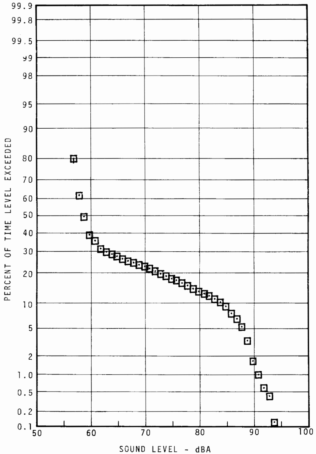
FIGURE 5.53 - WALNUT-LOCUST STATION PLATFORM STATISTICAL DISTRIBUTION DAYTIME
