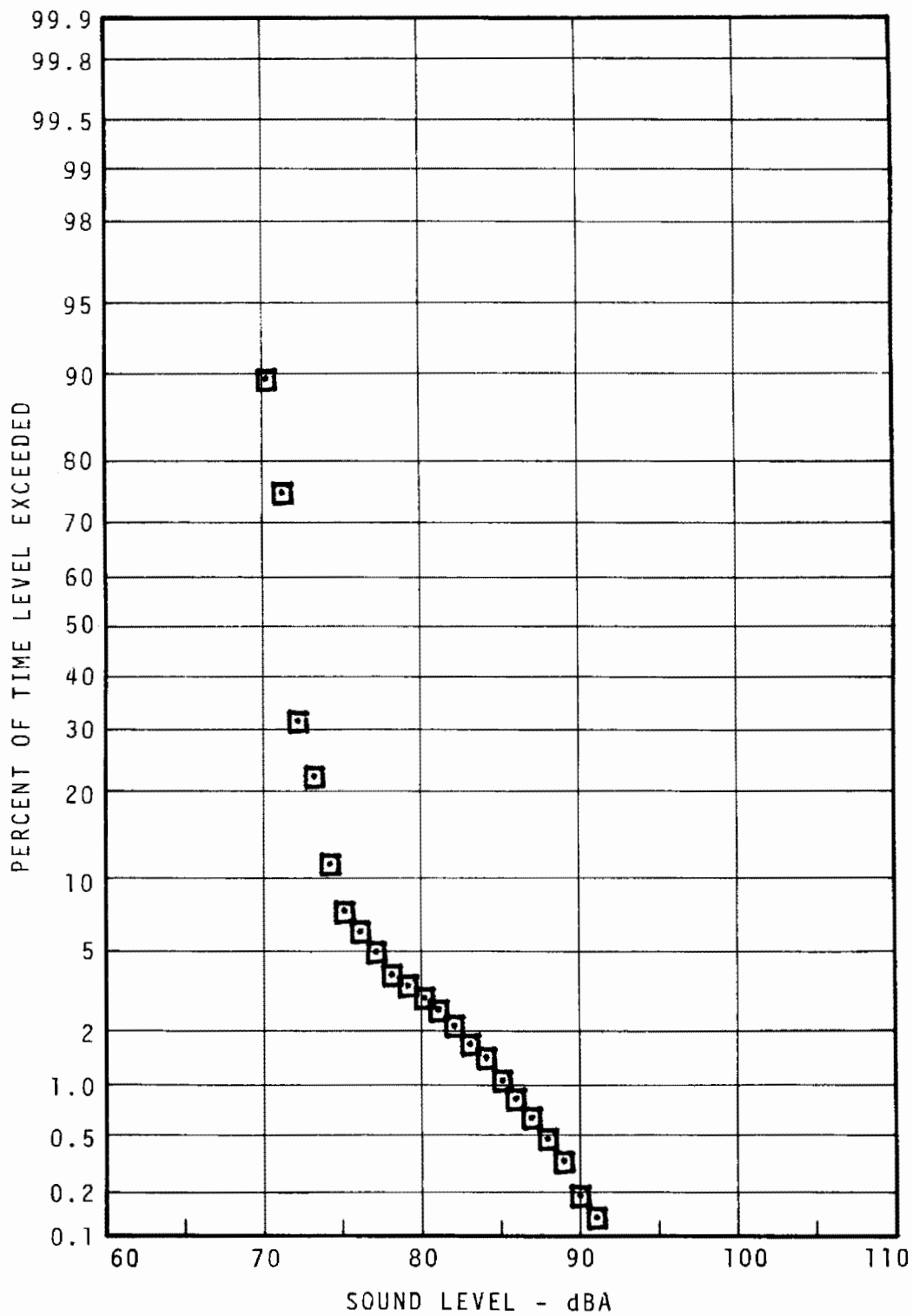
FIGURE 7.92 - BRIDGE STREET STATION PLATFORM STATISTICAL DISTRIBUTION - NIGHT
