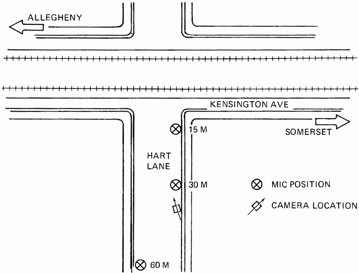
FIGURE 7.32 - WAYSIDE MEASUREMENT SITE, NEAR SOMERSET STATION. ELEVATED STEEL STRUCTURE
