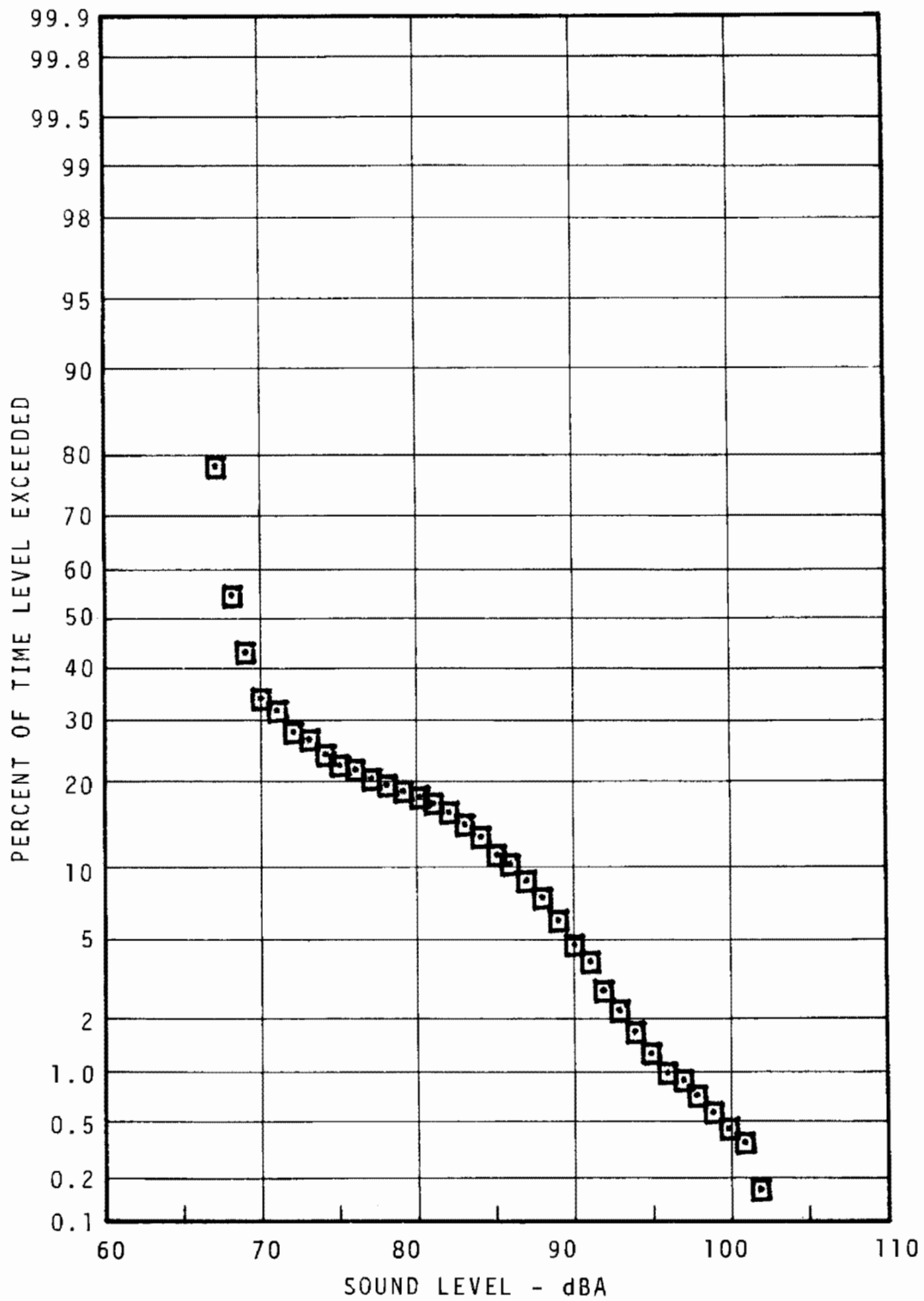
FIGURE 7.66 - 30TH STREET STATION PLATFORM STATISTICAL DISTRIBUTION - NIGHT
