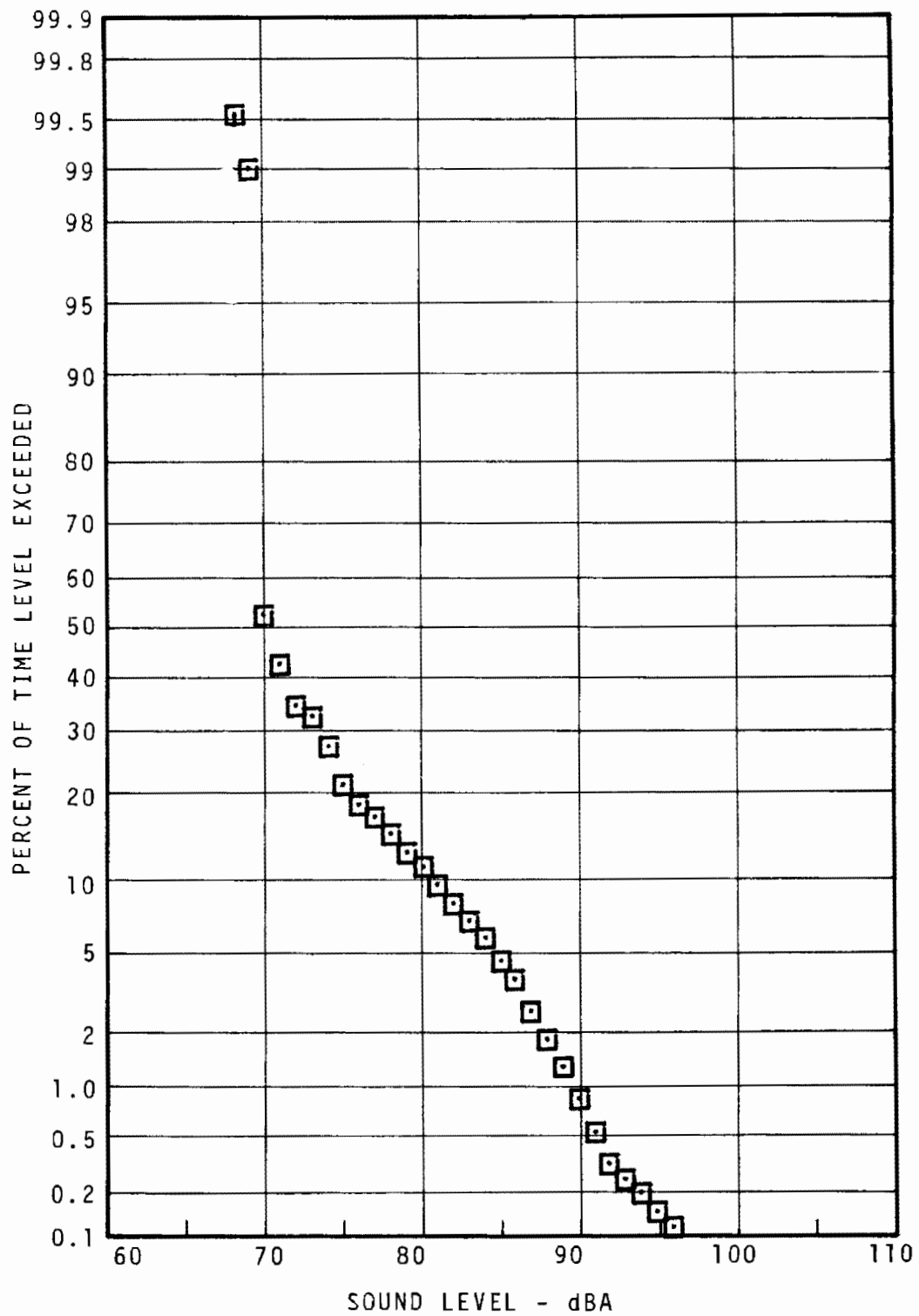
FIGURE 7.41 - 69TH ST. STATION PLATFORM STATISTICAL DISTRIBUTION - EVENING
