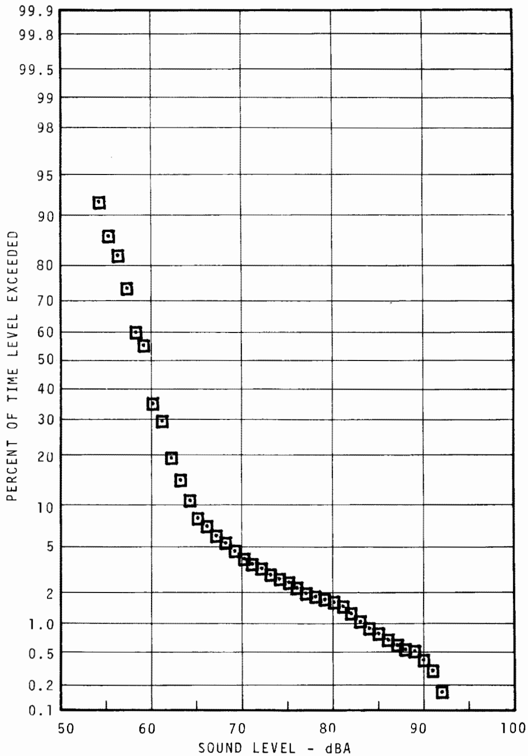
FIGURE 7.28 - YORK-DAUPHIN COMMUNITY STATISTICAL DISTRIBUTION - 15M - NIGHT
