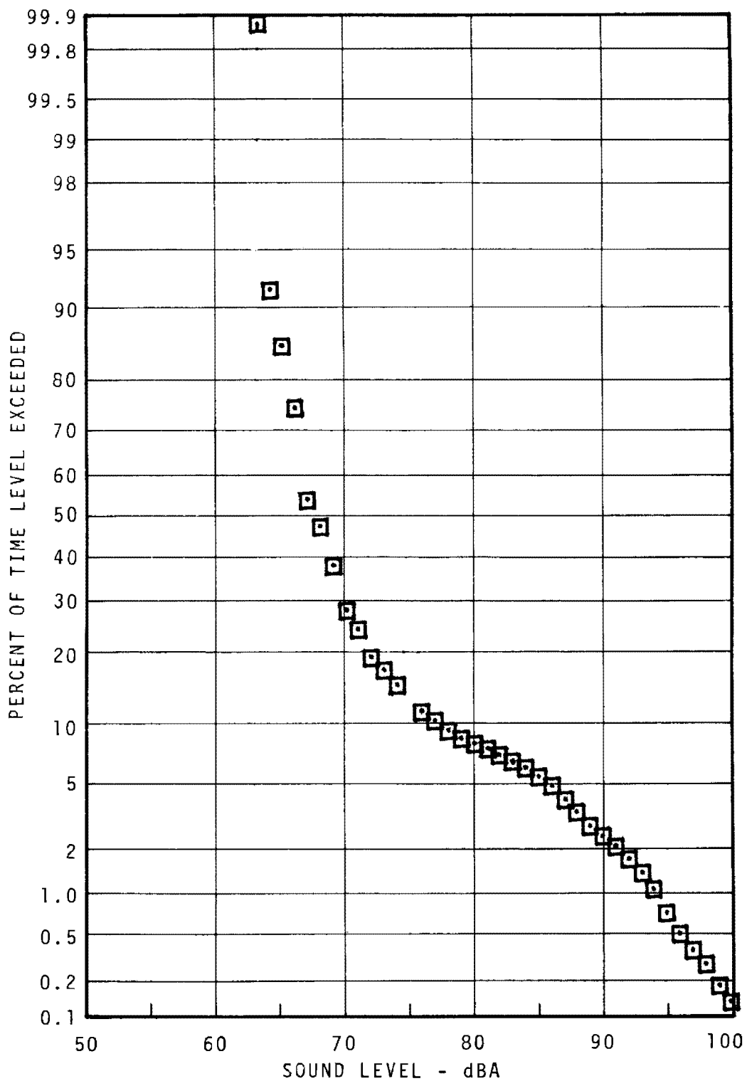
FIGURE 7.25 - YORK-DAUPHIN COMMUNITY STATISTICAL DISTRIBUTION - 15M - DAYTIME
