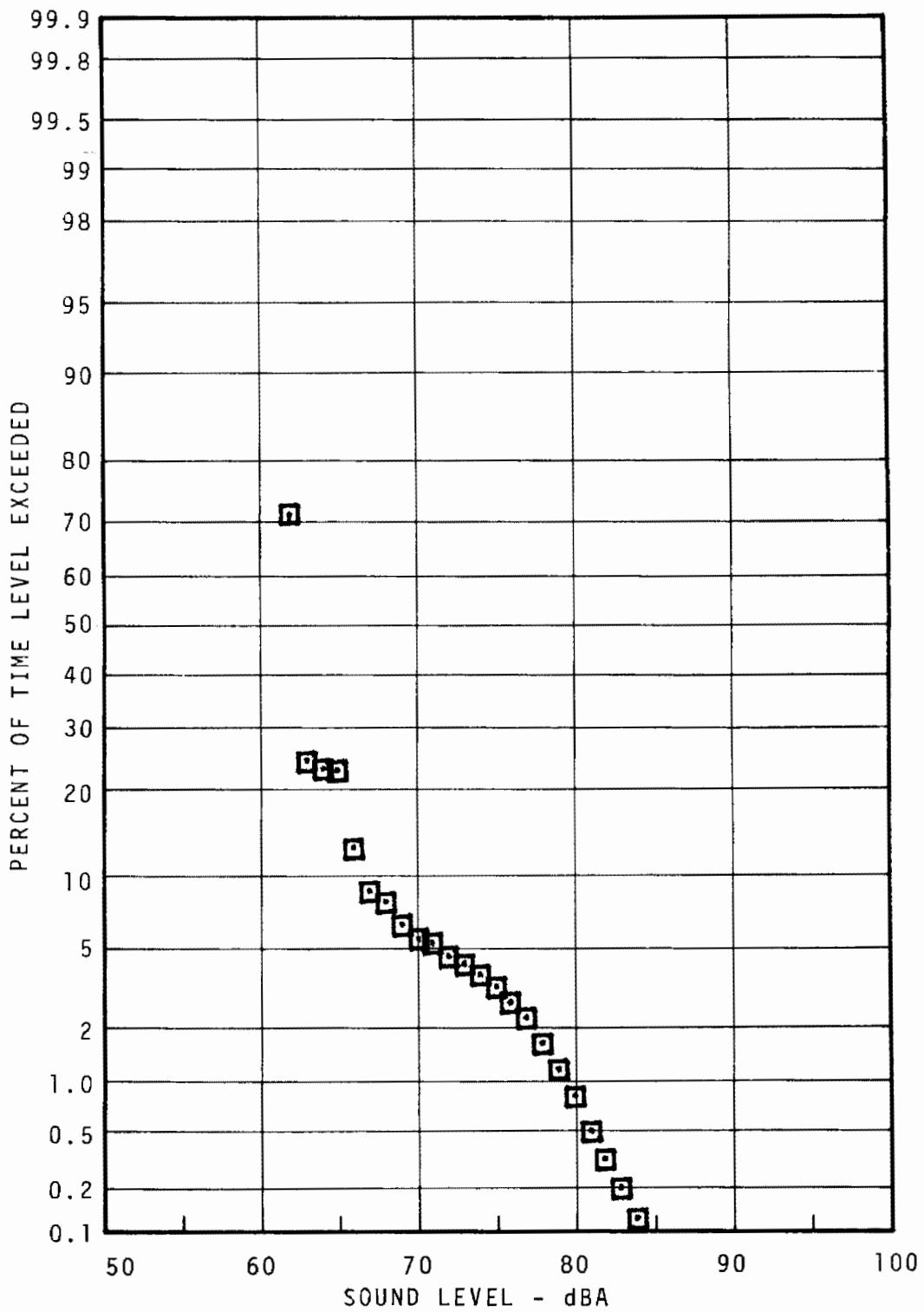
FIGURE 7.48 - MILLBOURNE STATION PLATFORM STATISTICAL DISTRIBUTION - NIGHT
