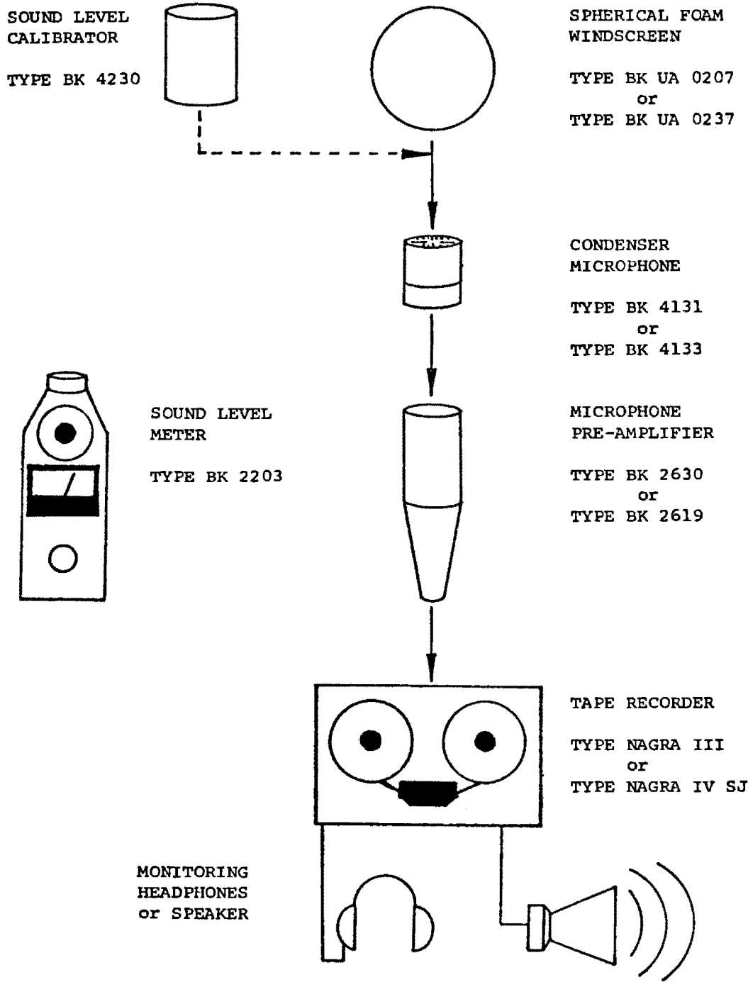
FIGURE 4.1. TYPICAL DATA ACQUISITION SYSTEM
