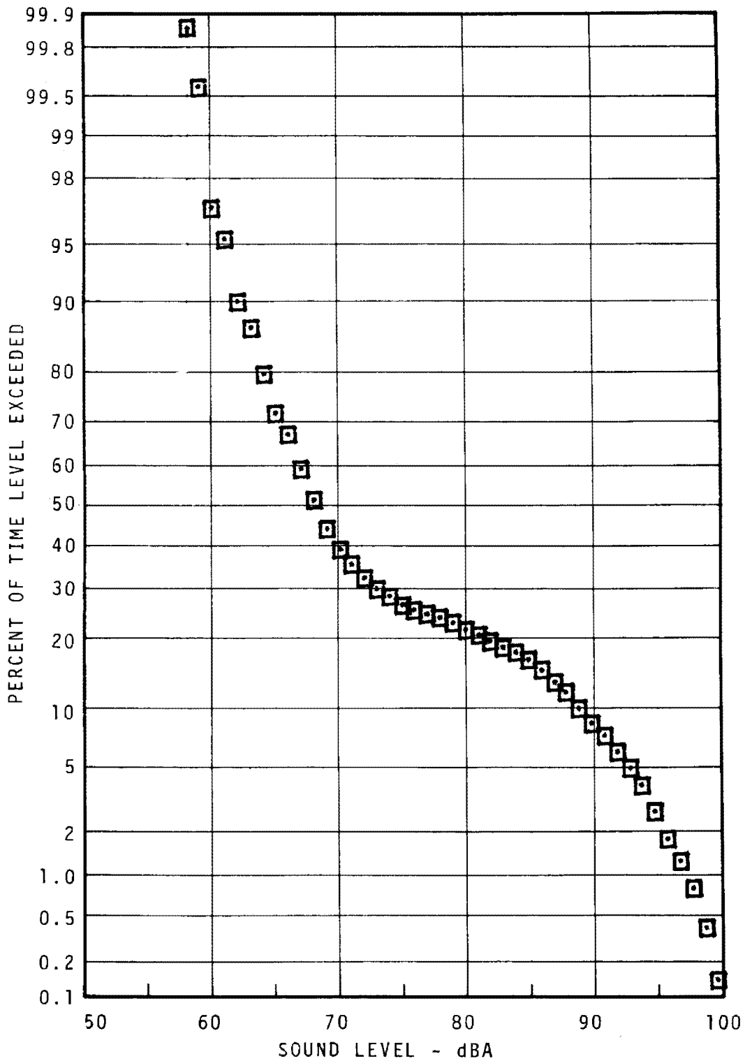
FIGURE 7.26 -YORK-DAUPHIN COMMUNITY STATISTICAL DISTRIBUTION - 15M - RUSH HOUR
