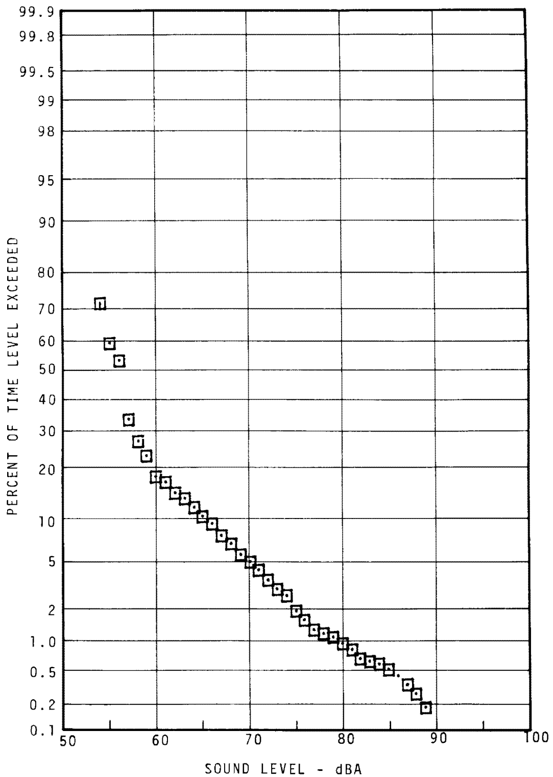
FIGURE 5.29 - FERN ROCK LOCATION PLATFORM STATISTICAL DISTRIBUTION NIGHT
