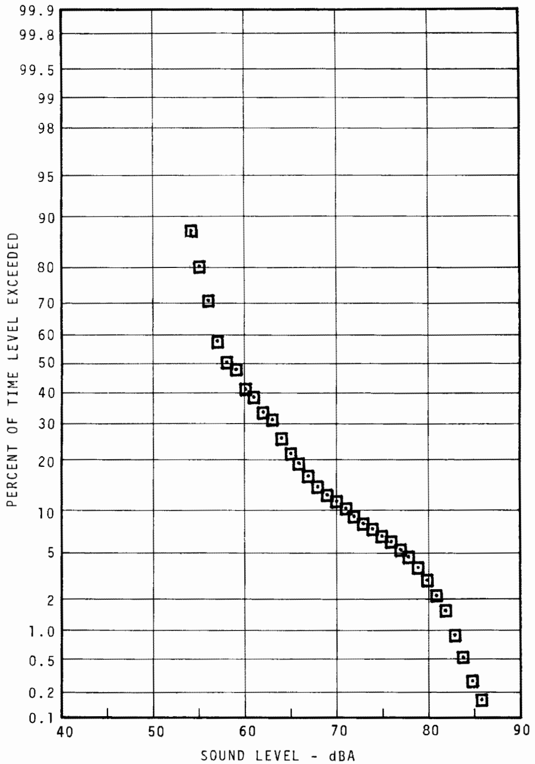
FIGURE 5.28 - FERN ROCK STATION PLATFORM STATISTICAL DISTRIBUTION EVENING
