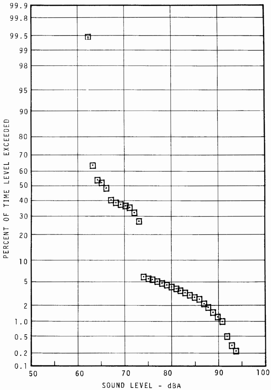
FIGURE 7.72 - 5TH STREET STATION PLATFORM STATISTICAL DISTRIBUTION - NIGHT
