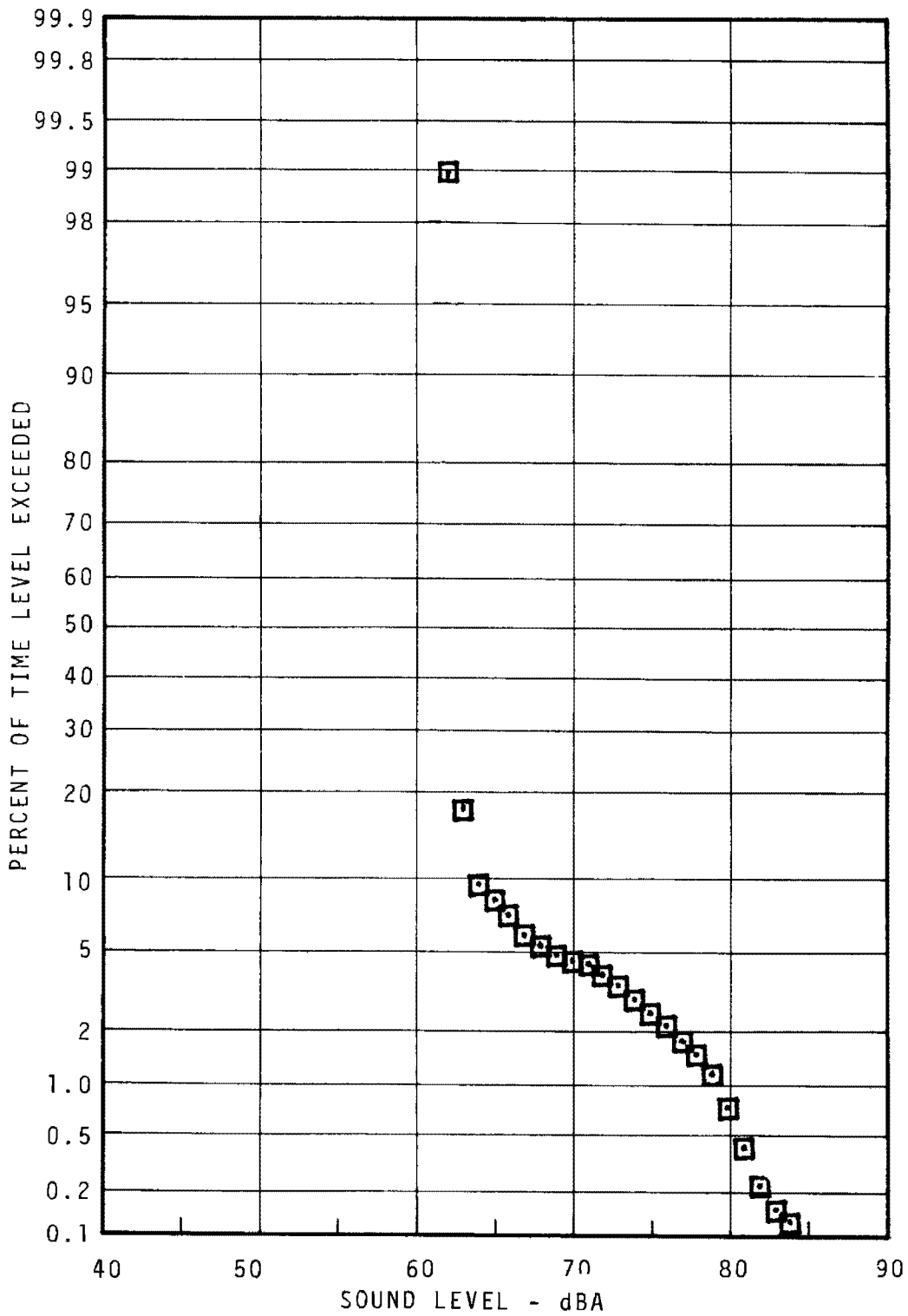
FIGURE 7.54 - 52ND STREET STATION PLATFORM STATISTICAL DISTRIBUTION - NIGHT
