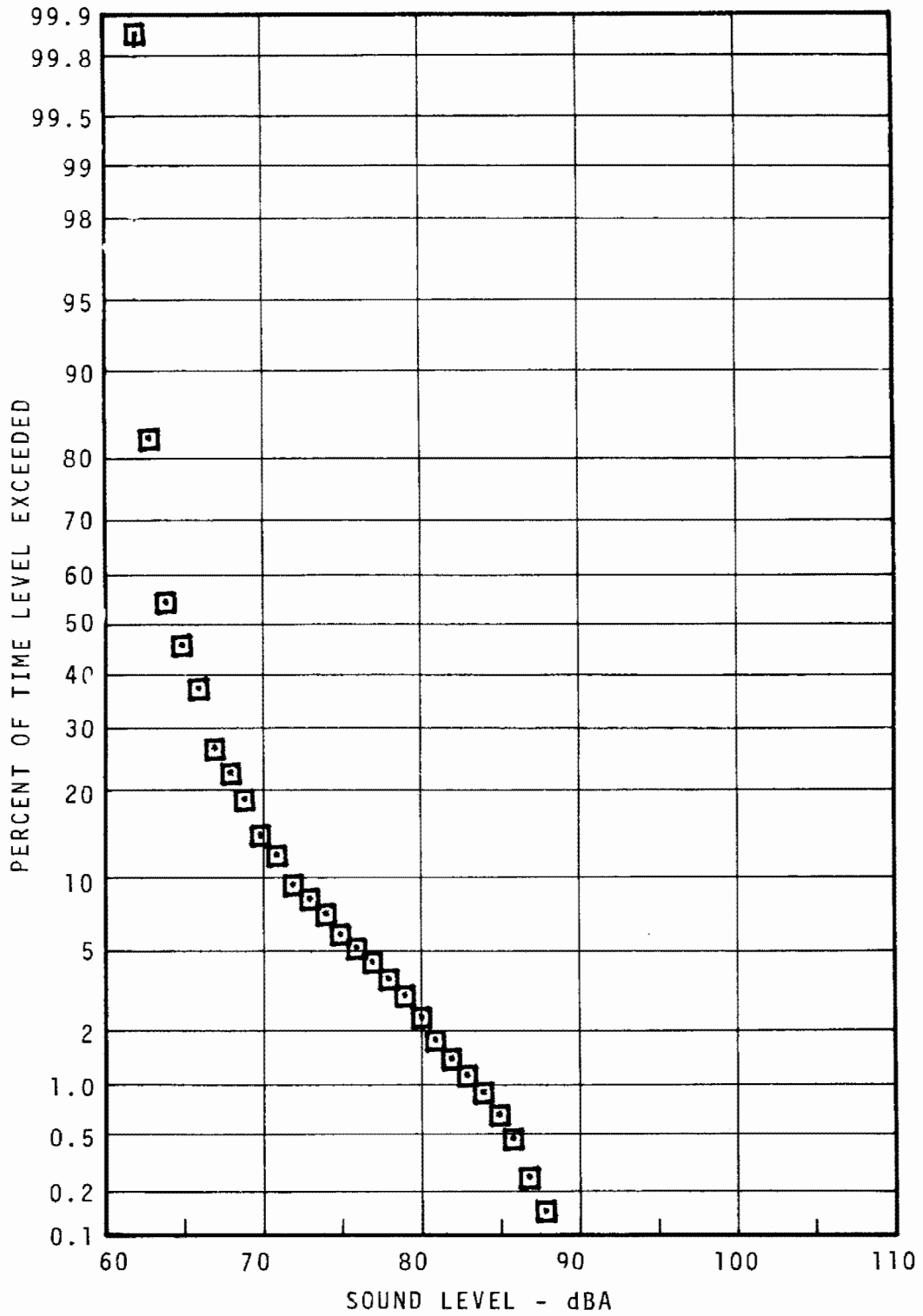
FIGURE 7.29 - YORK-DAUPHIN COMMUNITY STATISTICAL DISTRIBUTION - 60M - DAYTIME
