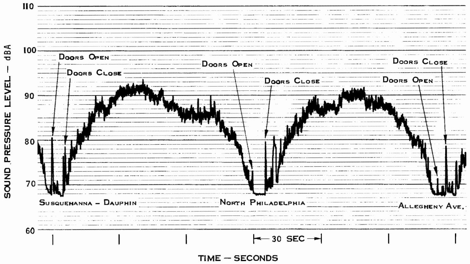
FIGURE 5.73-TIME HISTORY OF IN CAR NOISE ENVIRONMENT 1928 BRILL CAR SEPTA BROAD STREET LINE - CENTER CAR
