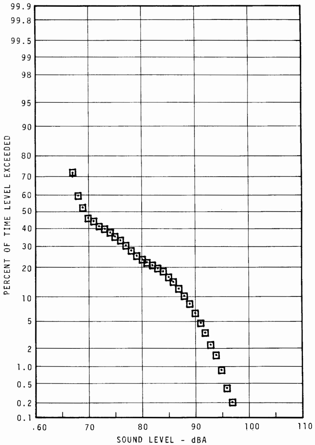
FIGURE 7.46 - MILLBOURNE STATION PLATFORM STATISTICAL DISTRIBUTION - RUSH HOUR
