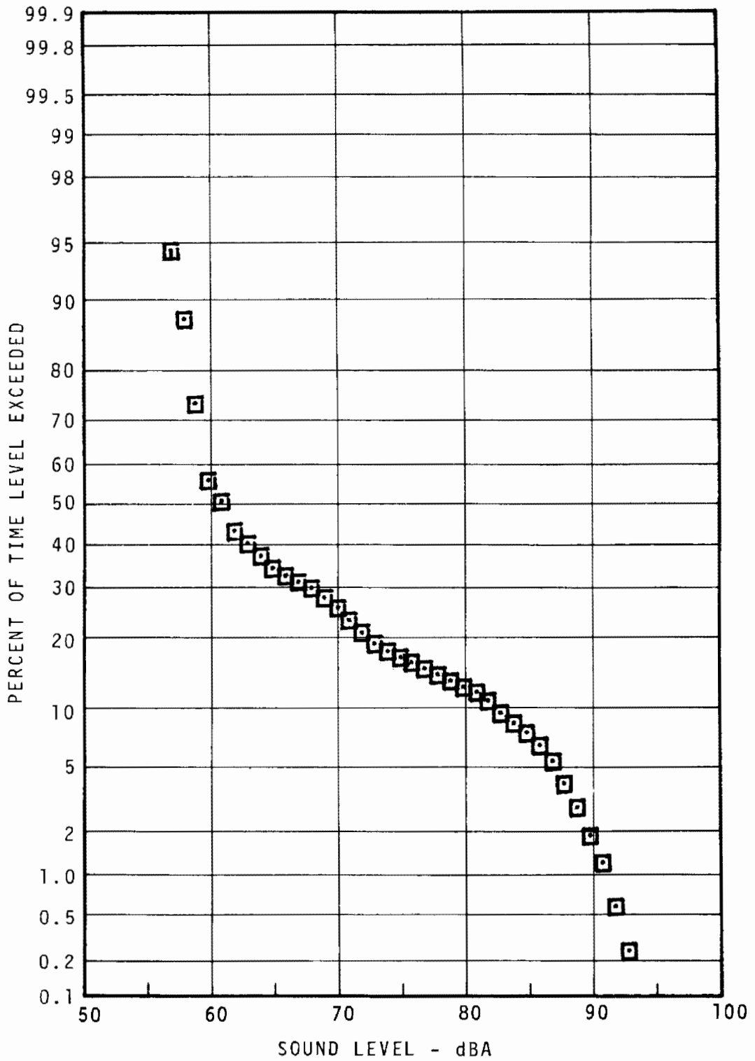
FIGURE 5.49 - CITY HALL STATION PLATFORM STATISTICAL DISTRIBUTION EVENING
