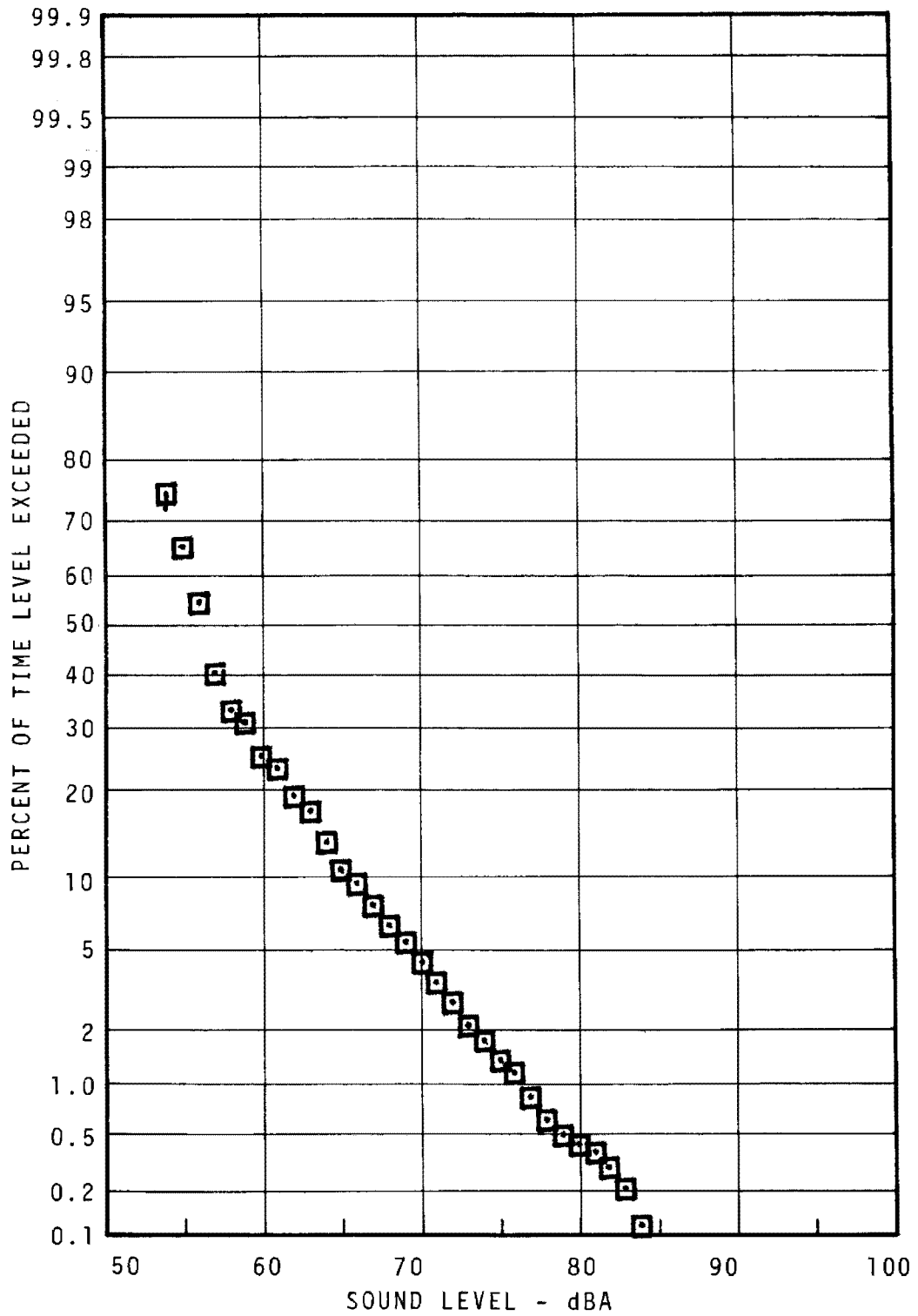
FIGURE 7.36 - SOMERSET COMMUNITY STATISTICAL DISTRIBUTION - 15M - NIGHT
