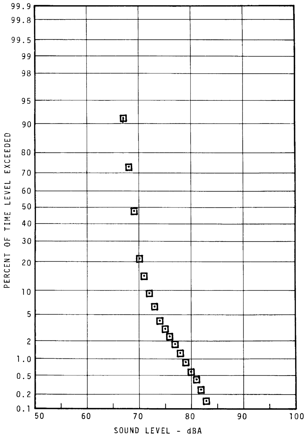
FIGURE 7.42 - 69TH ST. STATION PLATFORM STATISTICAL DISTRIBUTION - NIGHT
