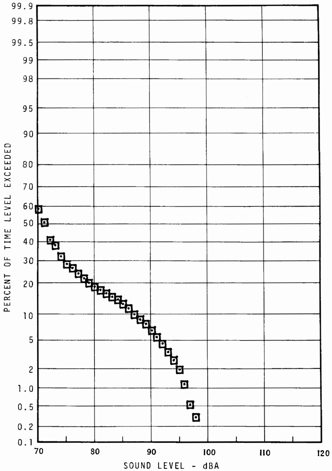
FIGURE 7.79 - BERKS STATION PLATFORM STATISTICAL DISTRIBUTION - RUSH HOUR
