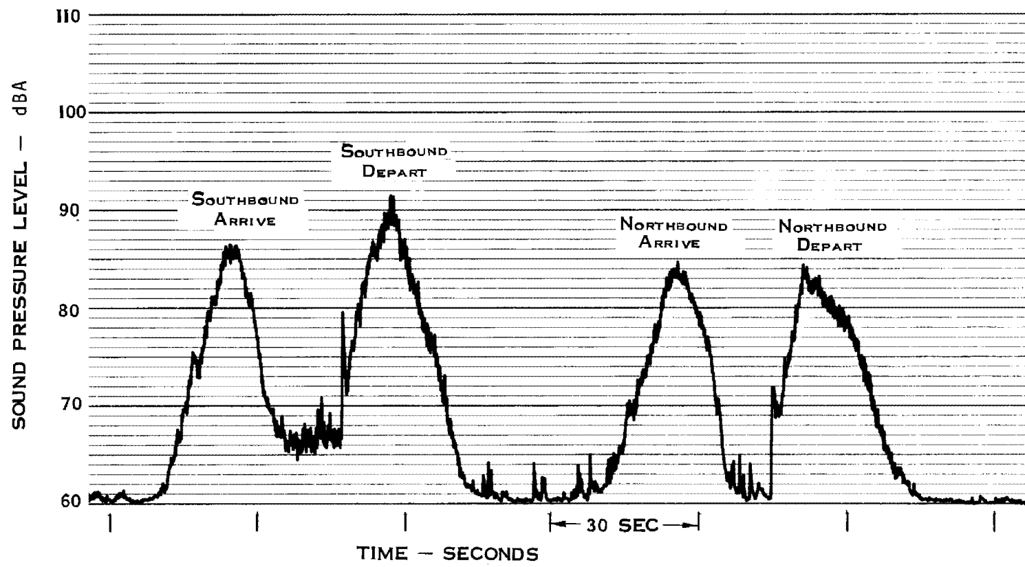
FIGURE 5.42 -TYPICAL TIME HISTORY SPRING GARDEN ST. STATION CENTER PLATFORM (EXPRESS TRACK)
