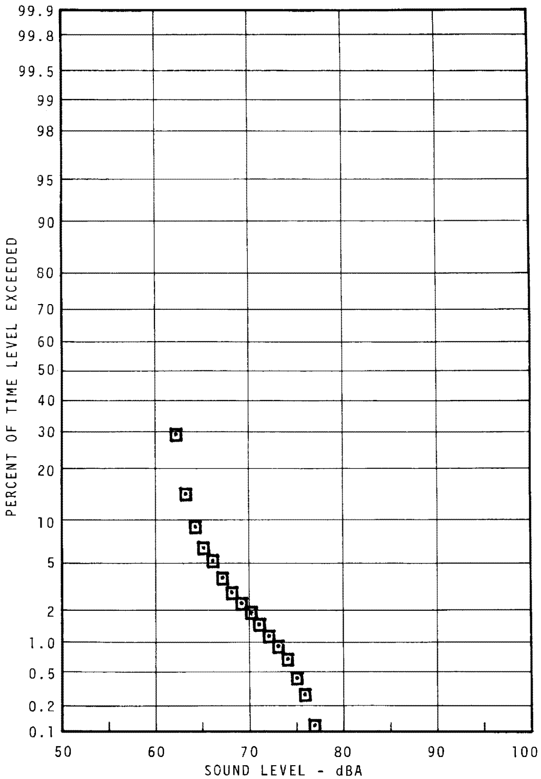
FIGURE 7.13 - MILLBOURNE COMMUNITY STATISTICAL DISTRIBUTION - 15M - NIGHT
