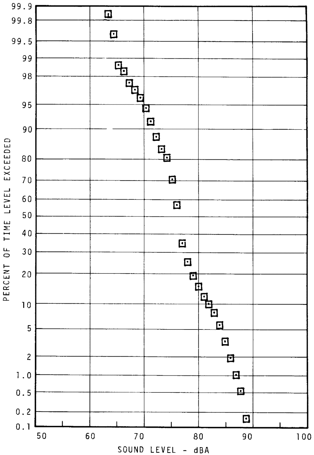
FIGURE 7.39 - 69TH ST. STATION PLATFORM STATISTICAL DISTRIBUTION - DAYTIME
