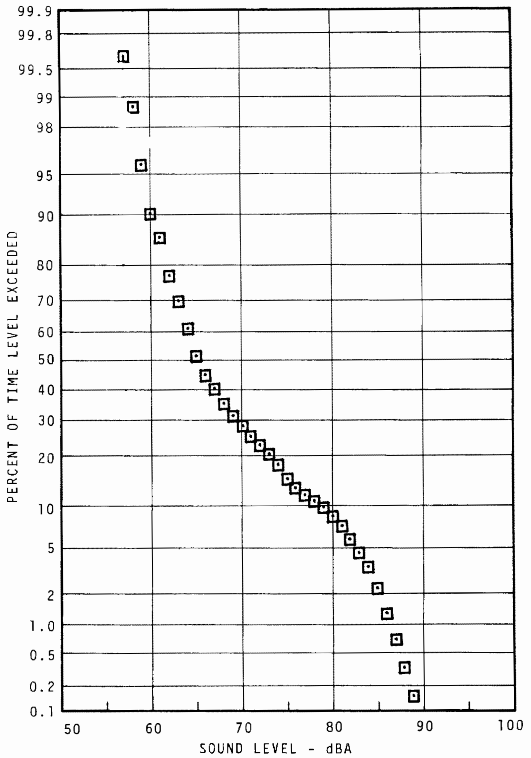
FIGURE 7.86 - CHURCH STREET STATION PLATFORM STATISTICAL DISTRIBUTION - DAYTIME
