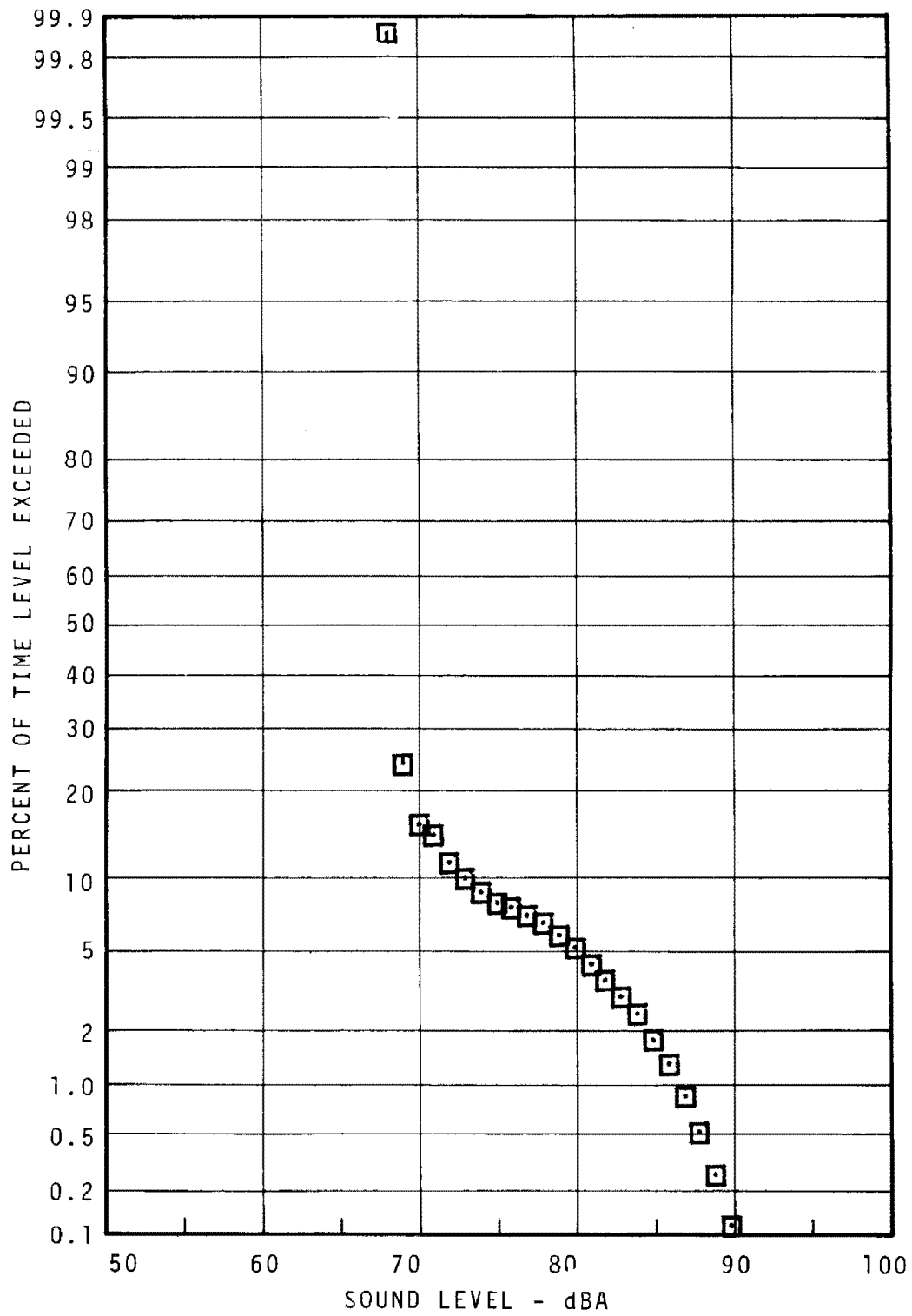
FIGURE 7.47 - MILLBOURNE STATION PLATFORM STATISTICAL DISTRIBUTION - EVENING
