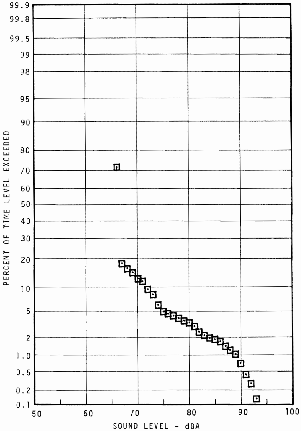
FIGURE 5.65 - PATTSION AVENUE STATION PLATFORM STATISTICAL DISTRIBUTION NIGHT
