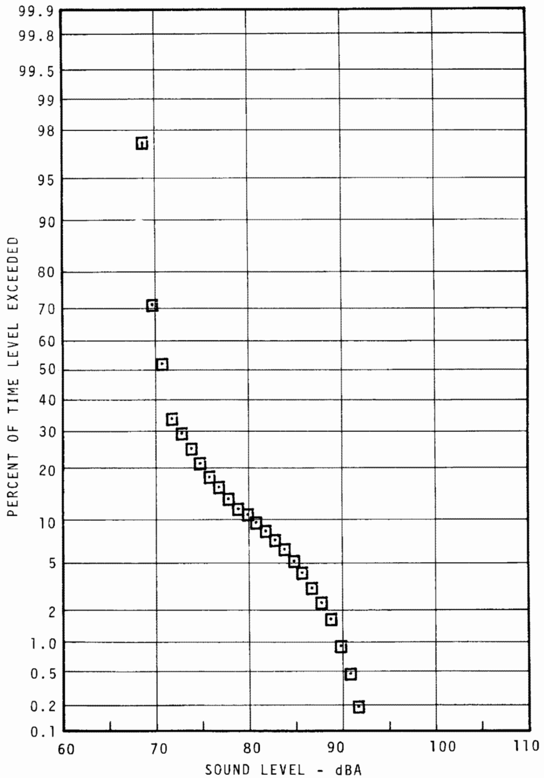
FIGURE 7.53 - 52ND STREET STATION PLATFORM STATISTICAL DISTRIBUTION - EVENING
