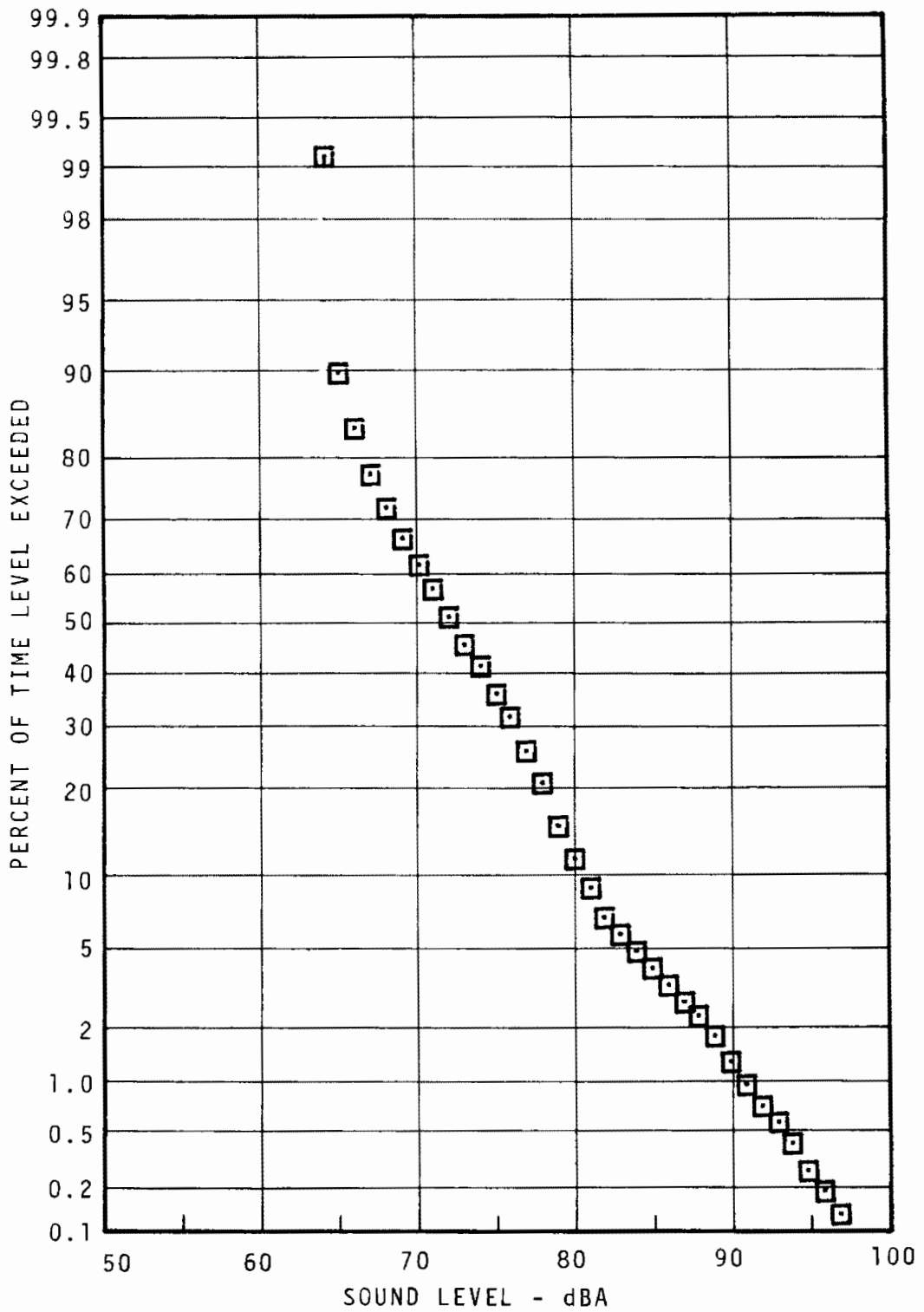
FIGURE 7.6 - 69TH ST. COMMUNITY STATISTICAL DISTRIBUTION - 15M - EVENING
