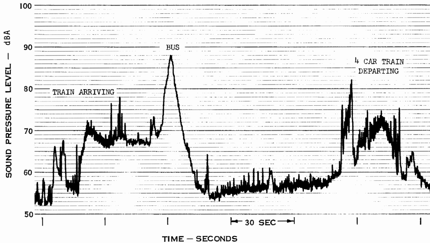
FIGURE 5.12-TYPICAL NOISE TIME HISTORY, 10 TH & NEDRO St. COMMUNITY, 25 METERS SEPTA BROAD STREET LINE
