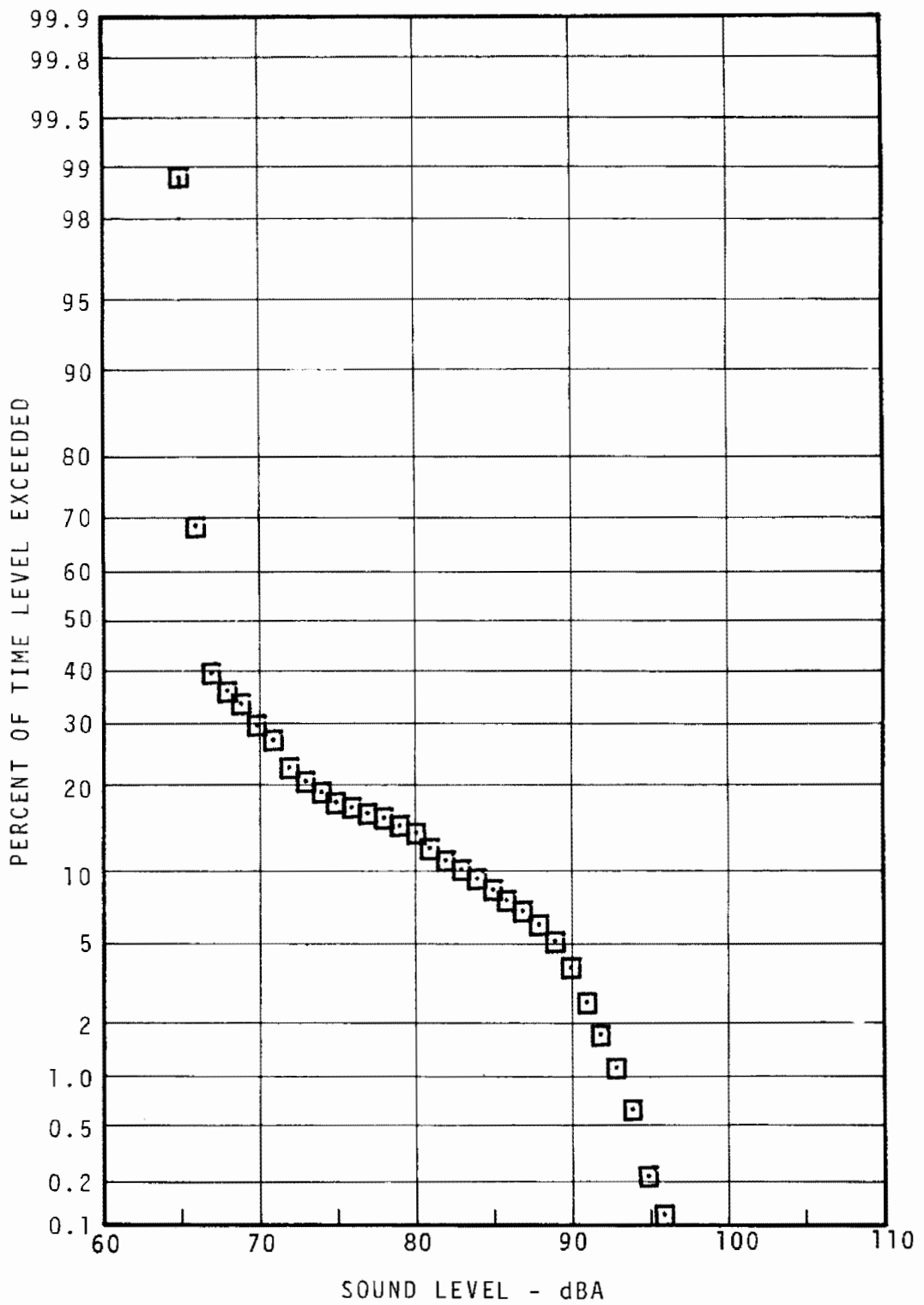
FIGURE 5.47 - CITY HALL STATION PLATFORM STATISTICAL DISTRIBUTION DAYTIME
