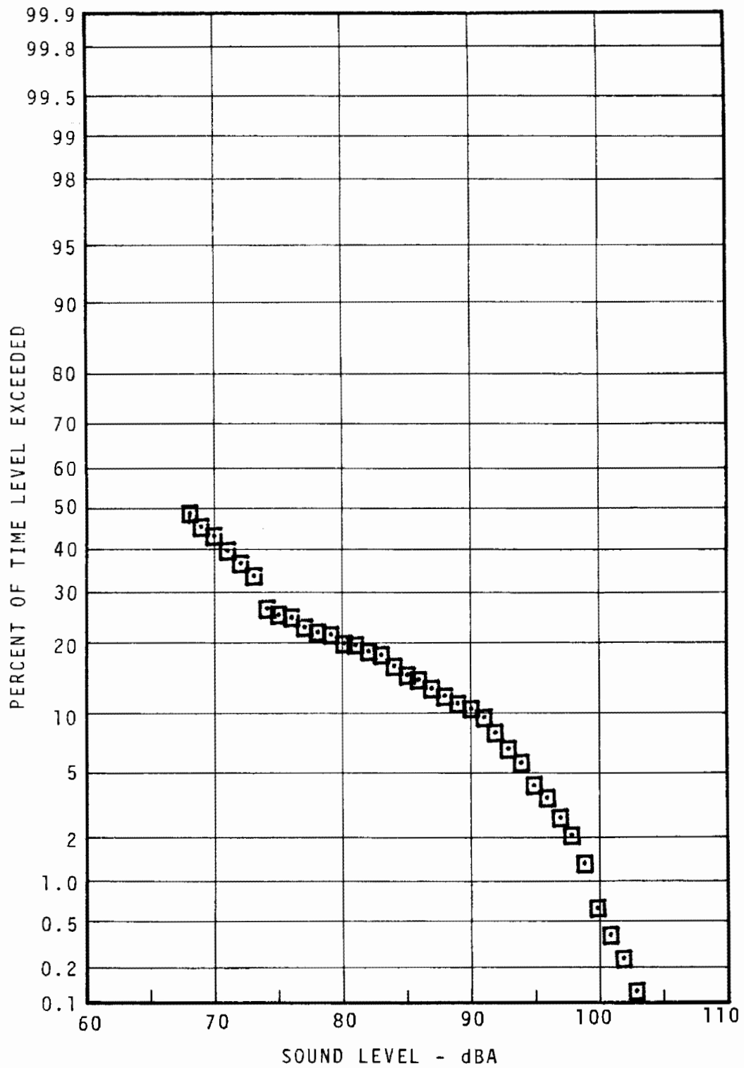
FIGURE 7.57 - 40TH STREET STATION PLATFORM STATISTICAL DISTRIBUTION - DAYTIME
