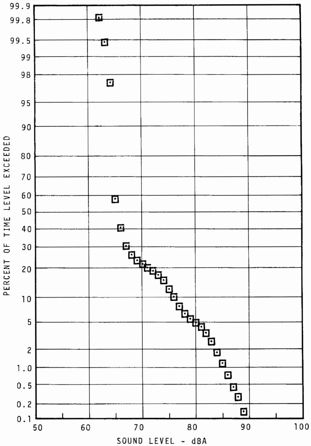
FIGURE 7.11 - MILLBOURNE COMMUNITY STATISTICAL DISTRIBUTION - 15M - RUSH HOUR
