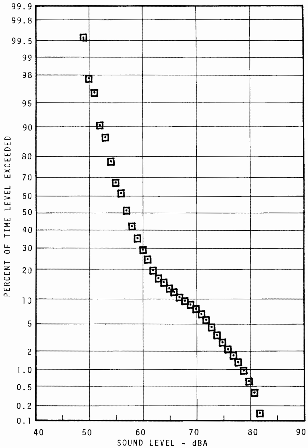
FIGURE 7.12 - MILLBOURNE COMMUNITY STATISTICAL DISTRIBUTION - 15M - EVENING
