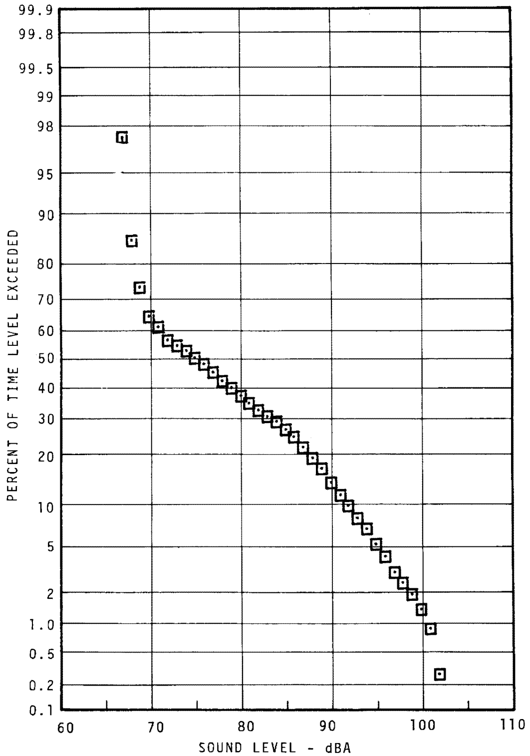
FIGURE 7.65 - 30TH STREET STATION PLATFORM STATISTICAL DISTRIBUTION - EVENING
