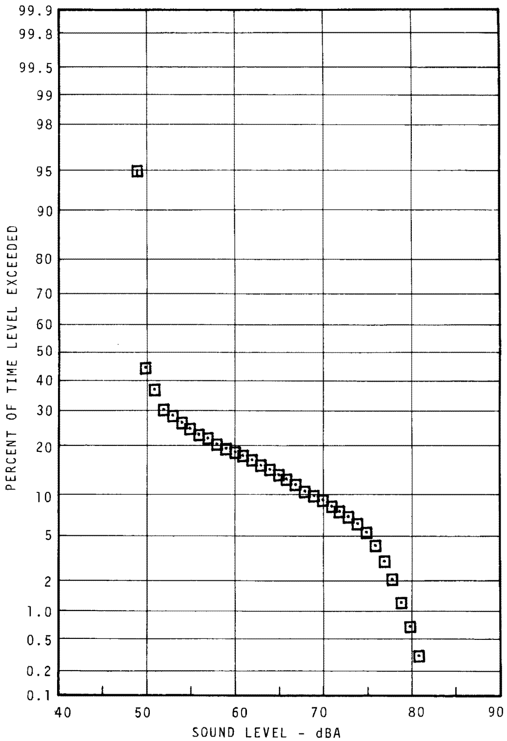
FIGURE 7.45 - MILLBOURNE STATION PLATFORM STATISTICAL DISTRIBUTION - DAYTIME
