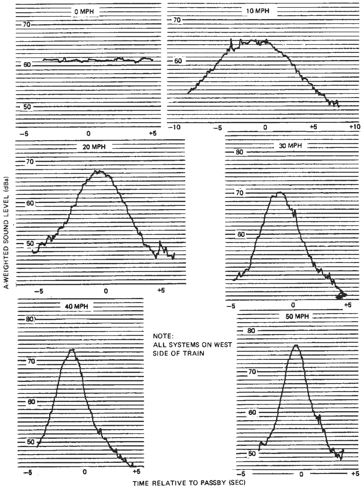
Figure 3-10. SLRV Wayside Noise Time Histories, 50-Ft, Two-Car Train, SFMR Configuration, AWO
