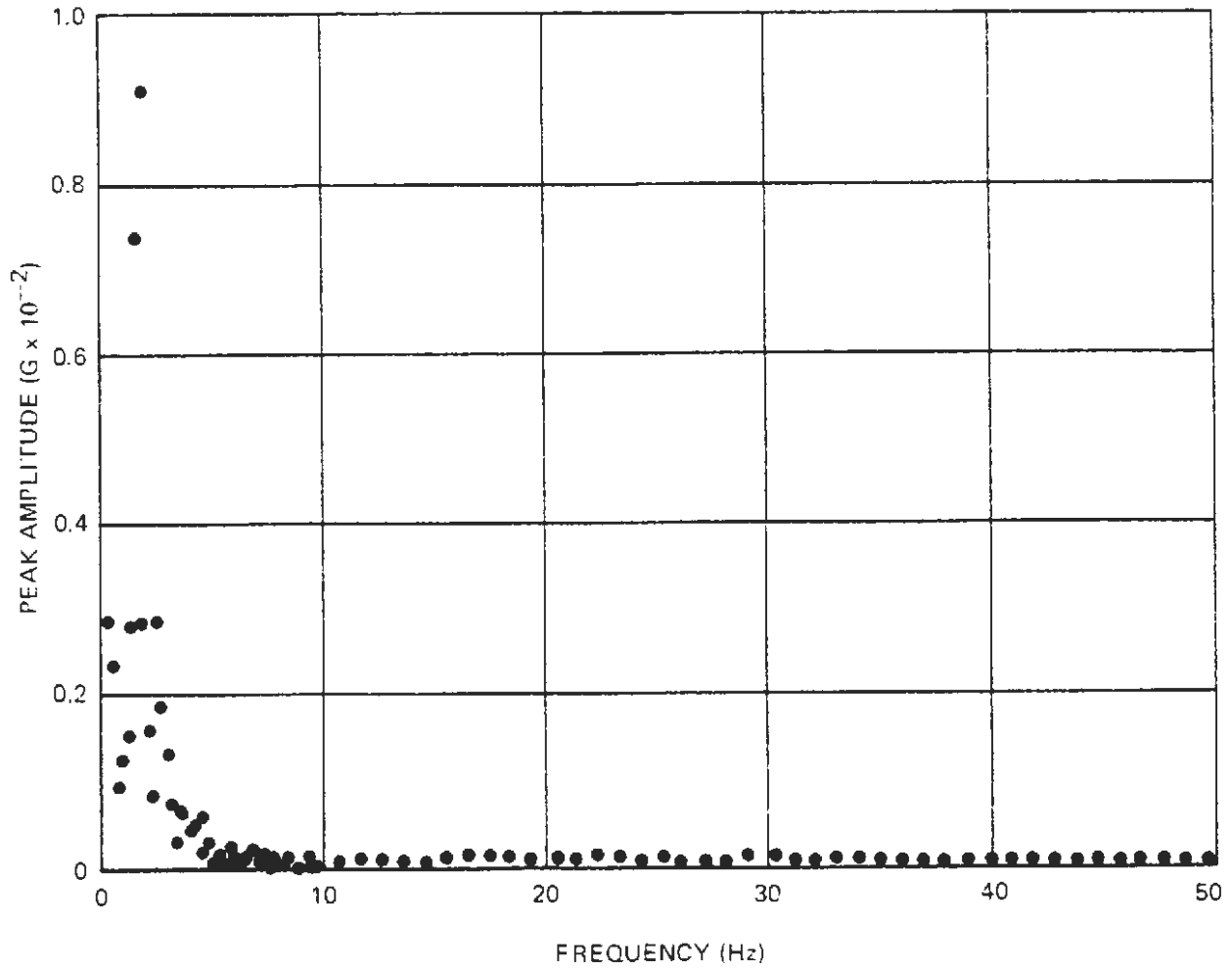
Figure A-22. Narrow-Band Spectrum Analysis – End Car, Lateral
