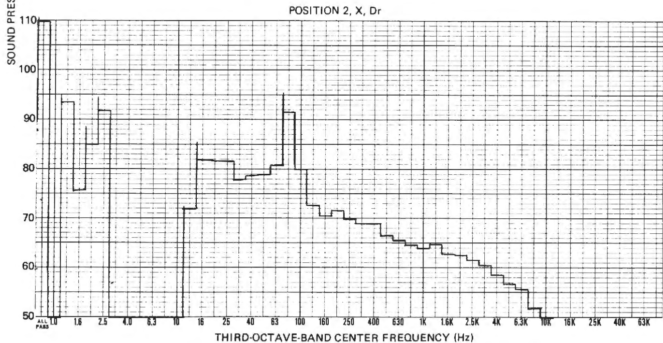
Figure 3-33. Third-Octave Band Analysis of SFMR Interior Noise, AWO, 40 mph.
