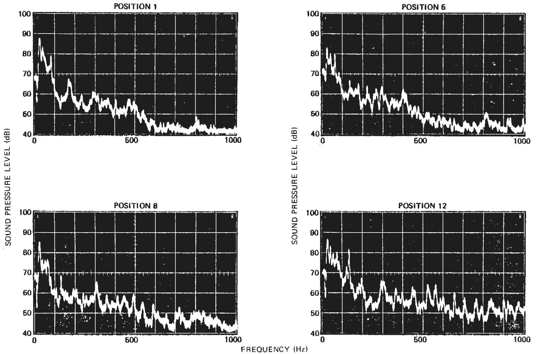
Figure 3-51. Narrowband Analysis of Interior Noise, MBTA, AW0, 50 mph
