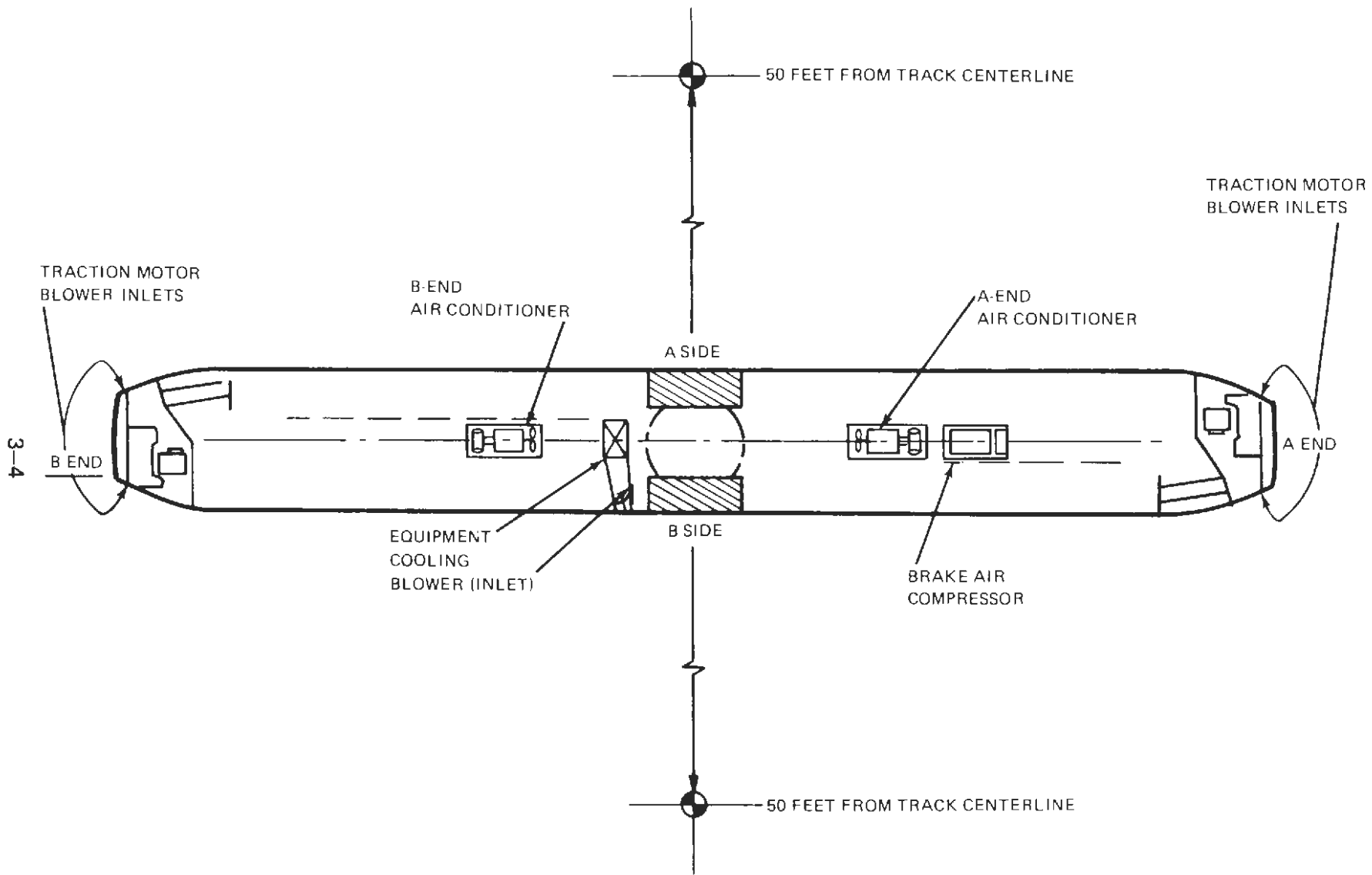
Figure 3-2. SLRV Undercar Equipment Measured for Wayside Noise
