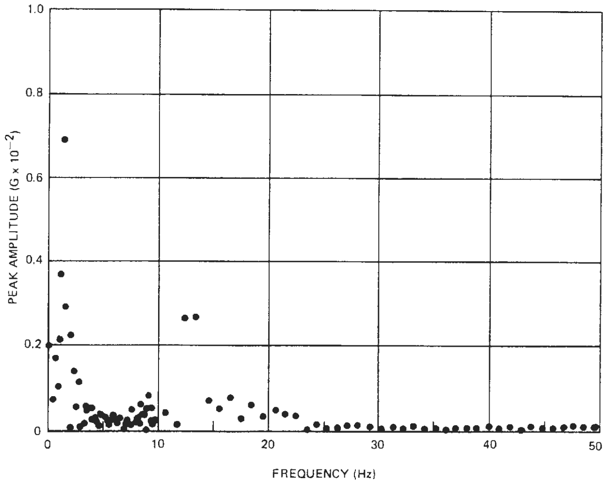
Figure A-49. Narrow-Band Spectrum Analysis – End Car, Lateral
