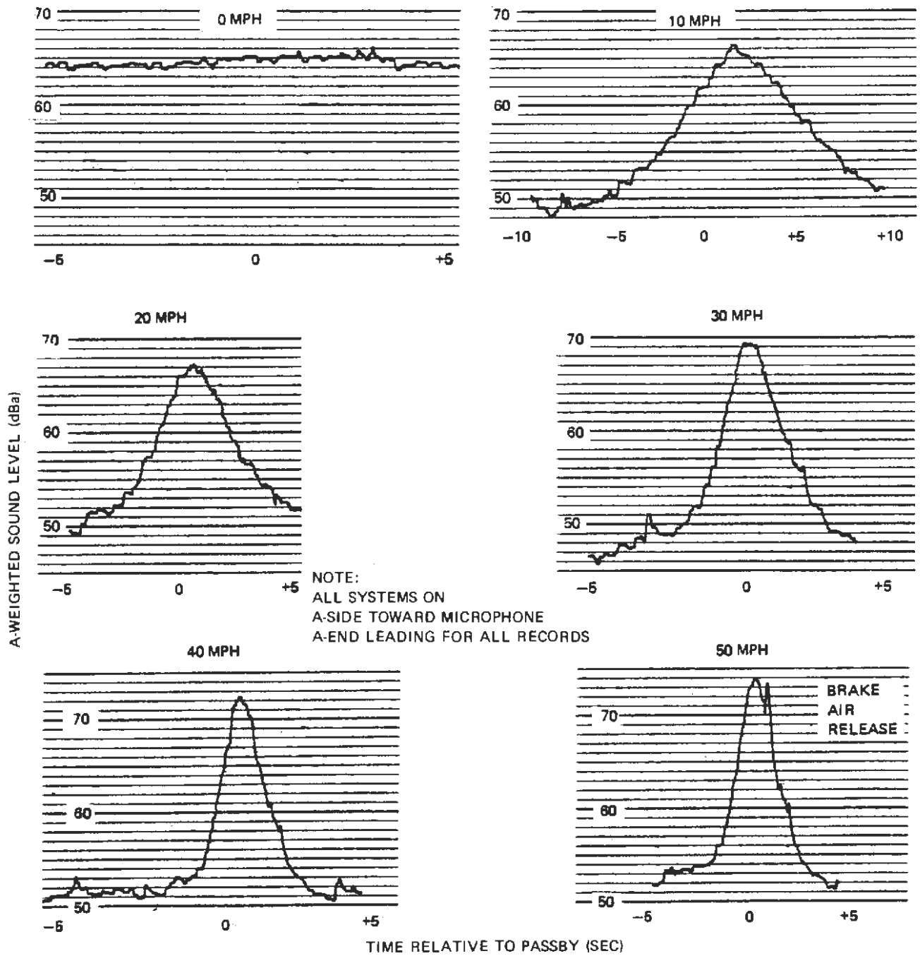
Figure 3-B. SLRV Wayside Noise Time Histories, 50-Ft Single Car, MBTA Configuration, AWO
