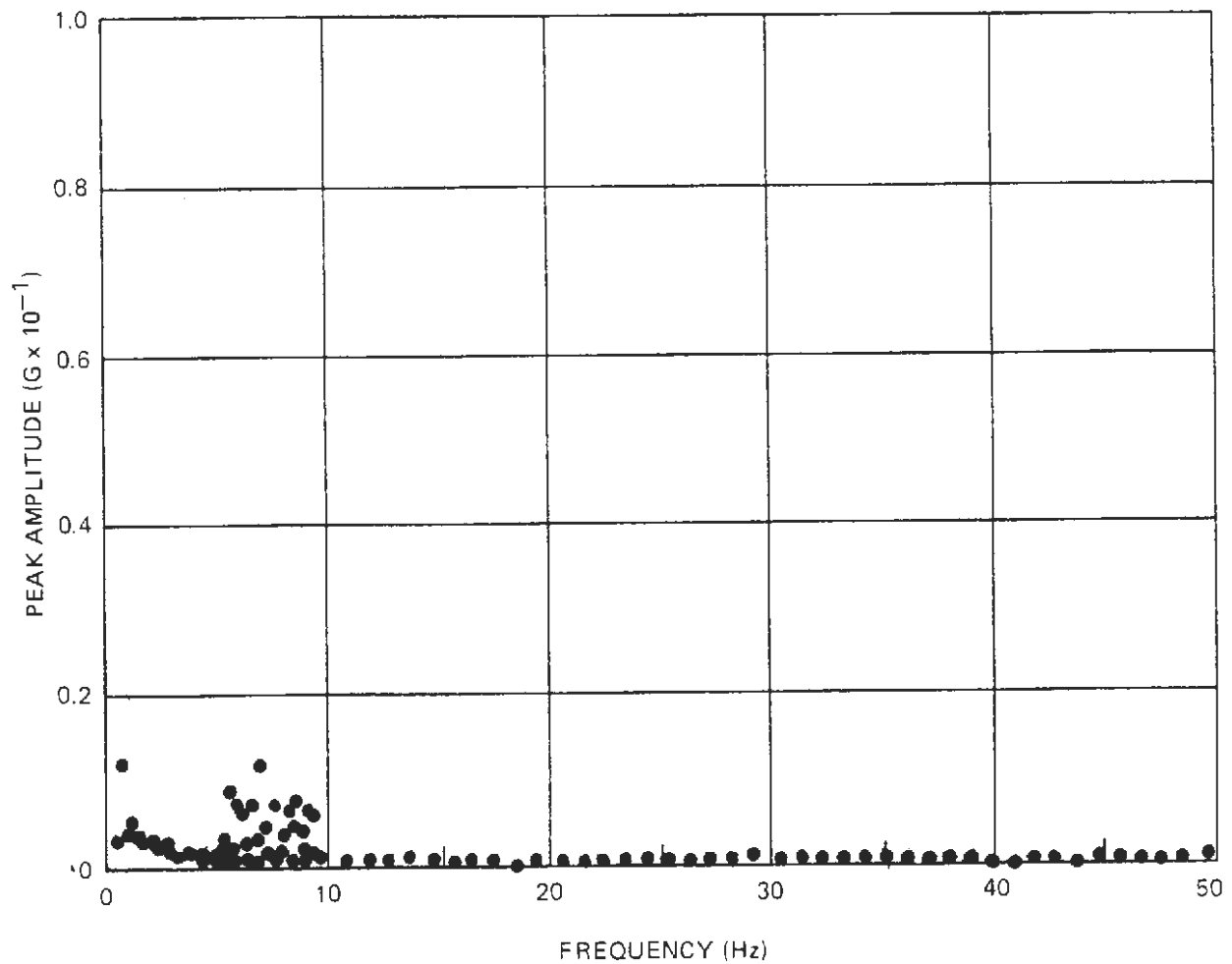
Figure A-47. Narrow-Band Spectrum Analysis – Mid Car, Longitudinal
