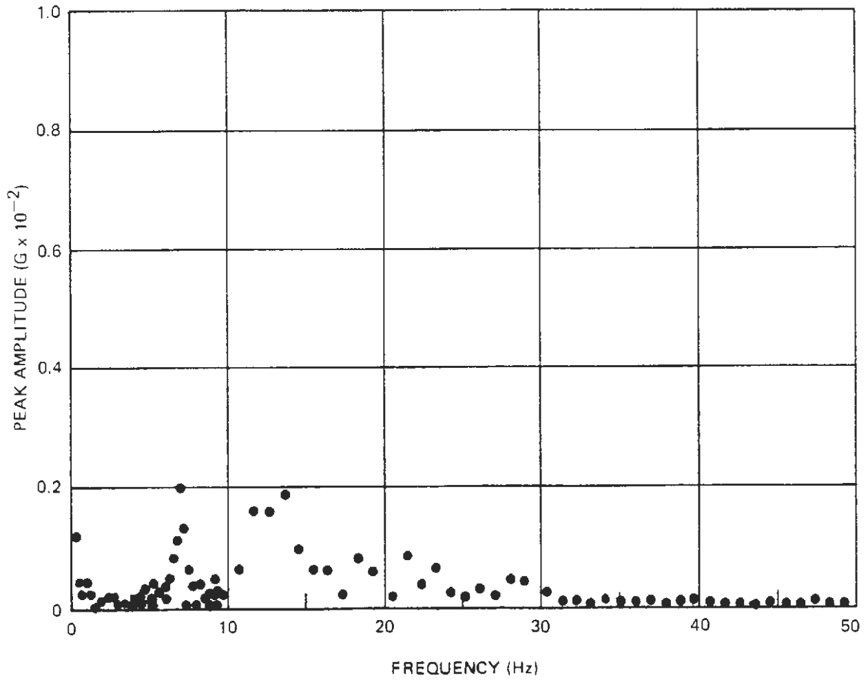
Figure A-53. Narrow-Band Spectrum Analysis — Mid Car, Longitudinal
