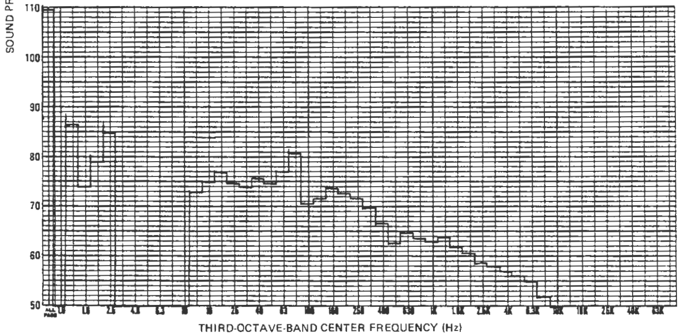
Figure 3-23. Third-Octave-Band Analysis of SFMR Interior Noise, AWO, 50 mph
