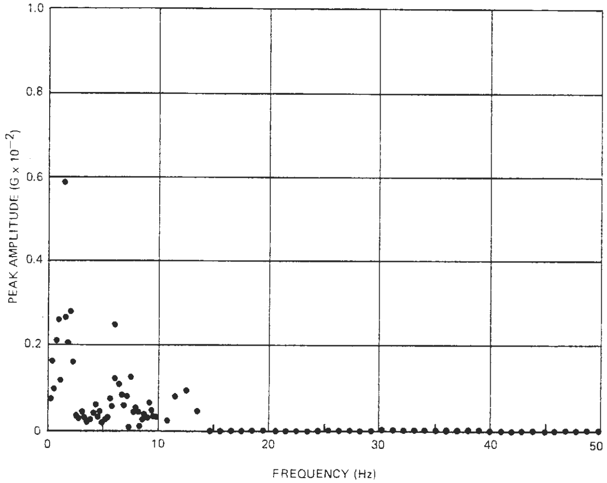
Figure A-11. Narrow-Band Spectrum Analysis – End Car, Vertical
