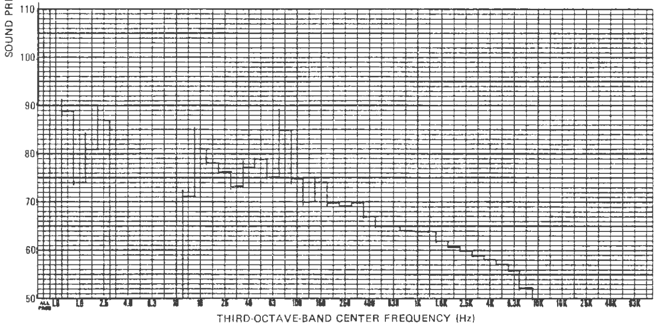
Figure 3-34. Third-Octave-Band Analysis of SFMR Interior Noise, AWO, 40 mph
