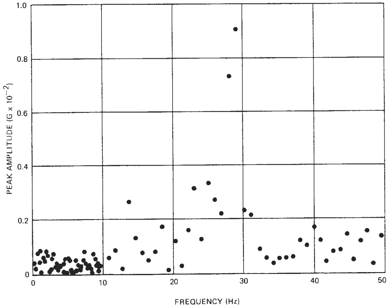
Figure A-39. Narrow-Band Spectrum Analysis – Mid Car, Vertical
