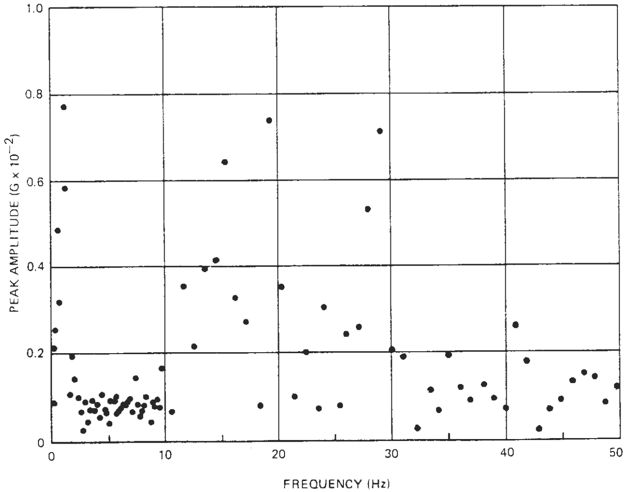
Figure A-45. Narrow-Band Spectrum Analysis – Mid Car, Vertical
