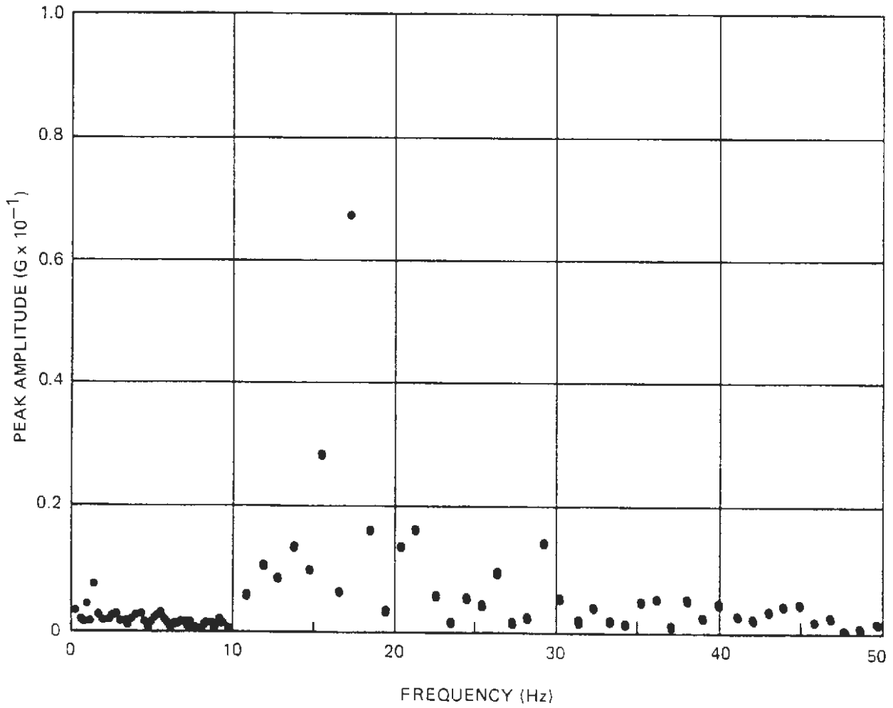
Figure A-57. Narrow-Band Spectrum Analysis -- Mid Car, Vertical
