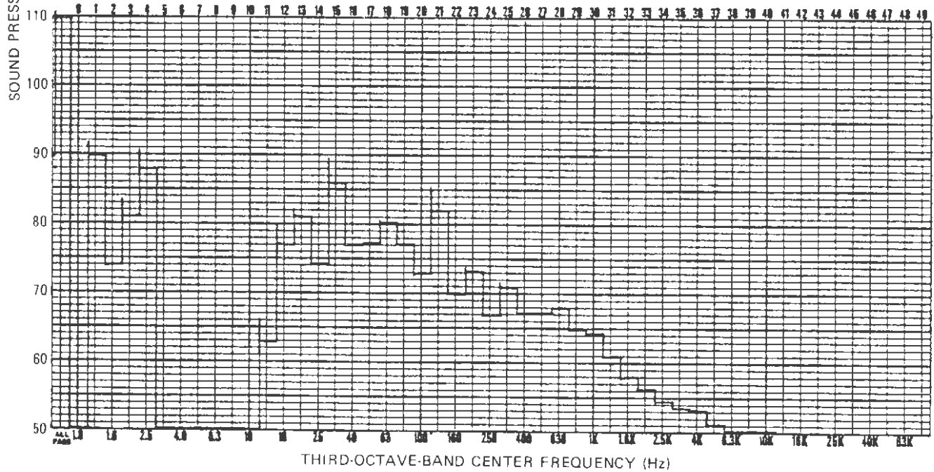
Figure 3-28. Third-Octave-Band Analysis of MBTA Interior Noise, AW0, 25 mph
