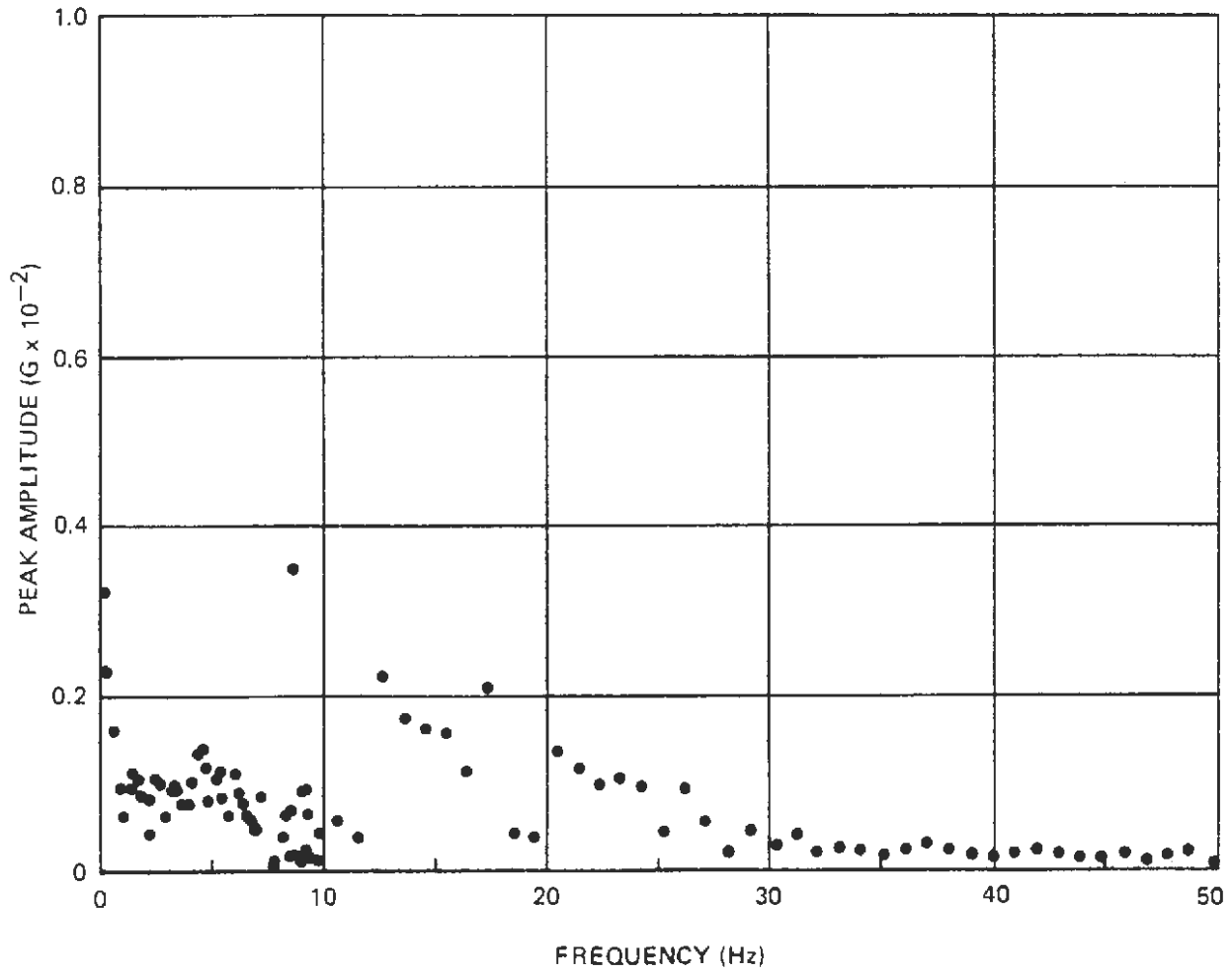
Figure A-59. Narrow-Band Spectrum Analysis – Mid Car, Longitudinal
