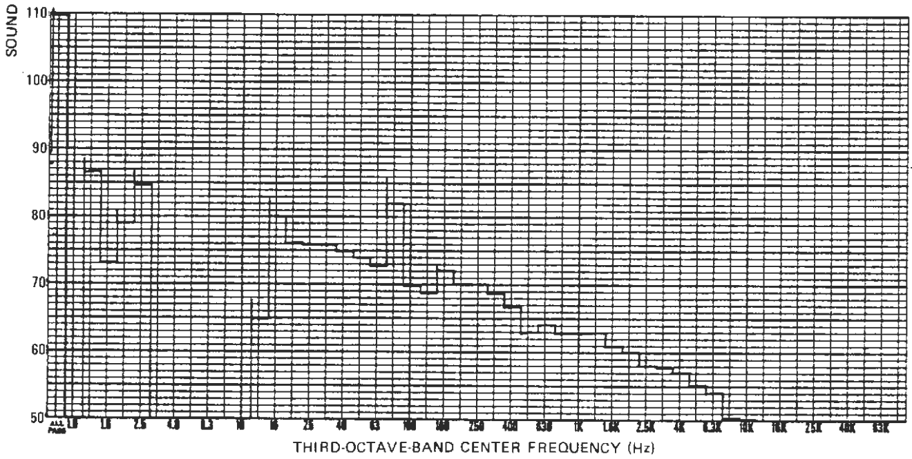
Figure 3-37. Third-Octave-Band Analysis of SFMR Interior Noise, AWO, 40 mph
