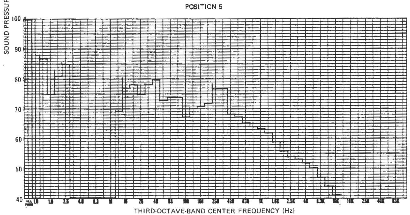
Figure 3-29. Third-Octave-Band Analysis of MBTA Interior Noise, AW0, 35 mph
