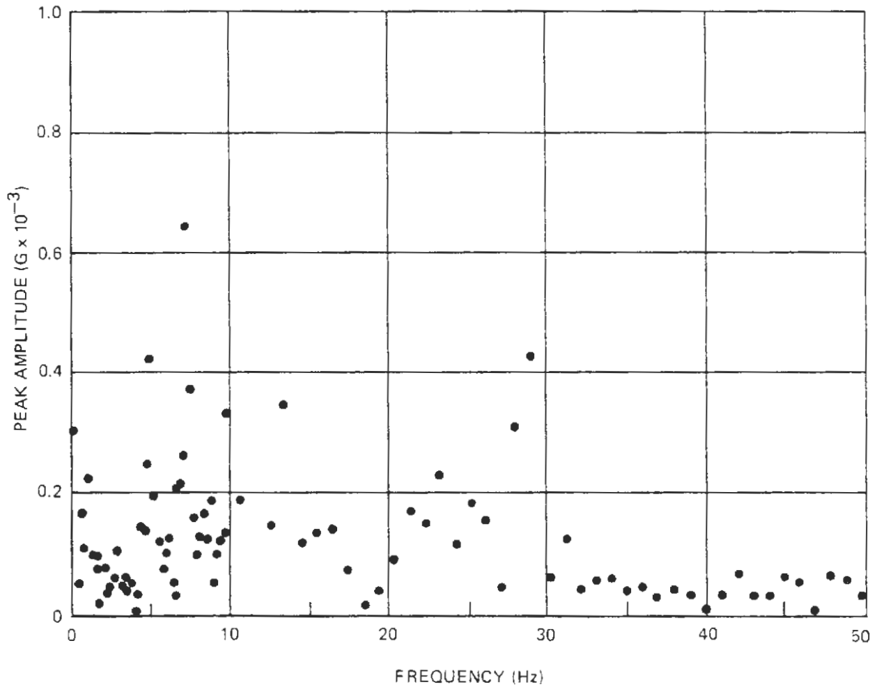
Figure A-41. Narrow-Band Spectrum Analysis – Mid Car, Longitudinal
