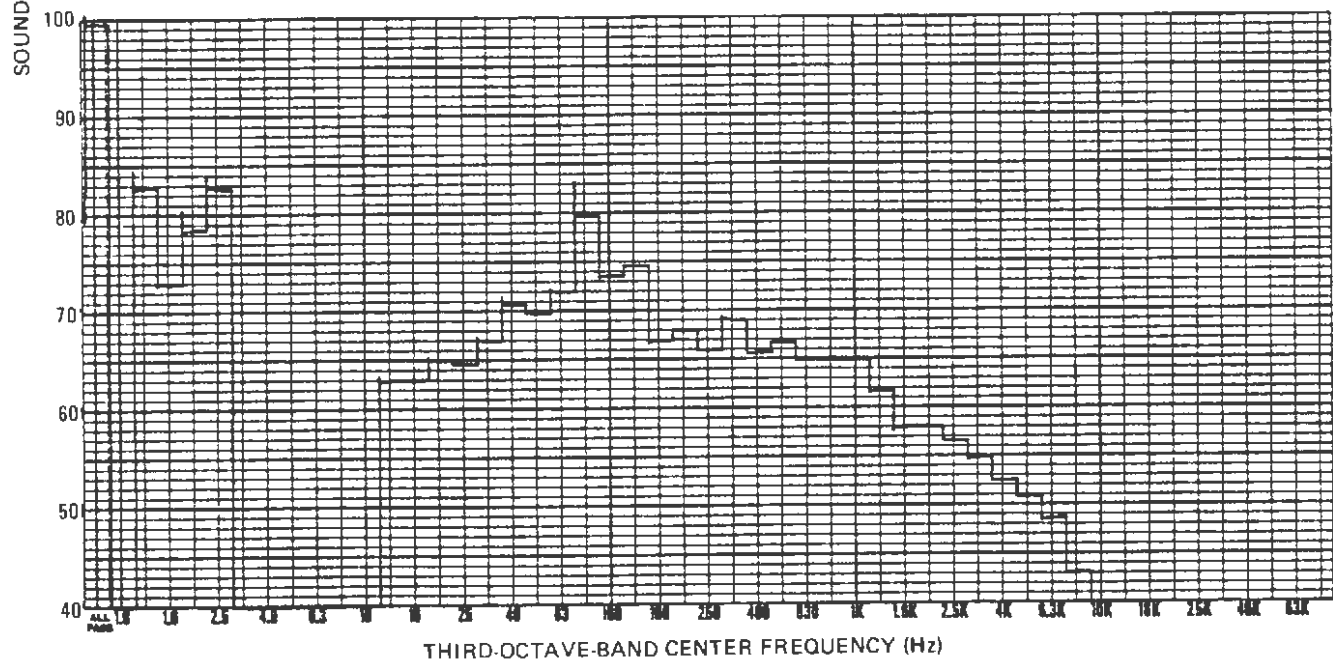
Figure 3-22. Third-Octave-Band Analysis of SFMR Interior Noise, AWO, 35 mph
