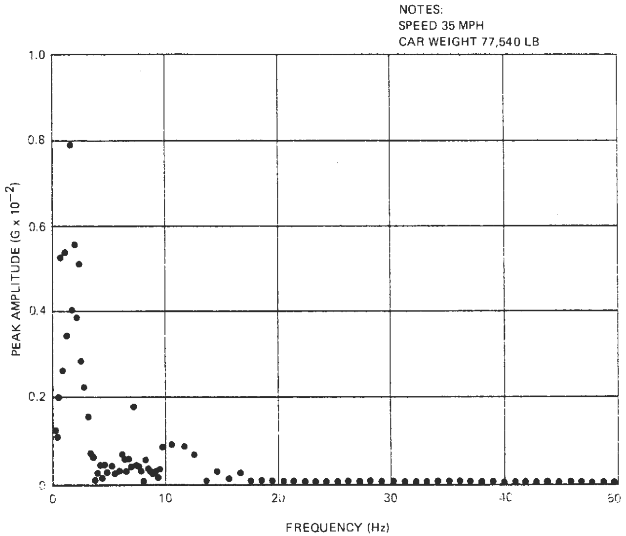
Figure 2-1. Typical Spectrum Analysis – Car Body Vertical Vibration
