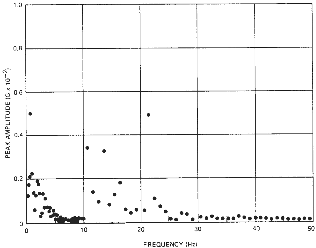
Figure A-61. Narrow-Band Spectrum Analysis – End Car, Lateral
