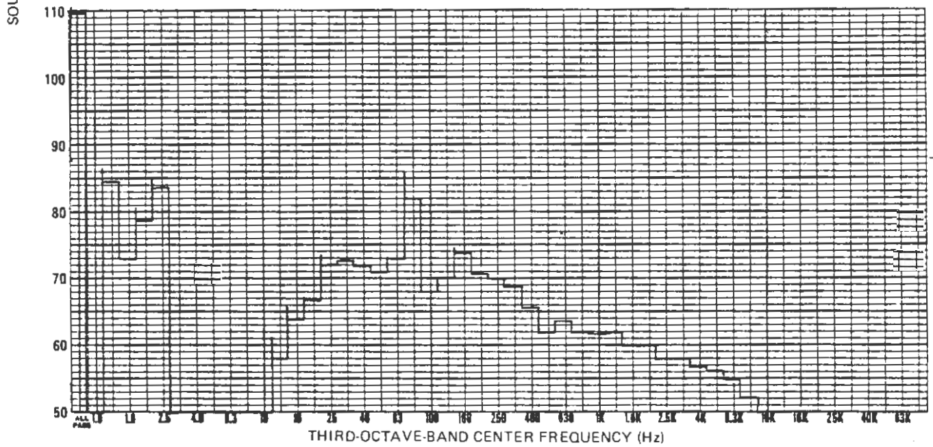
Figure 3-17. Third-Octave-Band Analysis of SFMR Interior Noise, AWO, 15 mph
