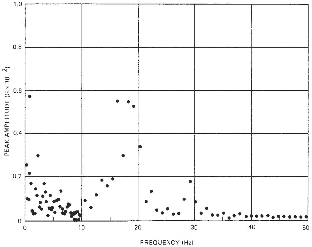
Figure A-15. Narrow-Band Spectrum Analysis — Mid Car, Lateral
