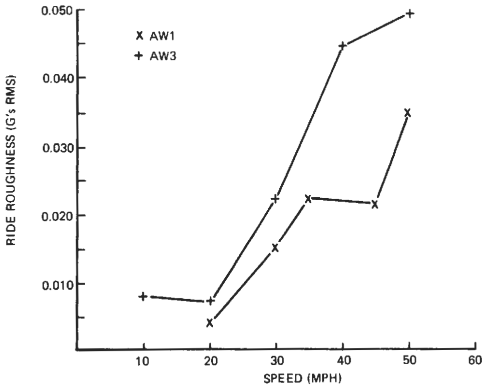
Figure 2-12. Effects of Speed and Weight on Vertical Ride Roughness, Mid Car
