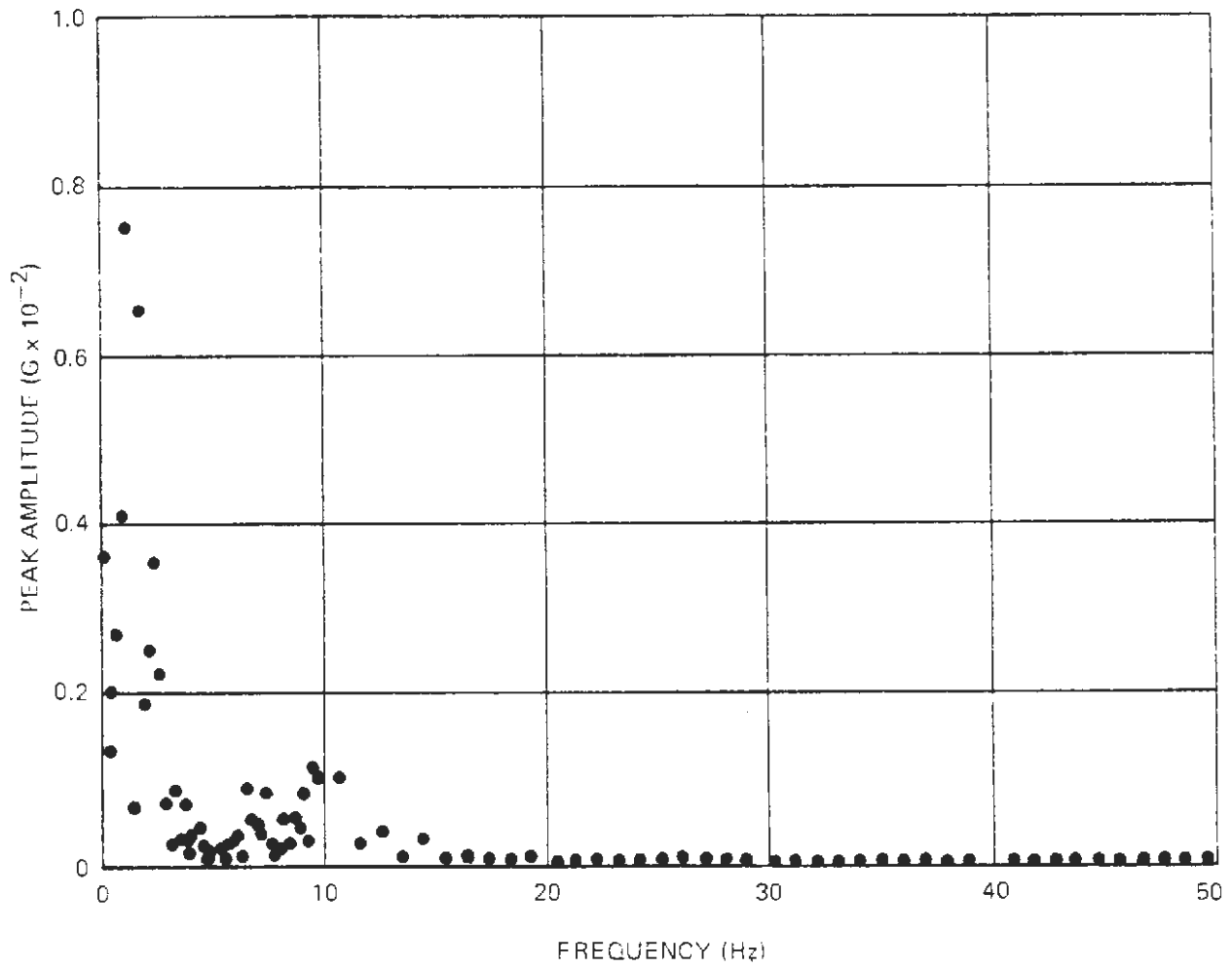
Figure A-21. Narrow-Band Spectrum Analysis – End Car, Vertical
