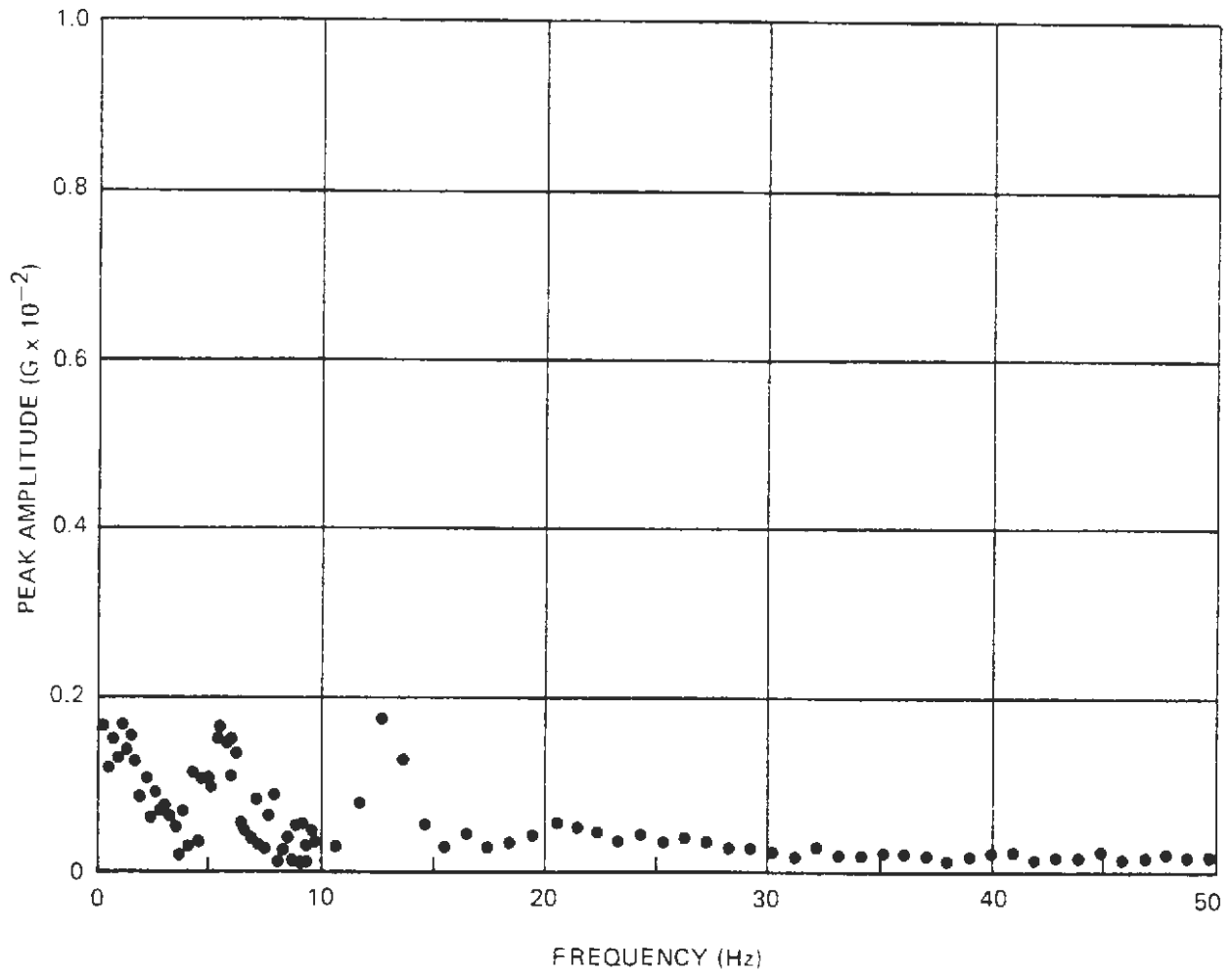
Figure A-13. Narrow-Band Spectrum Analysis -- End Car, Longitudinal
