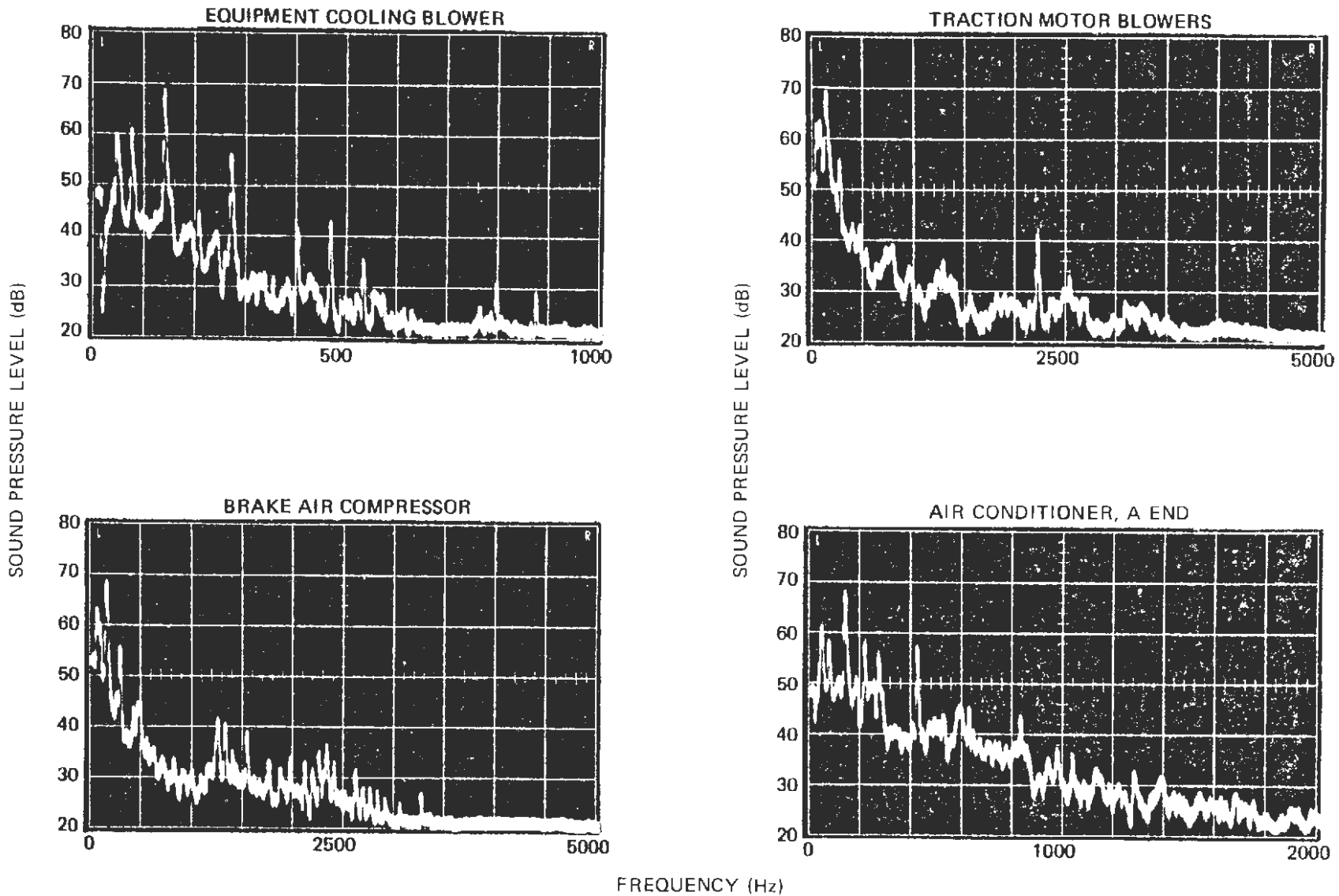
Figure 3-11. SLRV Equipment Noise, 50-Ft Wayside, Narrow-band Analysis
