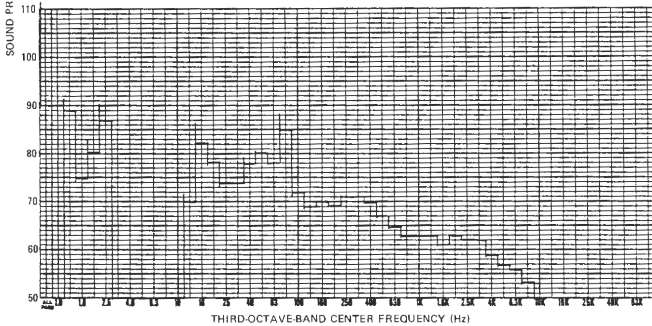
Figure 3-35. Third-Octave-Band Analysis of SFMR Interior Noise, AWO, 40 mph
