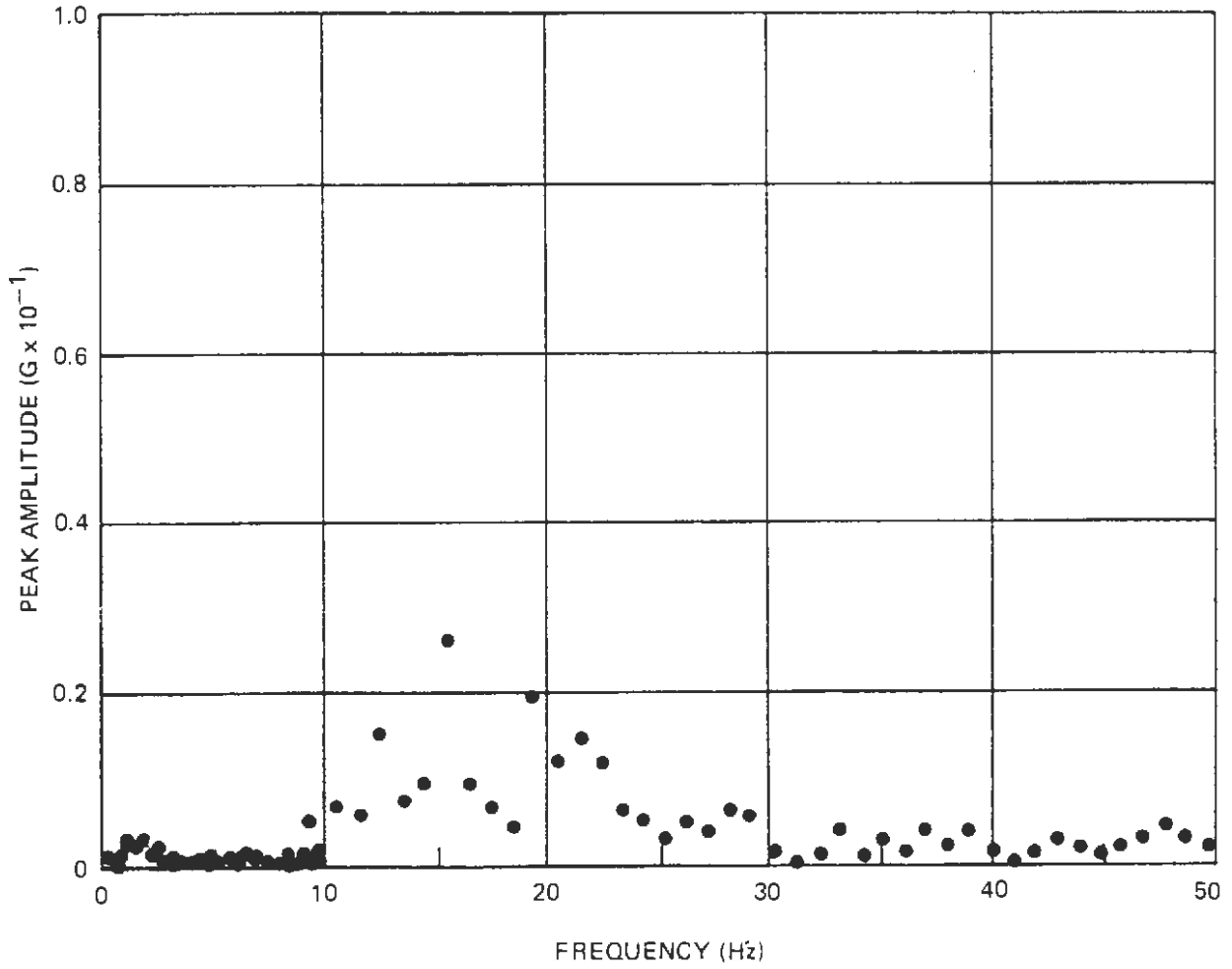
Figure A-51. Narrow-Band Spectrum Analysis – Mid Car, Vertical
