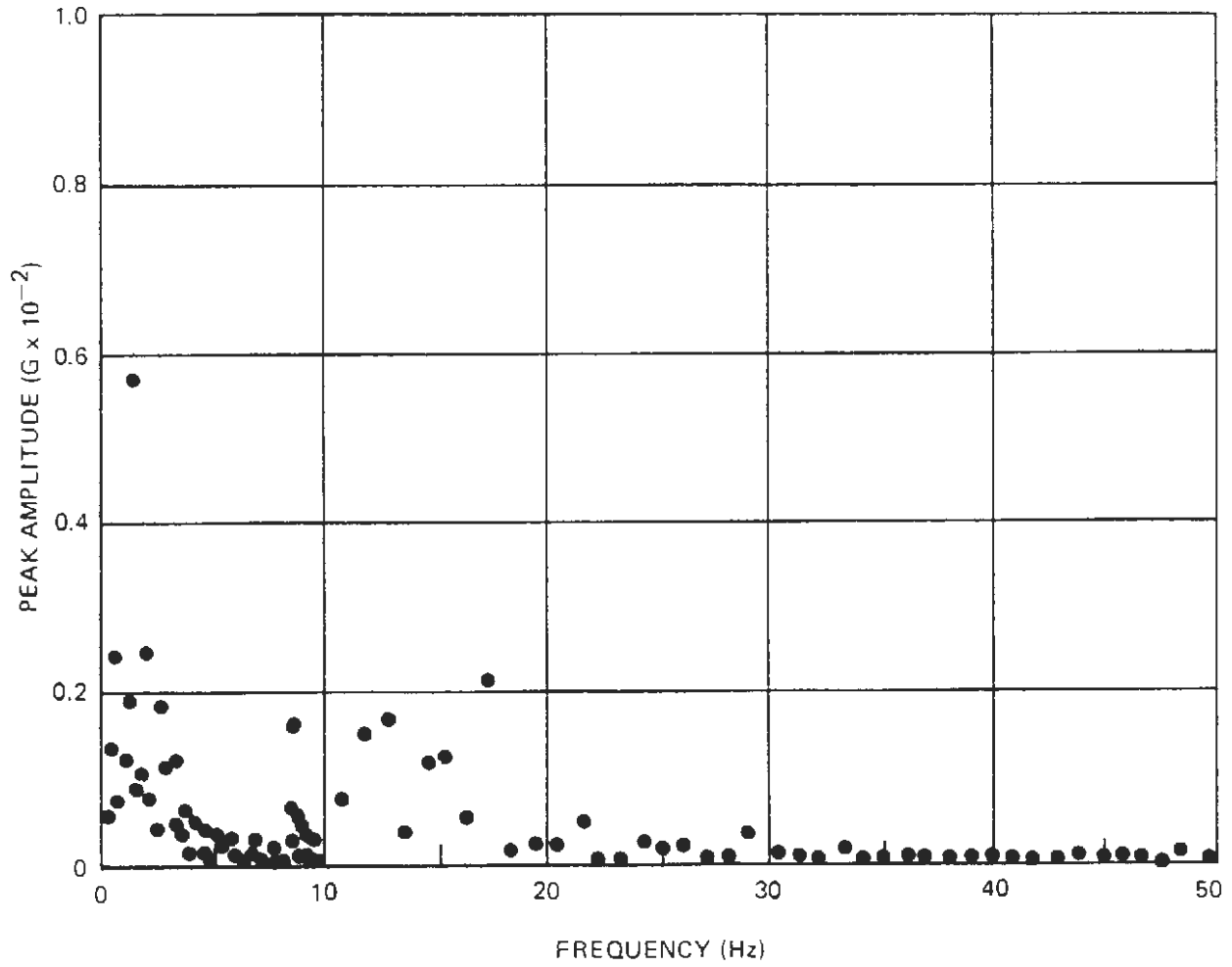
Figure A-55. Narrow-Band Spectrum Analysis – End Car, Lateral
