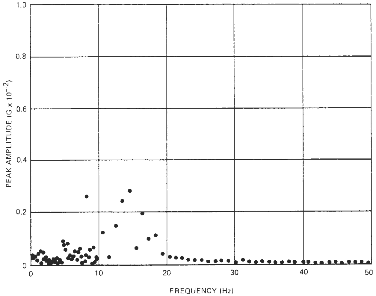
Figure A-23. Narrow-Band Spectrum Analysis – End Car, Longitudinal
