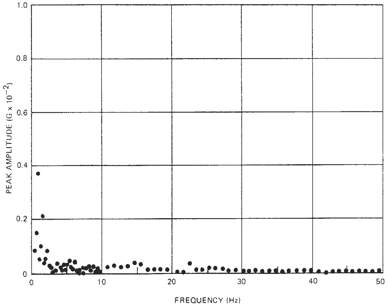
Figure A-43. Narrow-Band Spectrum Analysis — End Car, Lateral
