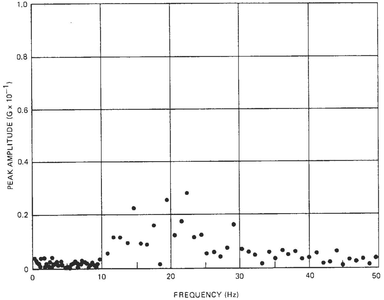
Figure A-63. Narrow-Band Spectrum Analysis – Mid Car, Vertical
