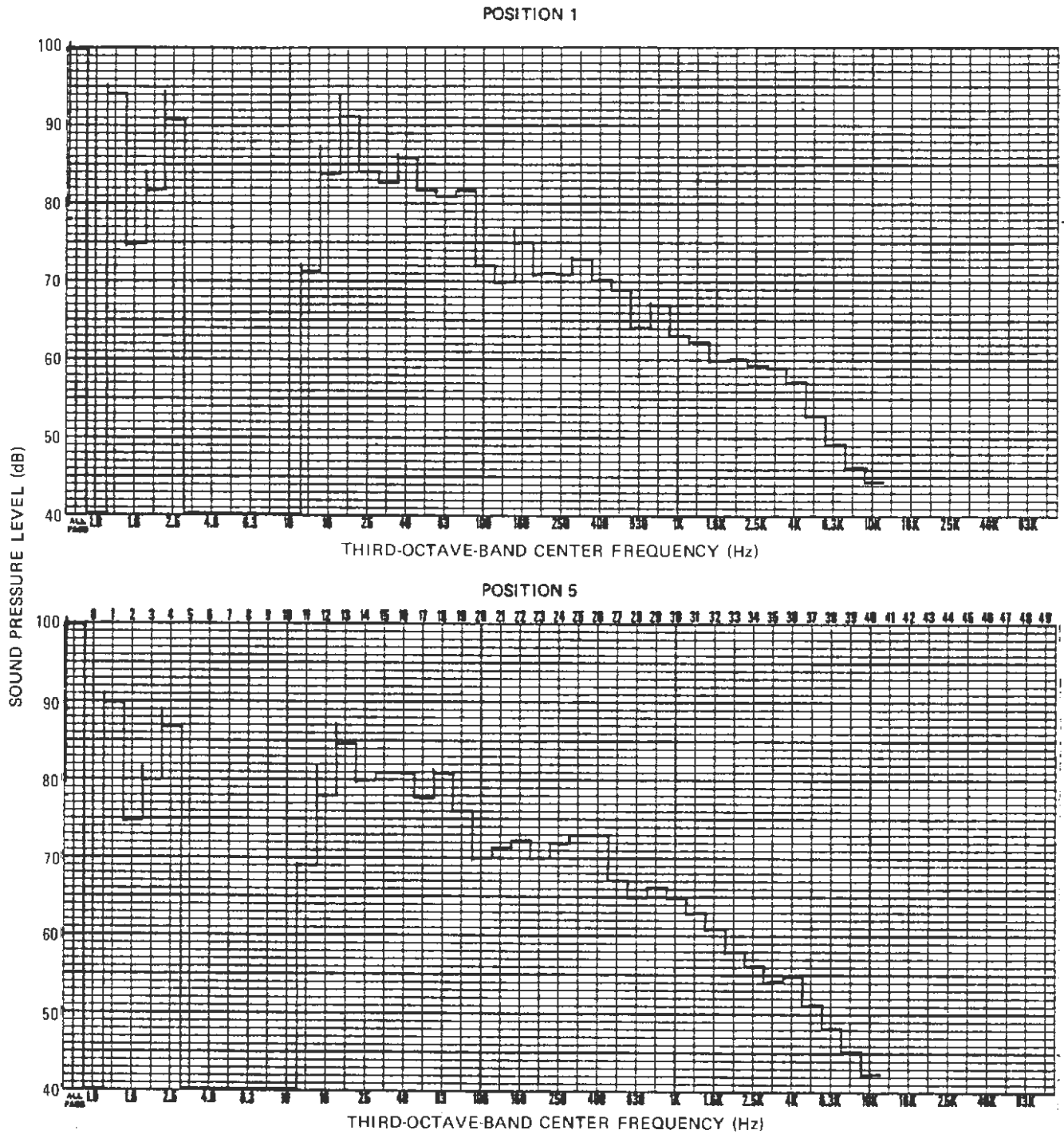
Figure 3-31. Third-Octave-Band Analysis of MBTA Interior Noise, AW0, 50 mph
