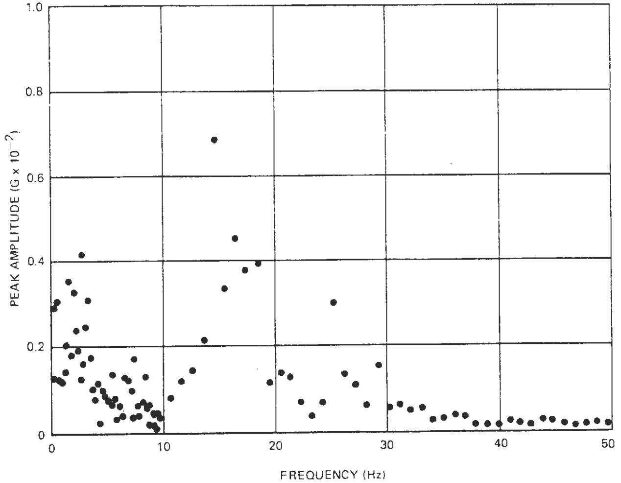
Figure A-25. Narrow-Band Spectrum Analysis – Mid Car, Lateral
