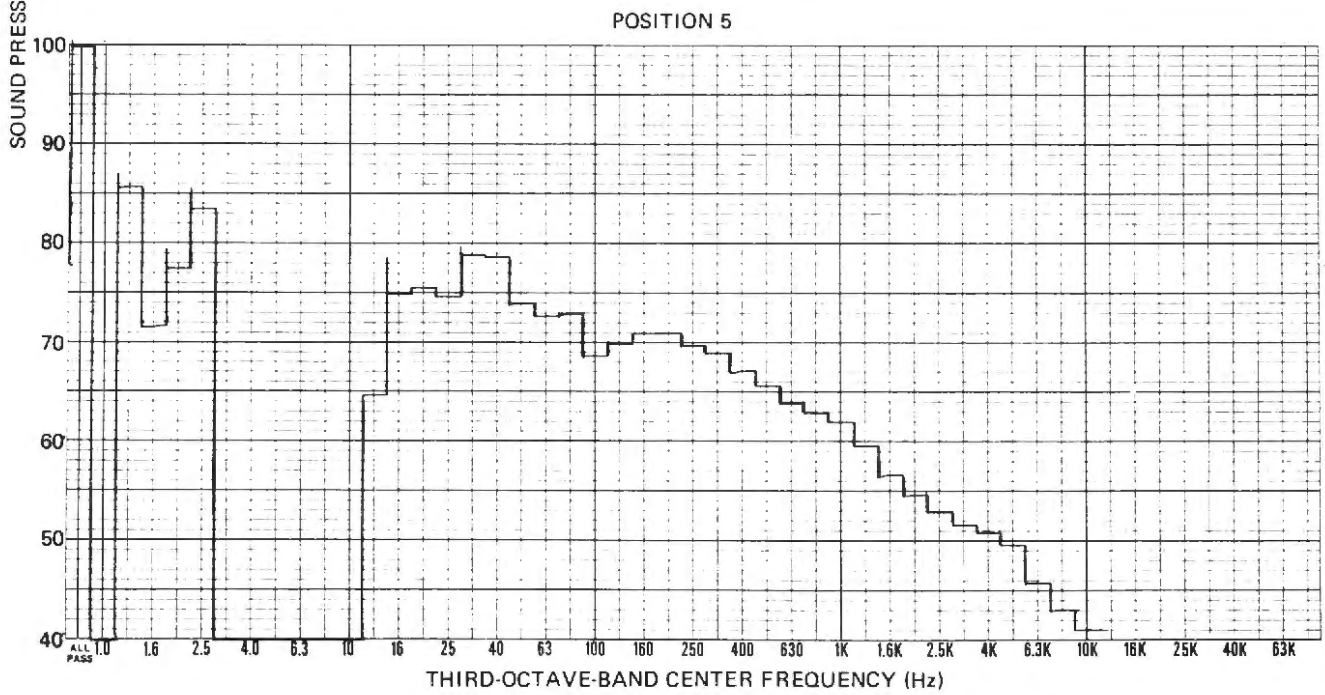
Figure 3-27. Third-Octave-Band Analysis of MBTA Interior Noise, AWO, 25 mph
