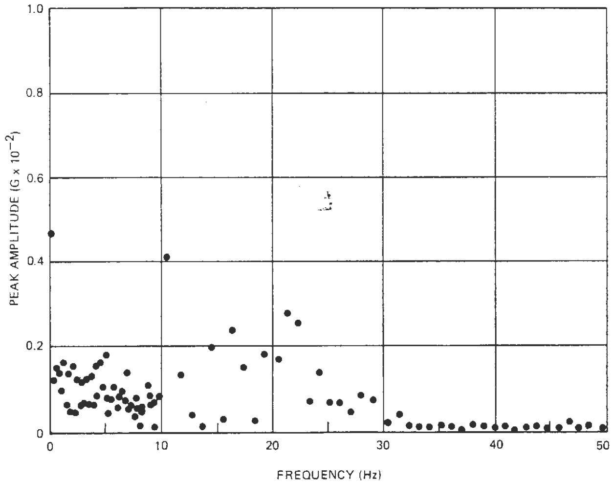
Figure A-65. Narrow-Band Spectrum Analysis - Mid Car, Longitudinal
