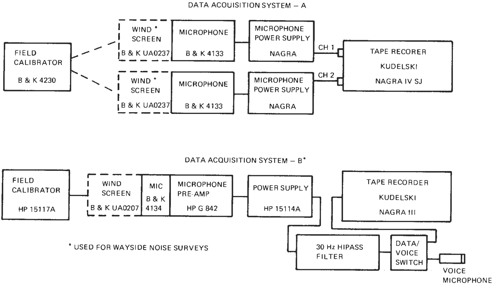
Figure 3-3. Block Diagram for Data Acquisition and Reduction Systems (Sheet 1 of 2)
