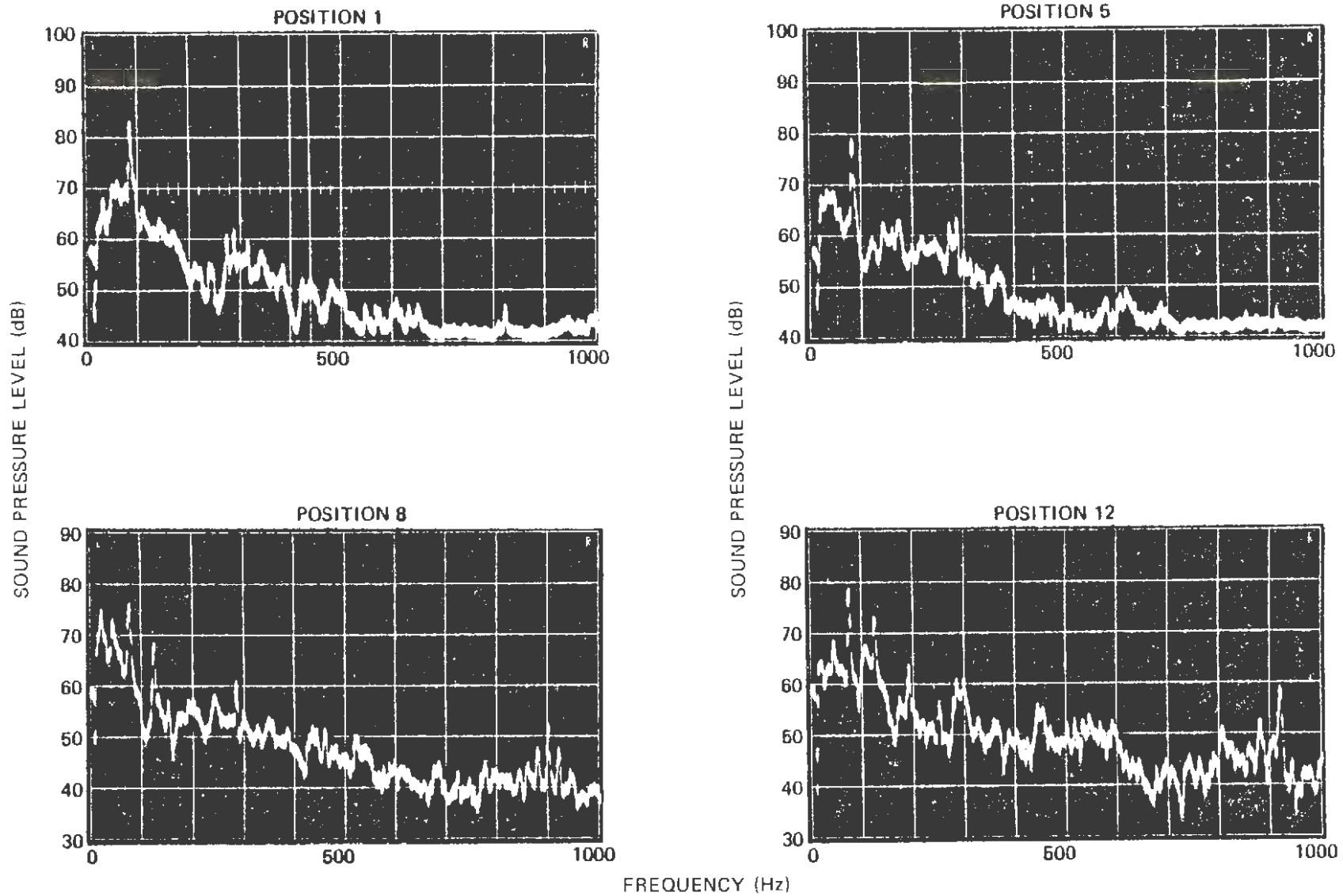
Figure 3-46. Narrowband Analysis of Interior Noise, SFMR, AW0, 35 mph
