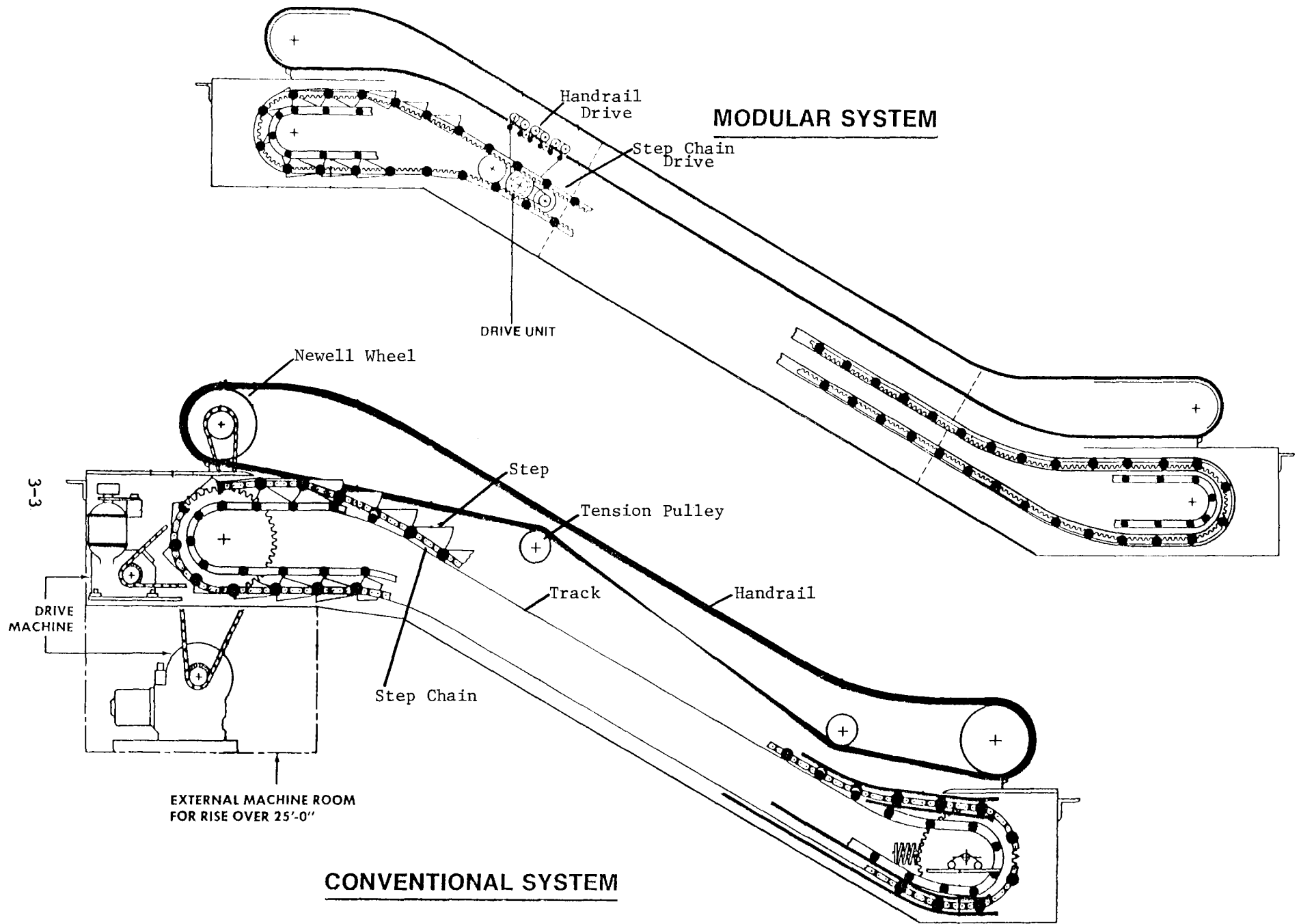
Figure 3-1. Westinghouse Escalator, Modular System (above) and Conventional System (below)
