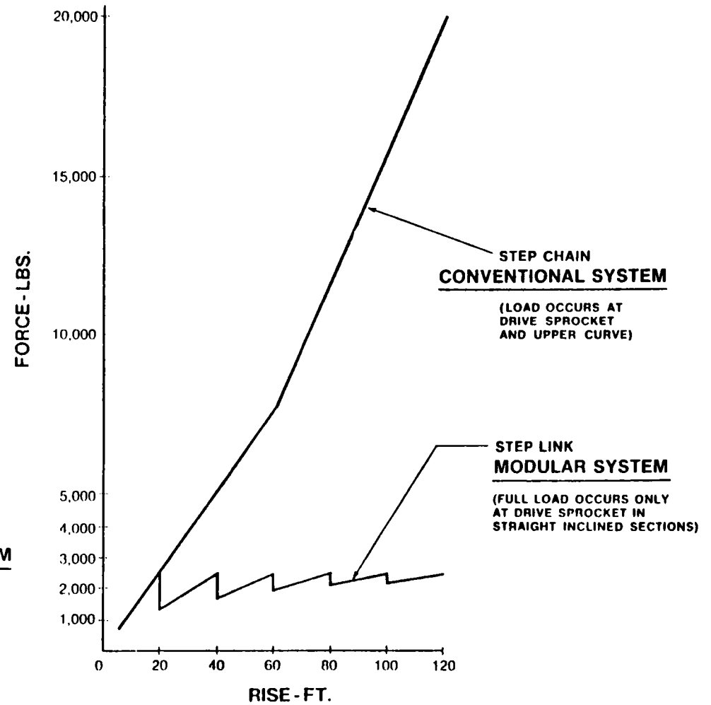
Figure 3-3. Westinghouse Modular Escalator System - Step Chain Load
