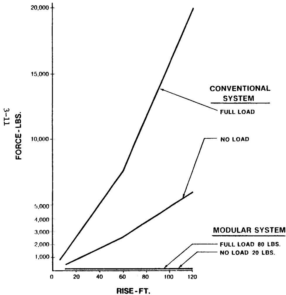
Figure 3-3. Westinghouse Modular Escalator System - Step Chain Load
