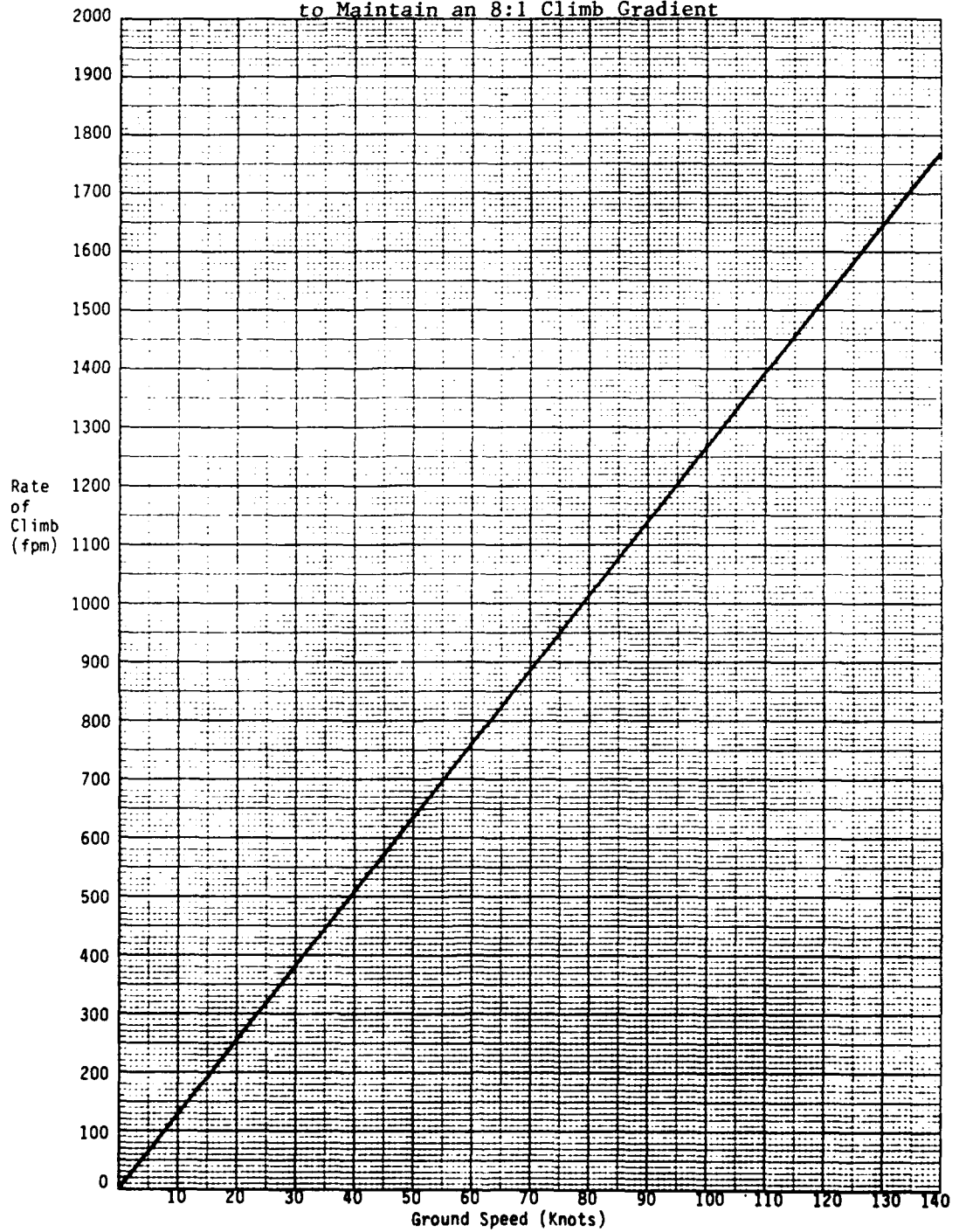
Variation of Rate of Climb with Groundspeed Necessary to Maintain an 8:1 Climb Gradient
