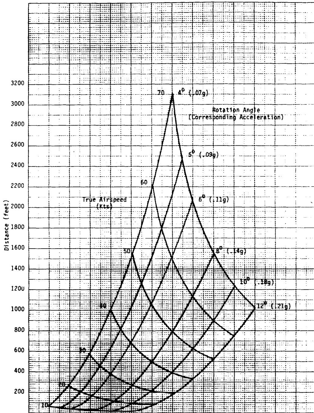
Distance Required to Accelerate to Various Airspeeds for Various Initial Rotation Angles (Acceleration Rate Assumed Held Constant Throughout Maneuver)
