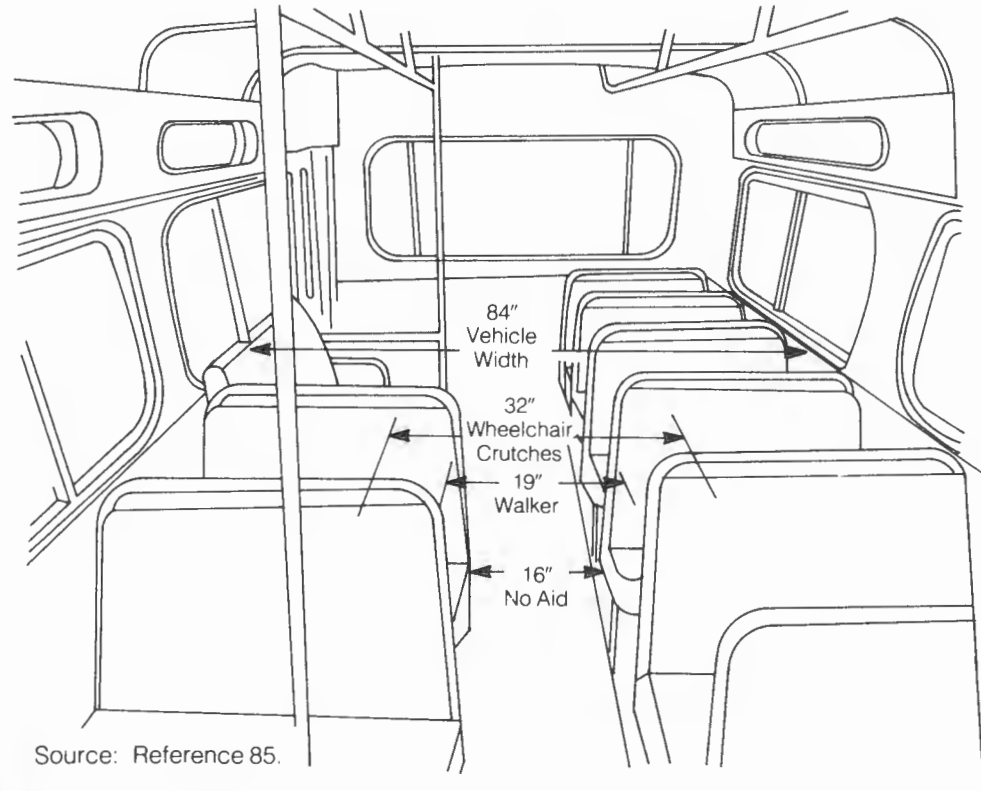
Figure 7. Aisle Space Requirements for Various Users
