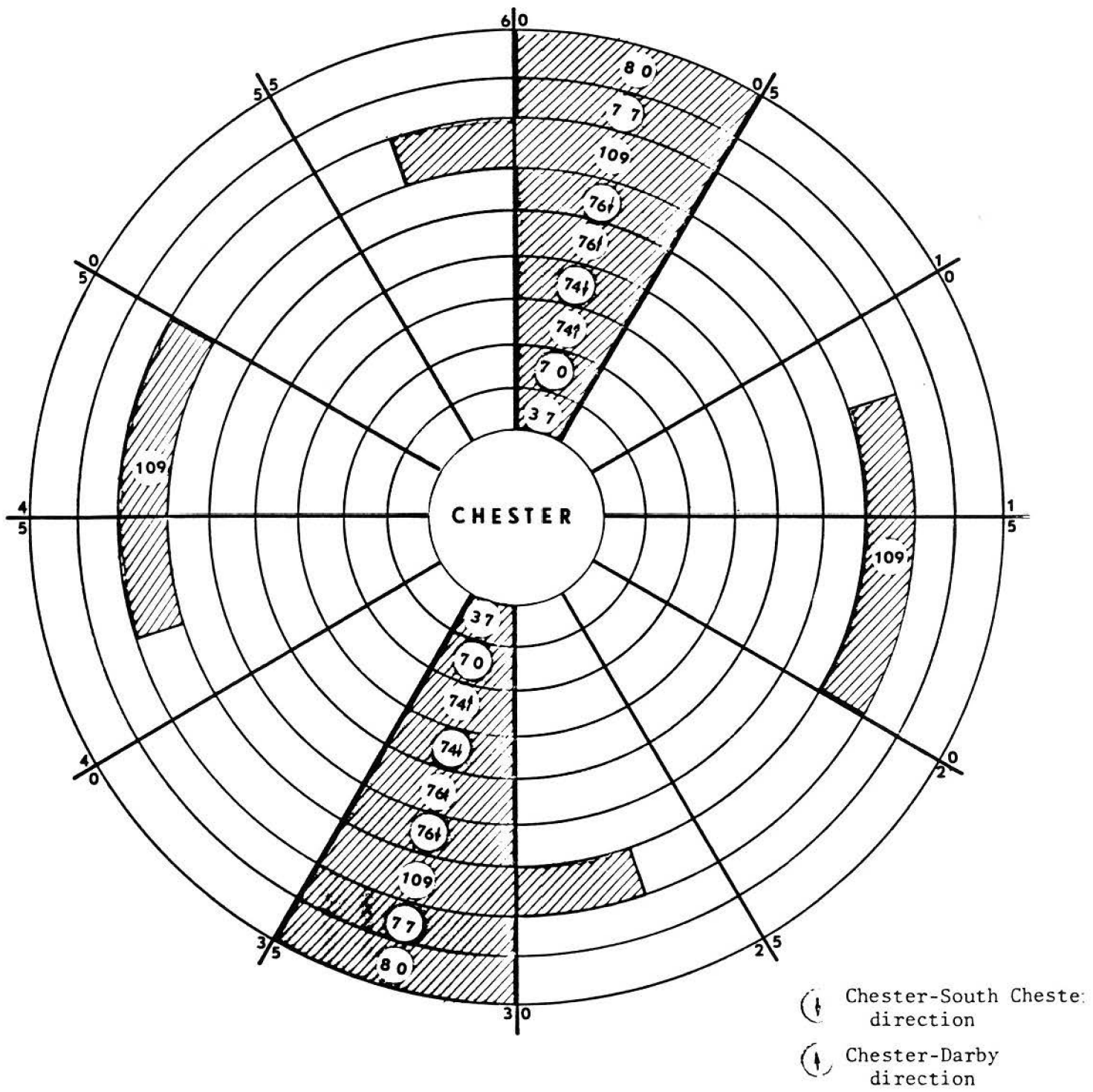
Figure 8.9 Chester transit center with fully synchronized schedules
