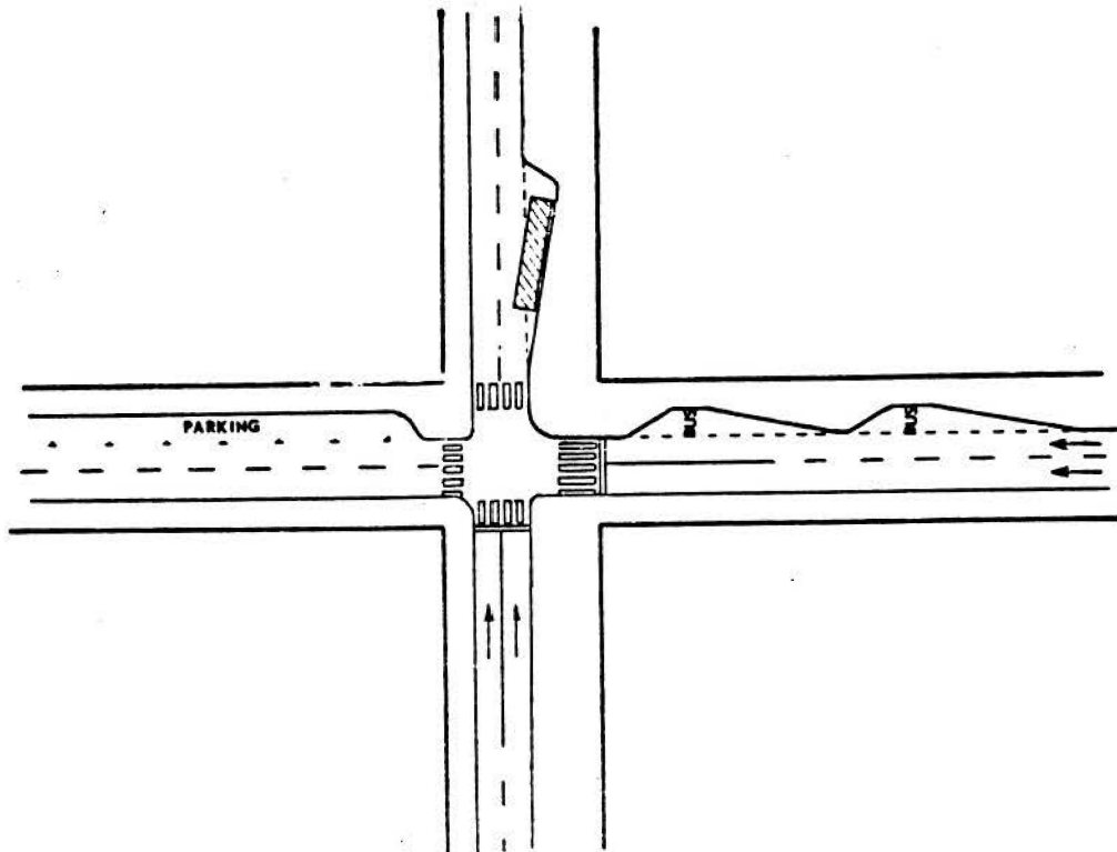
Figure 5.2 Sawtooth design of bus stops on street
