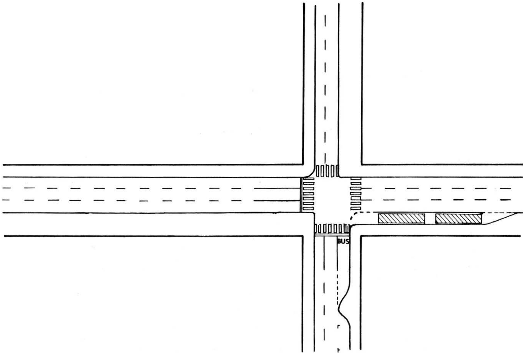
Figure 5.4 Bus bays for on-street stops
