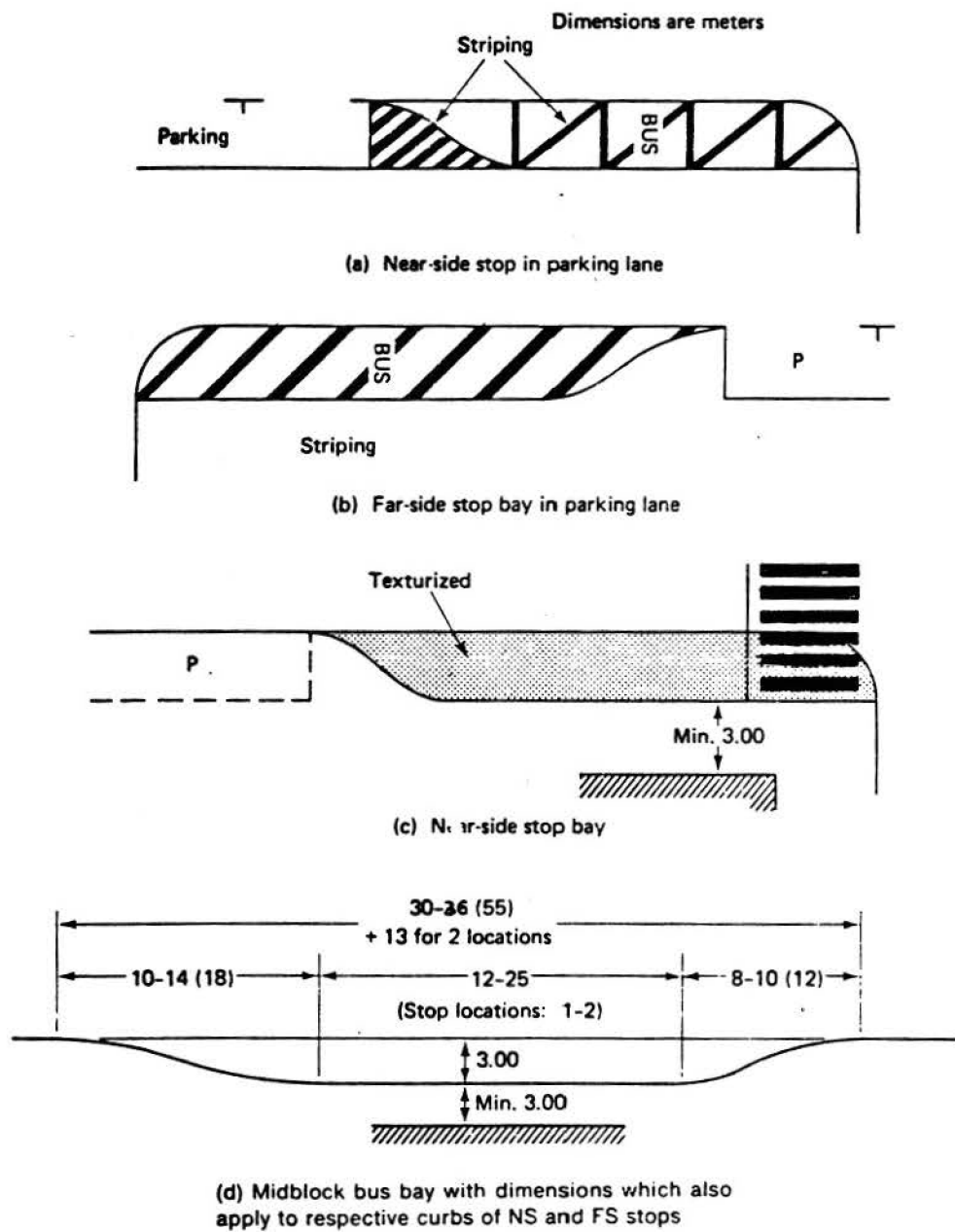
Figure 5.5 Design details and dimensions of bus bays
