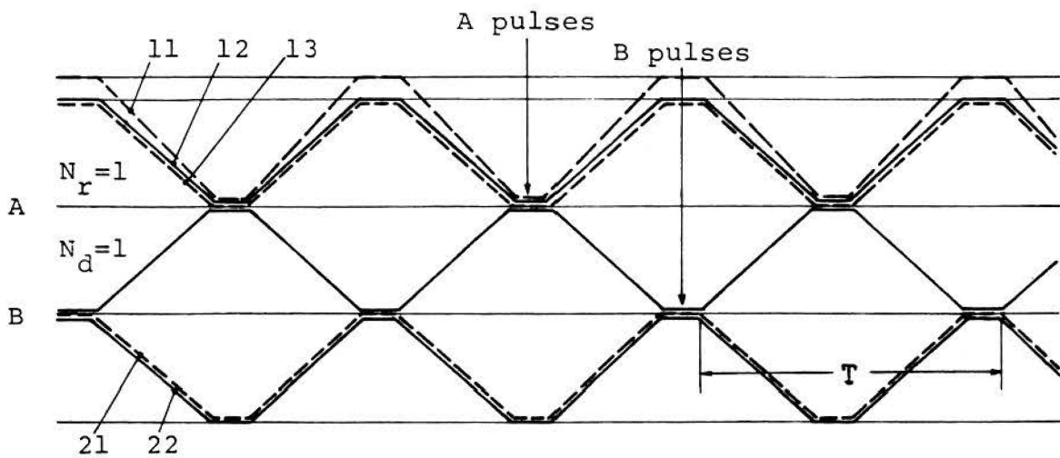
(b) Staggered pulsing between A and B focal points
