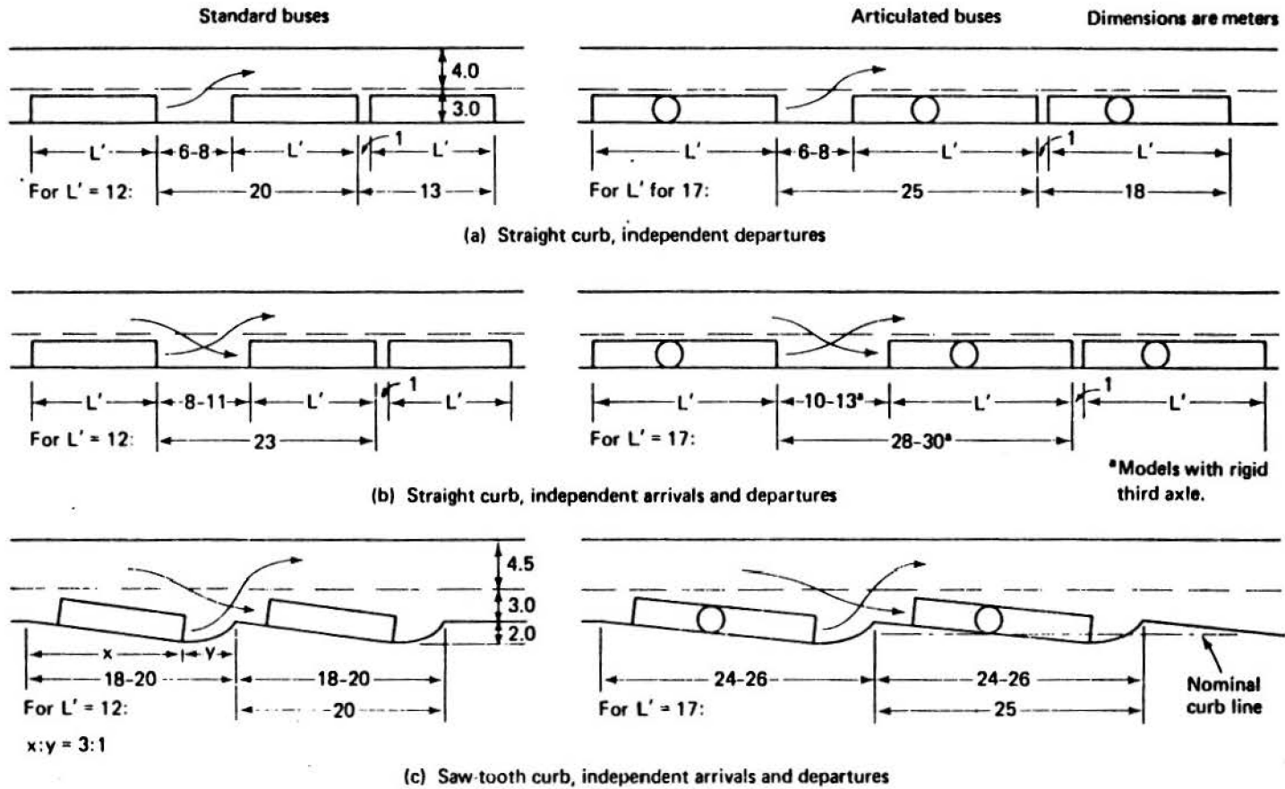
Figure 5.3 Dimensions of different types of curb bus stops
