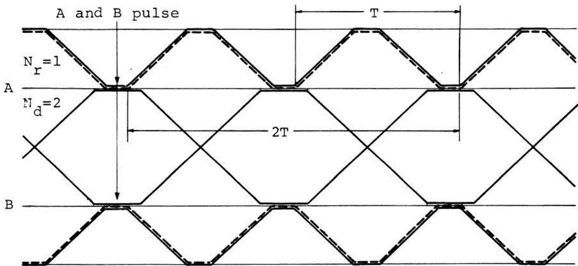
(c) Simultaneous pulsing at A and B focal points
