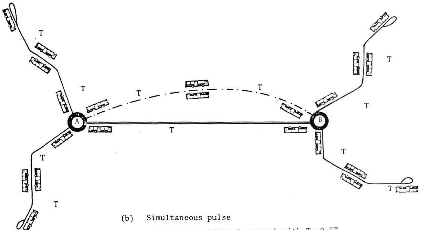
Figure 4.8 Operations of a bifocal network with T_d = 0.5T_r
