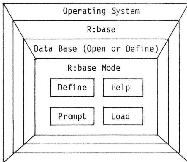
FIGURE 2-6. R:BASE TIERS
