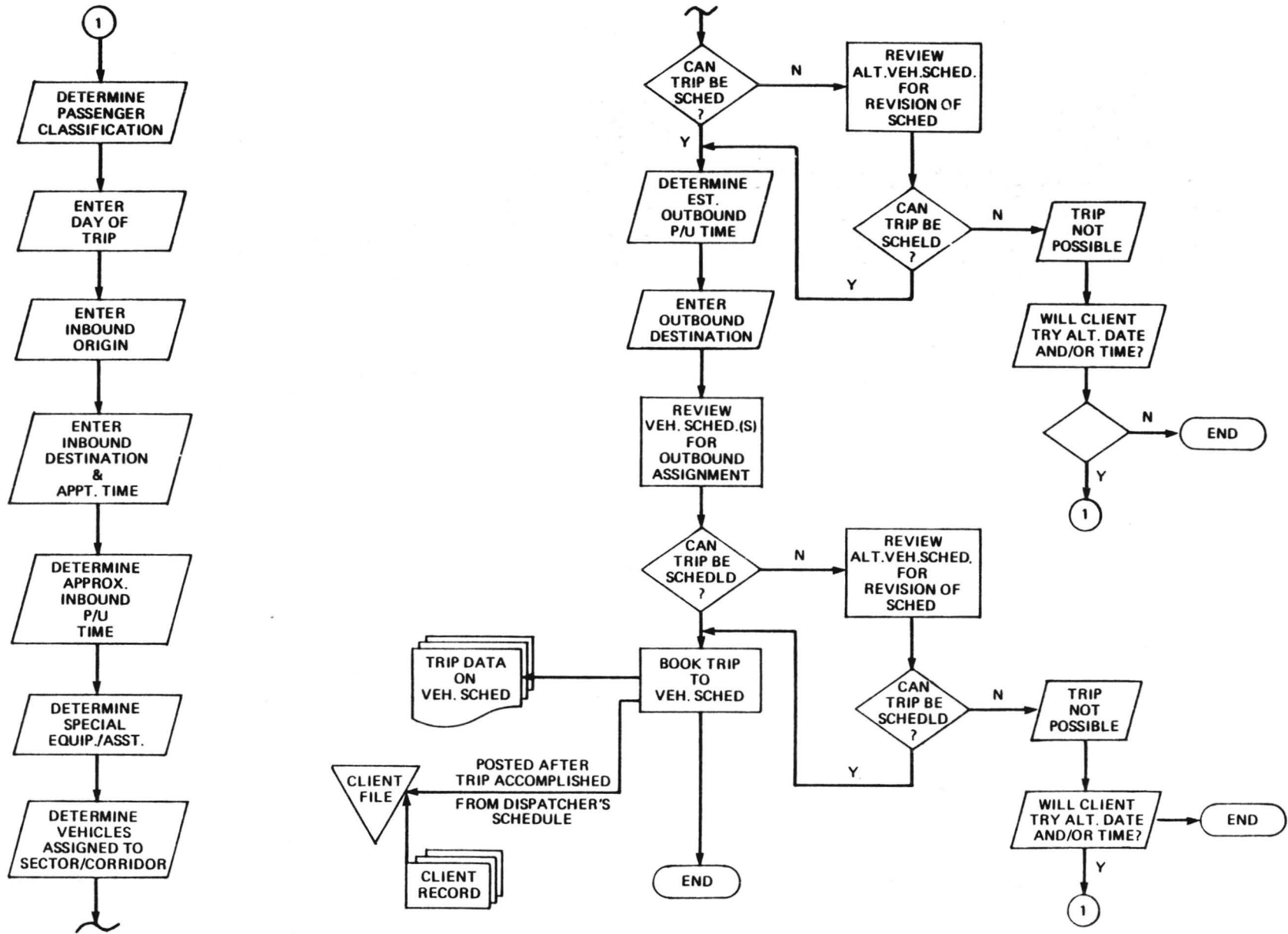
FIGURE 1-4: MANUAL PARATRANSIT SCHEDULING PROCESS
