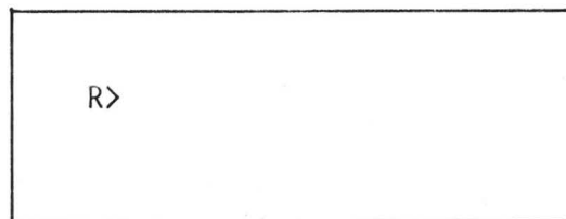
FIGURE 2-2. R:BASE PROMPT
