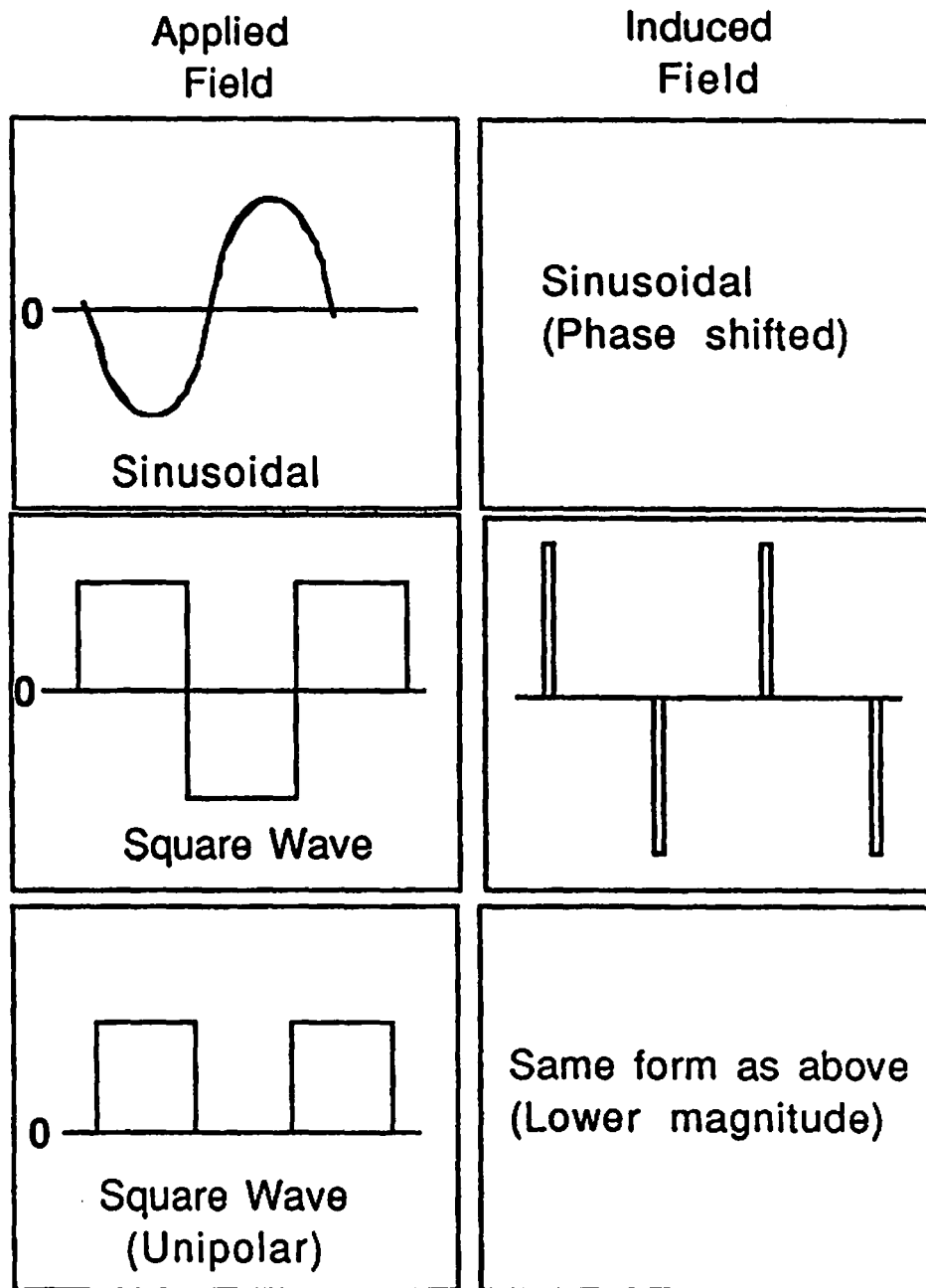
Figure 2-2. Depictions of several incident magnetic field waveforms and their corresponding induced field waveforms. No attempt is made to show relative amplitude of the induced currents. Waveforms in the right-hand panels are, to a first approximation, the first time derivative of the signals in the left-hand panels. The bipolar dc pulse waveform has been shown effective in modulation of rat pineal indoleamine metabolism in several laboratories. (Lerchl, ital. , 1991)
