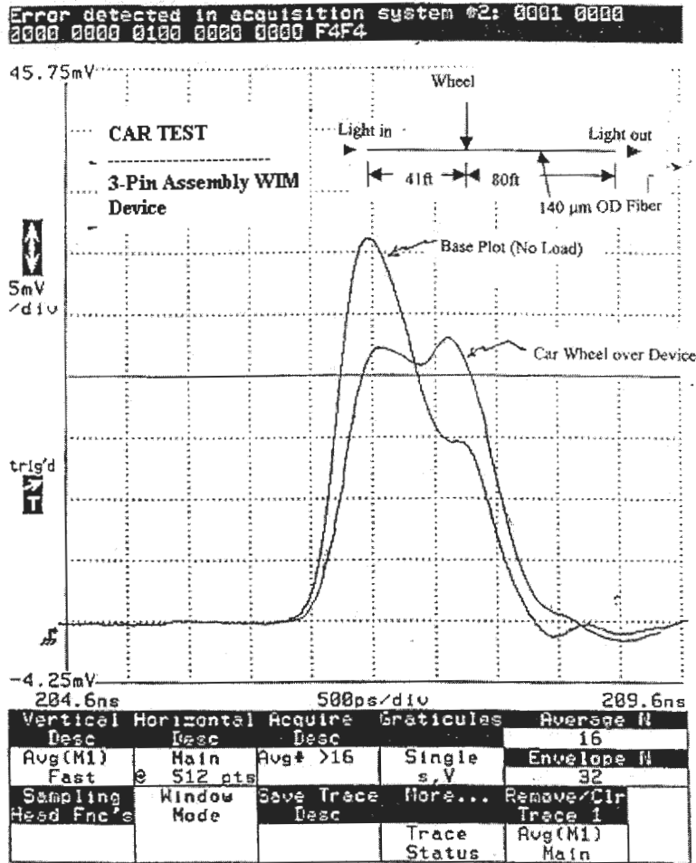
Figure 2 Oscilloscope traces from car test
