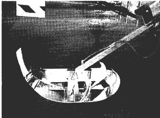
ground-coupled antenna with spacer
