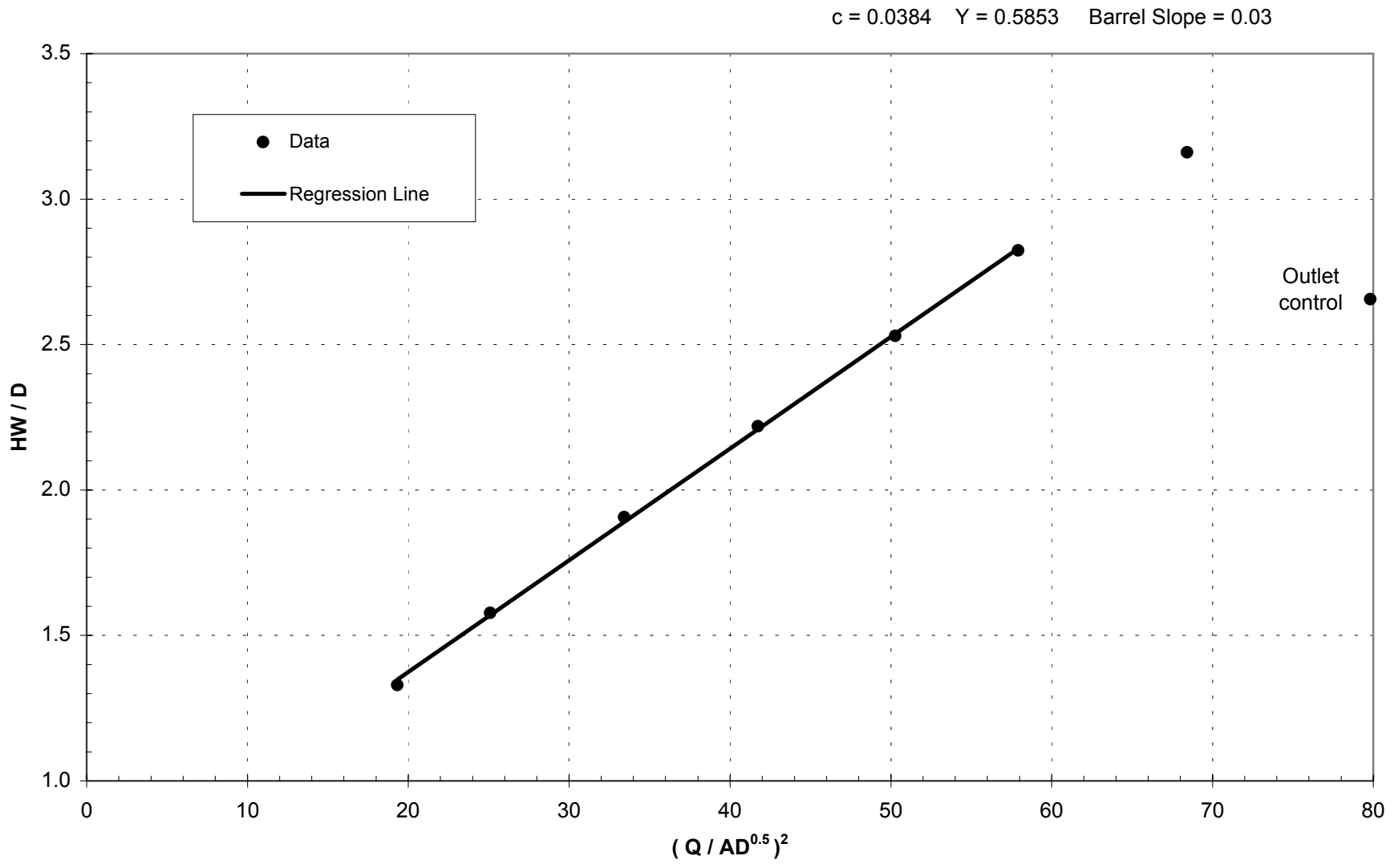
Figure 11l. Regression line vs. data, submerged conditions, culvert model 5, run 43.
