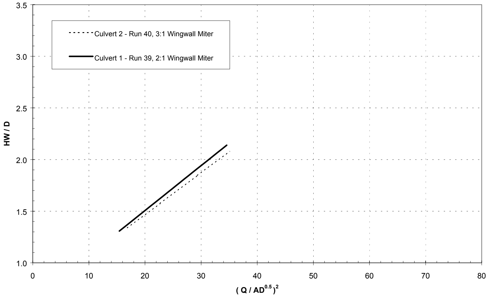
Figure 13b. Effect of wingwall miter, submerged conditions.
