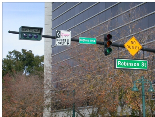
Running Way and ITS – Traffic Signage and Transit Signal Priority signal Orlando, FL
