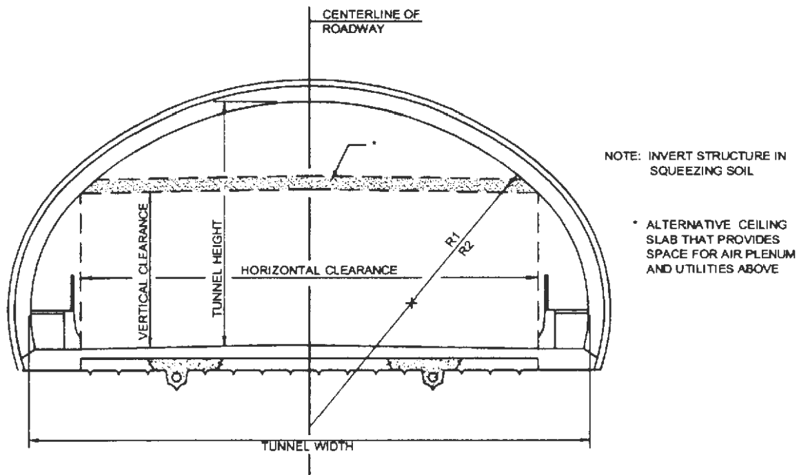
Figure 2.4 – Oval/cgg tunnel with three traffic lanes and two safety walks. Also shown is alternative ceiling slab.
