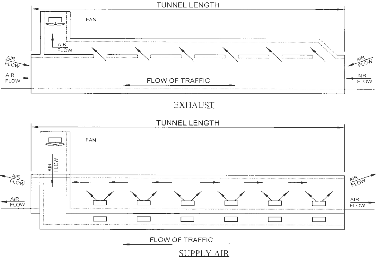
Figure 2.15 – Semi-Transverse Ventilation
