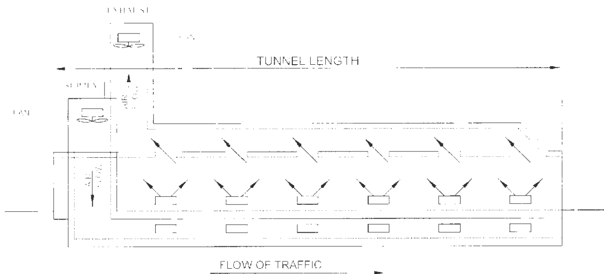
Figure 2.16 – Full-Transverse Ventilation
