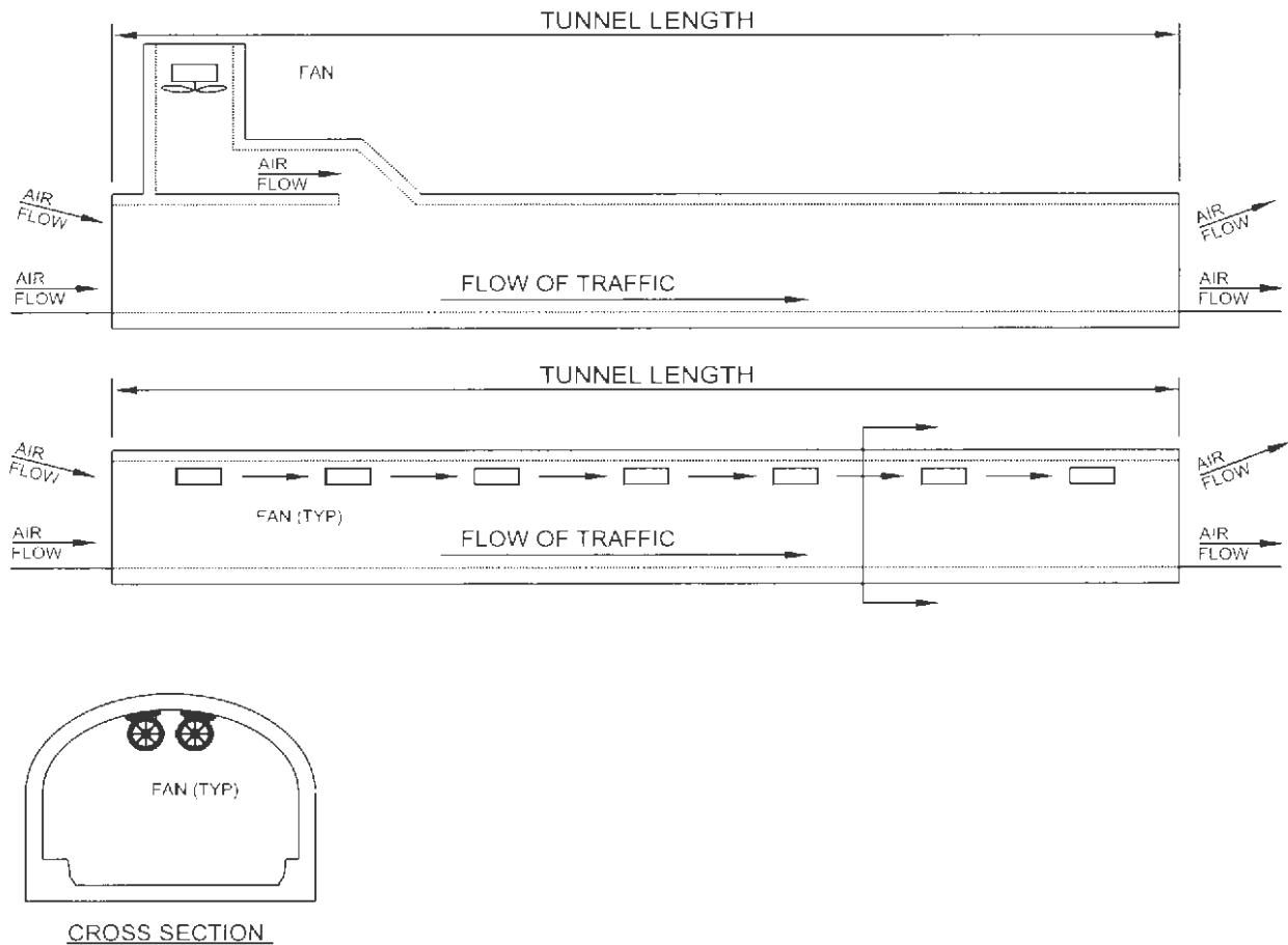
Figure 2.14 – Longitudinal Ventilation
