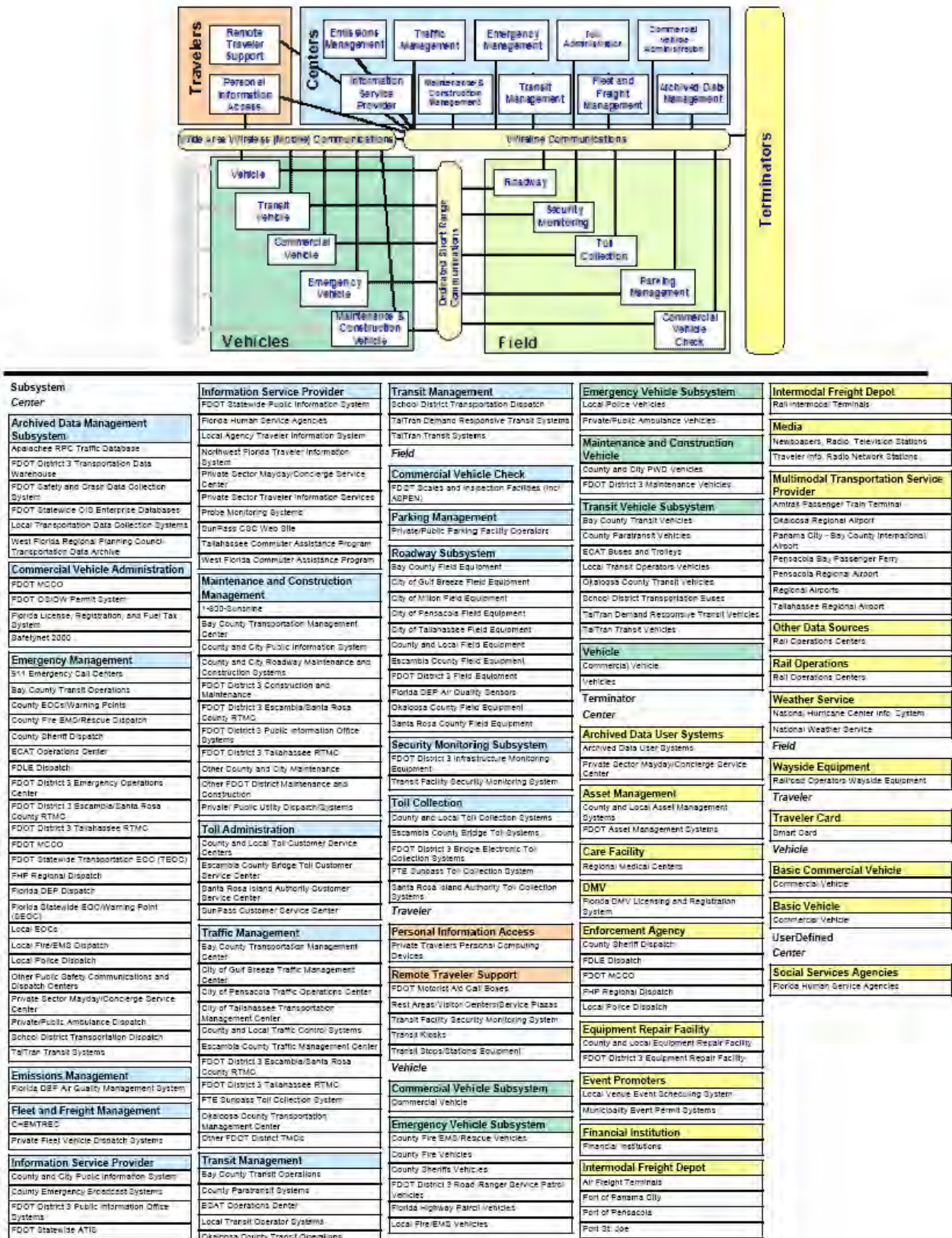
Figure 8: Florida DOT District 3, Extended Subsystem Diagram
