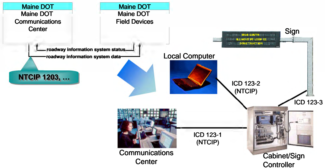
Figure 53: Example DMS Project Architectural Design
