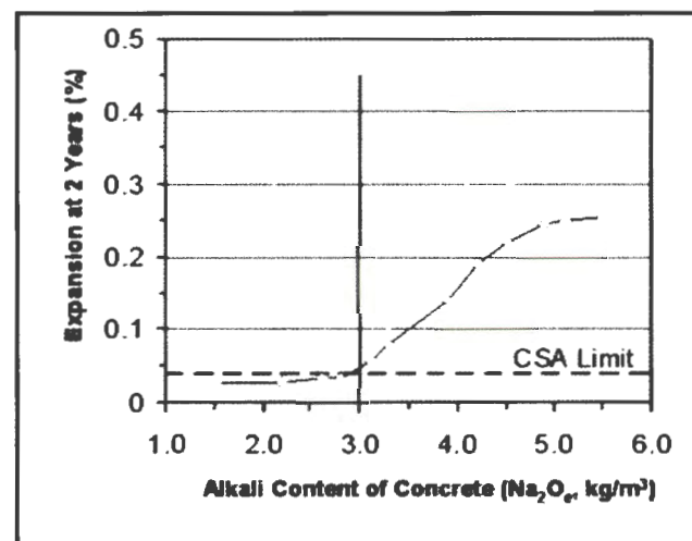
Figure 13. Effect of the alkali content of concrete on the expansion of prisms.
