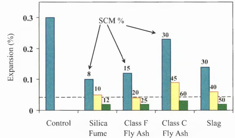
Figure 14. Effect of SCM on the expansion of concrete (using concrete prism test).
