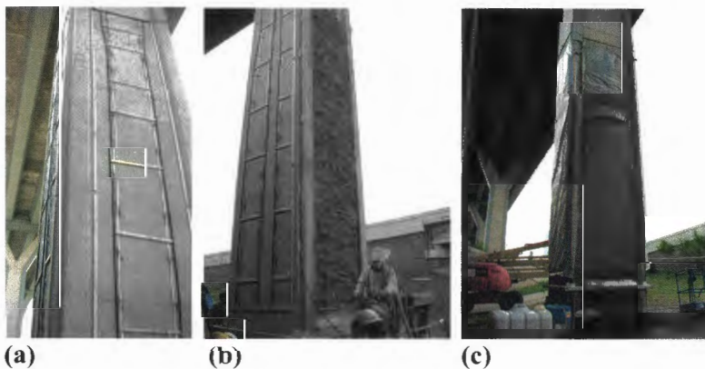
Figure 24. Electrochemical lithium treatment process. (a) irrigation tubes, wood splices, and metal strips are placed on the column. The metal strips are attached to titanium mesh that runs inside holes drilled into the sides of the column. (b) A cellulose layer is applied to the side of the column, and (c) plastic sheeting is placed on all sides of the column. The gutters under the sheeting collect excess lithium for reuse.
