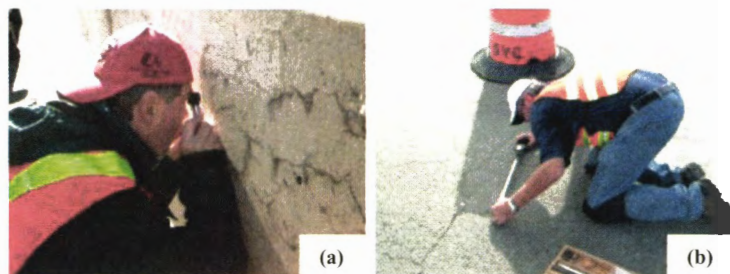
Figure 27. Monitoring techniques—(a) crack mapping of a barrier wall and (b) measuring length changes on concrete pavement with a DEMEC gauge.
