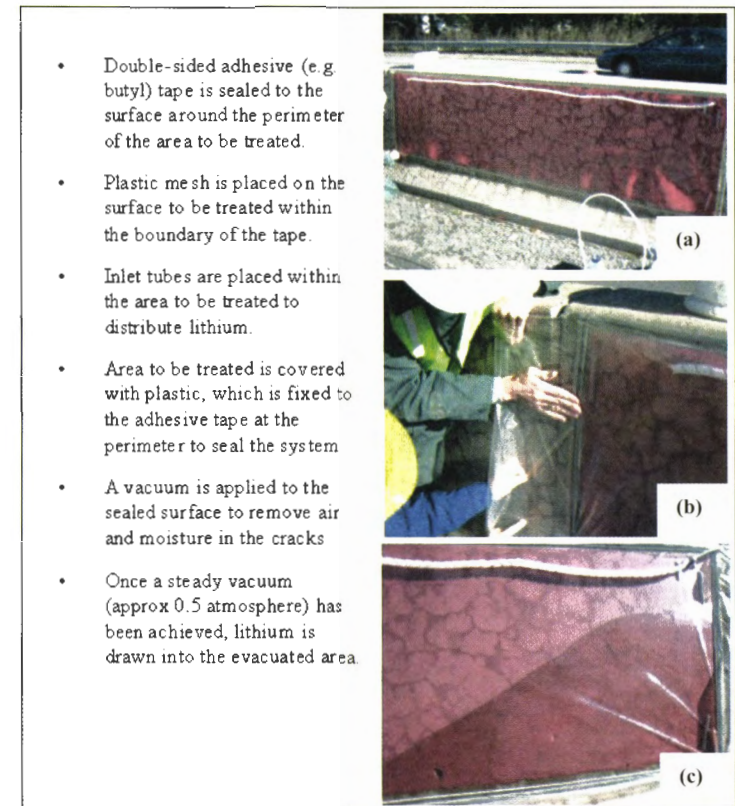
Figure 25. Typical vacuum impregnation setup.
