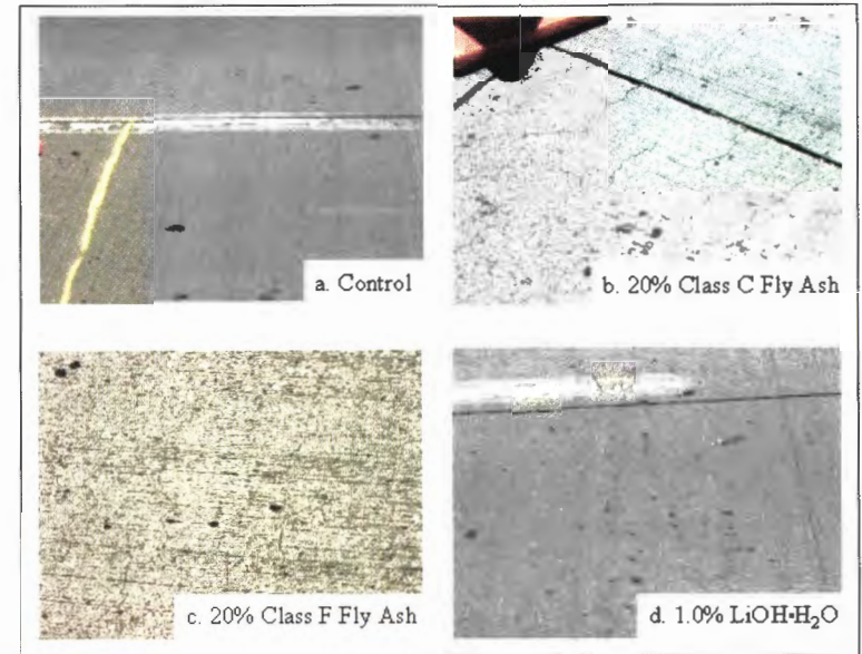
Figure 18. Photographs of 12-year-old pavement sections reactive aggregate from Placitas pit in Albuquerque, NM.
