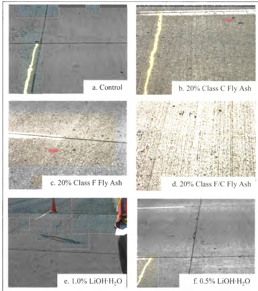
Figure 17. Photographs of 12-year-old pavement sections reactive aggregate from Shakespeare pit in Albuquerque, NM (photos taken in 2004).
