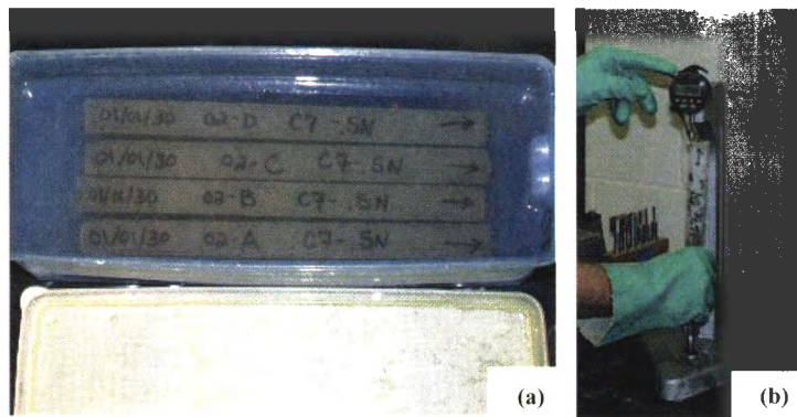
Figure 12. Accelerated mortar bar test (ASTM C1260): (a) view from the top of four rectangular concrete samples, under water in a blue rectangular container; (b) measuring a concrete sample for length change using a digital comparator.
