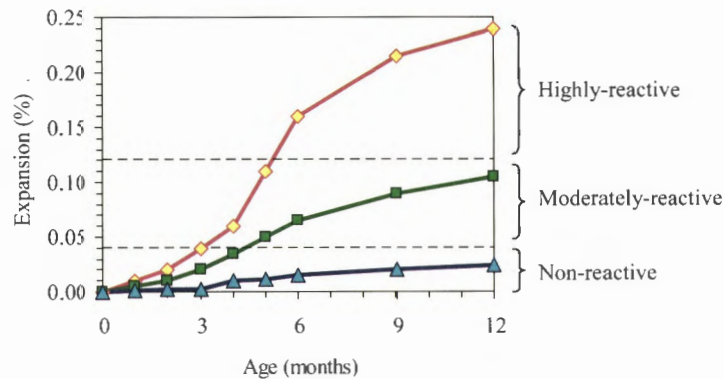
Figure 11. Concrete prism test—length change measurements (ASTM C1293) 1 .
