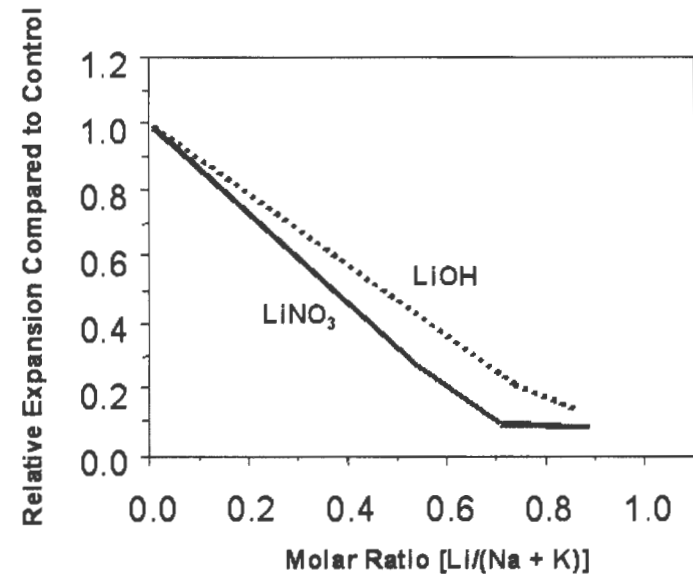
Figure 16. Relative expansion of concrete prisms (ASTM C1293) containing lithium compounds and reactive siltstone aggregate (Thomas et al., 2000).
