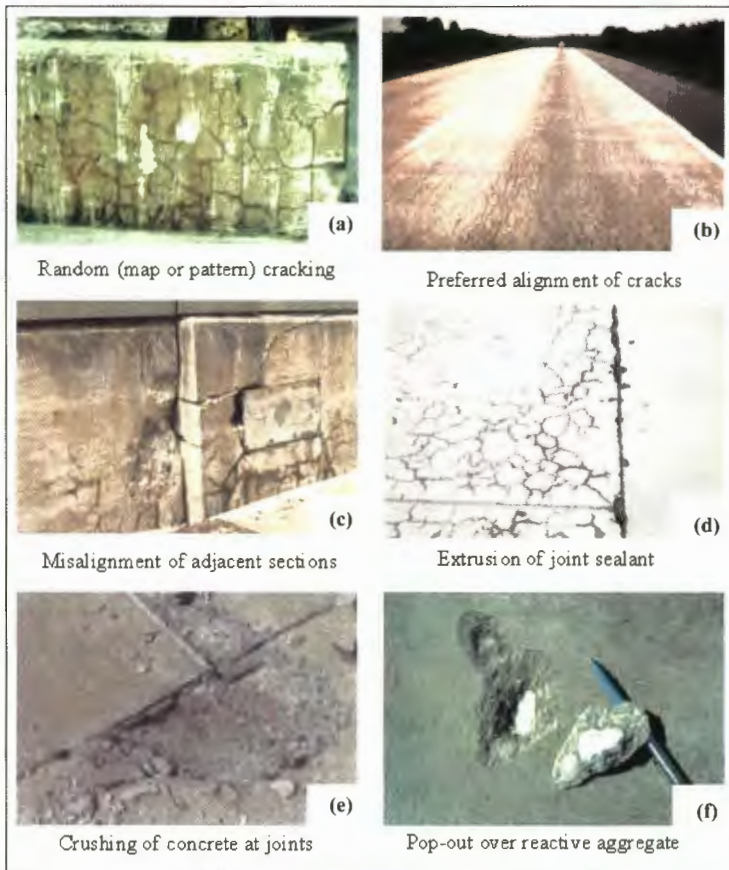
Figure 9. Typical symptoms of ASR.
