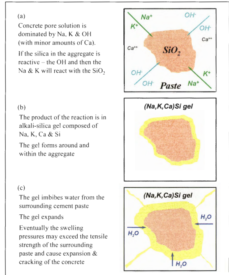
Figure 6. Sequence of alkali-silica reaction (ASR) in concrete.
