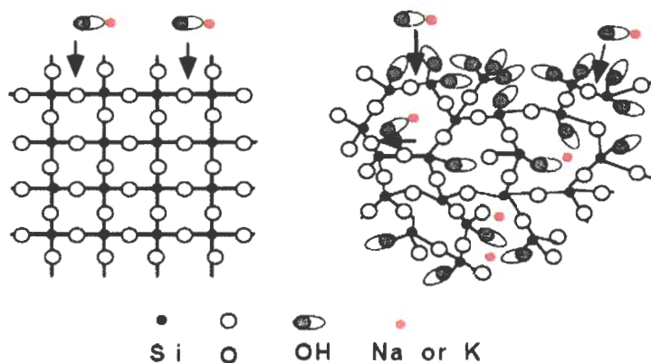
Figure 7. Schematic showing difference in crystal structure of quartz (left) and opal (right).
