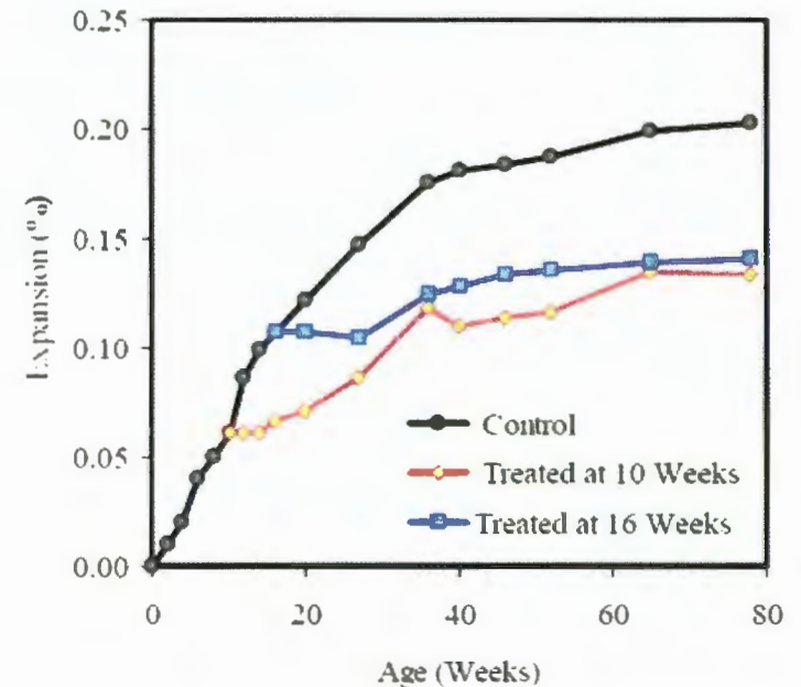
Figure 19. Expansion of concrete prisms after treatment with lithium at 10 weeks (expansion = 0.061 percent) and 16 weeks (expansion = 0.107 percent) (Thomas and Stokes, 2004).
