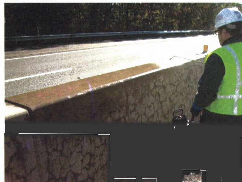
Figure 21. Spraying 30-percent \text{LiNO}_3 solution with handheld spray applicator on barrier wall near Leominster, MA.
