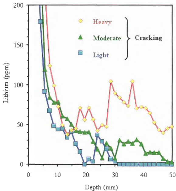
Figure 22. Lithium concentration profiles for concrete pavement after six treatments (at approximately 6-month intervals) of 0.24 L/m 2 (6 gal/1000 ft 2 ) (Stokes et al., 2002).
