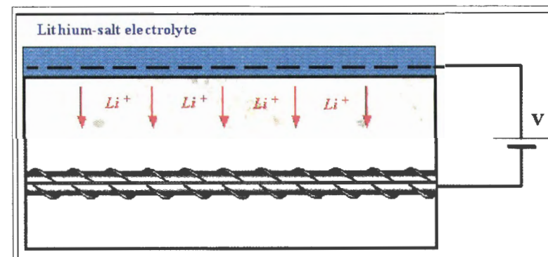
Figure 23. Electrochemical lithium impregnation.
