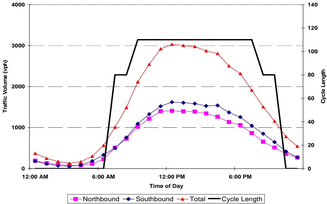
Figure 7-3 Traffic Volumes Summary Used to Determine Weekend Time of Day Plans
