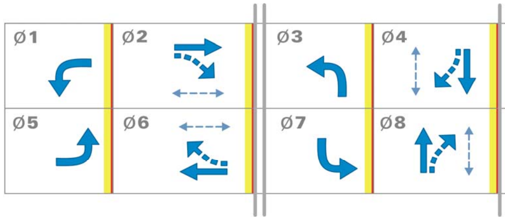
Figure 4-7 Ring-and-barrier diagram showing protected phasing
