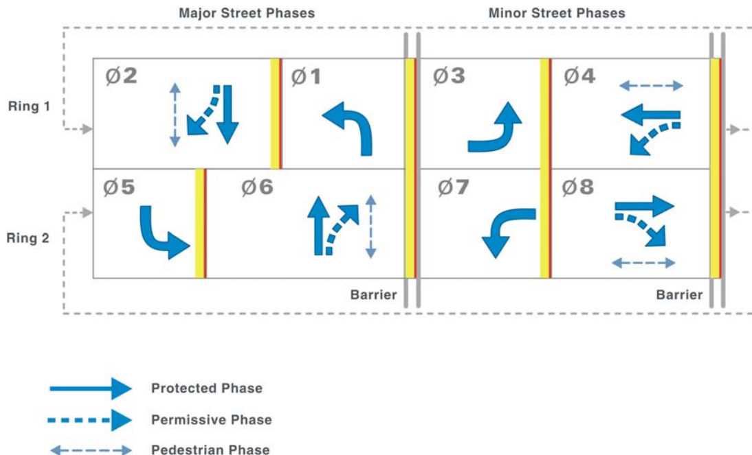
Figure 4-12 Ring-and-barrier diagram showing protected lead-lag left turns
