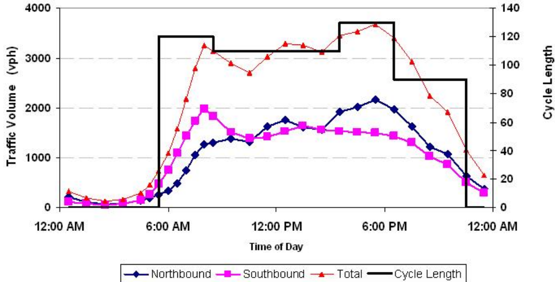
Figure 7-2 Traffic Volumes Summary Used to Determine Weekday Time of Day Plans
