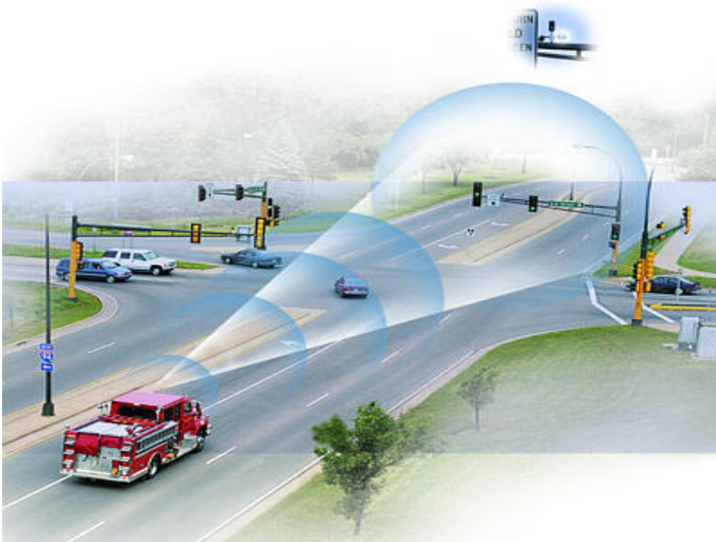
Figure 9-1 Emergency Vehicle Signal Preemption Example (2)
