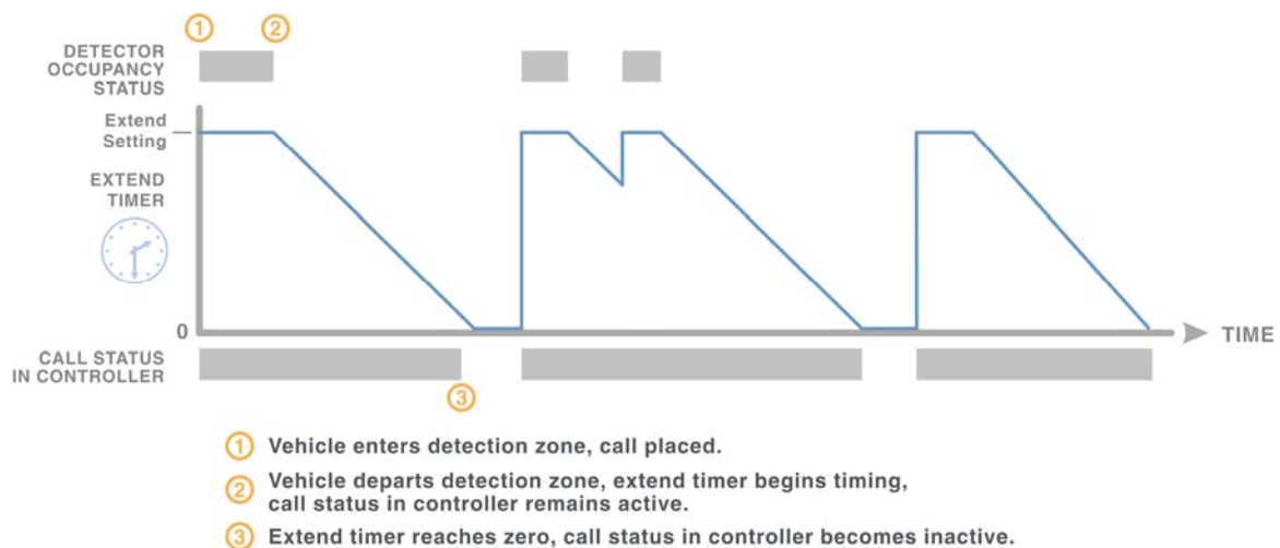
Figure 5-8 Application of extend timer
