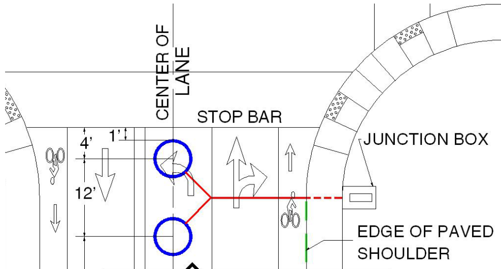
(a) Schematic design of loop detector design
