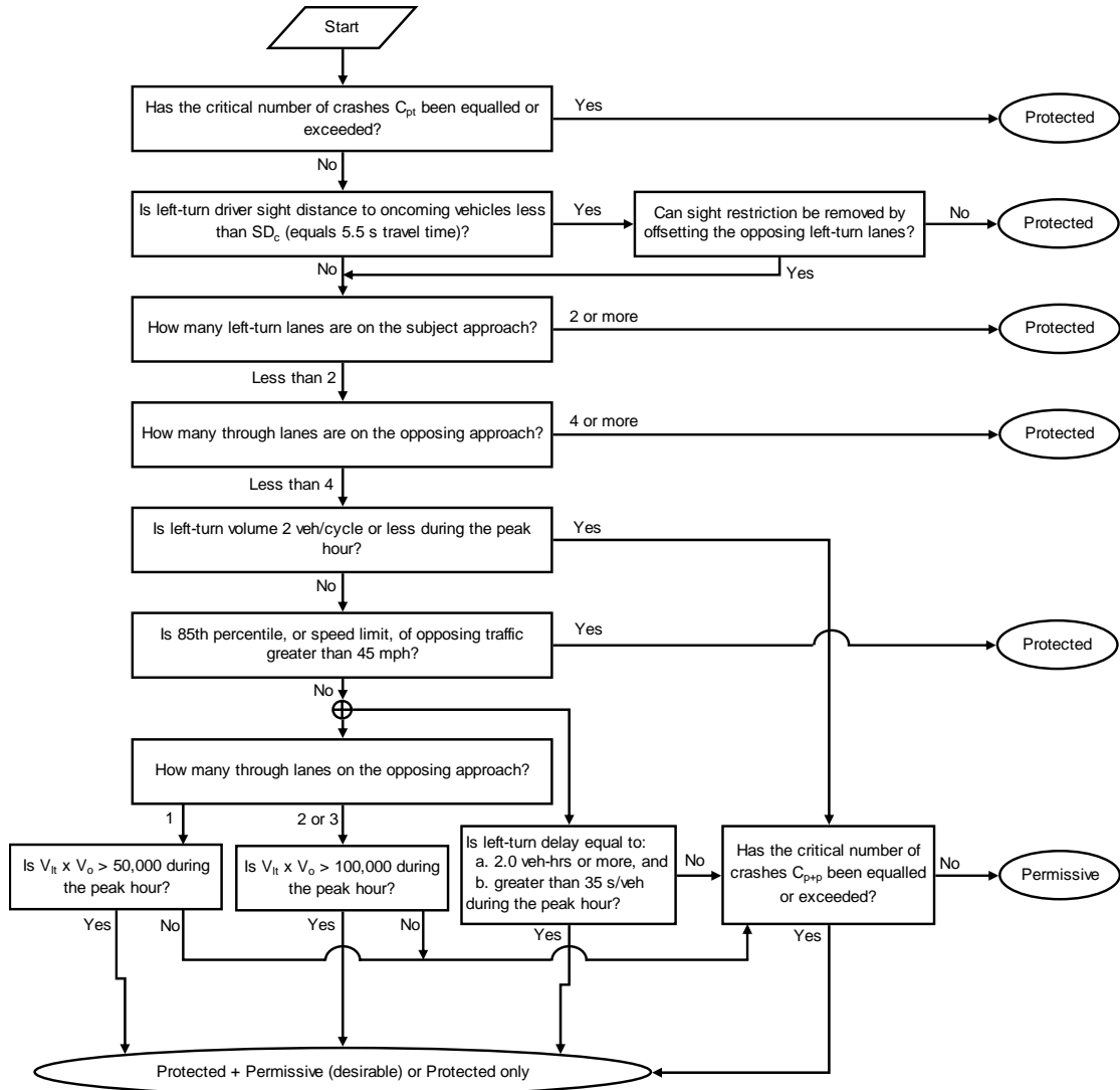
Figure 4-11 Guidelines for determining the potential need for a left-turn phase
