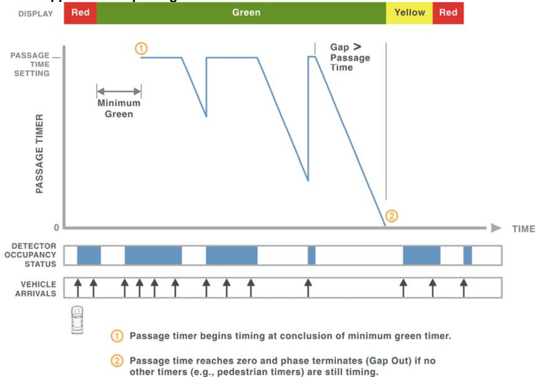
Figure 5-3 Application of passage time
