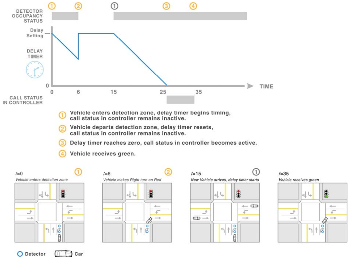
Figure 5-7 Application of delay timer
