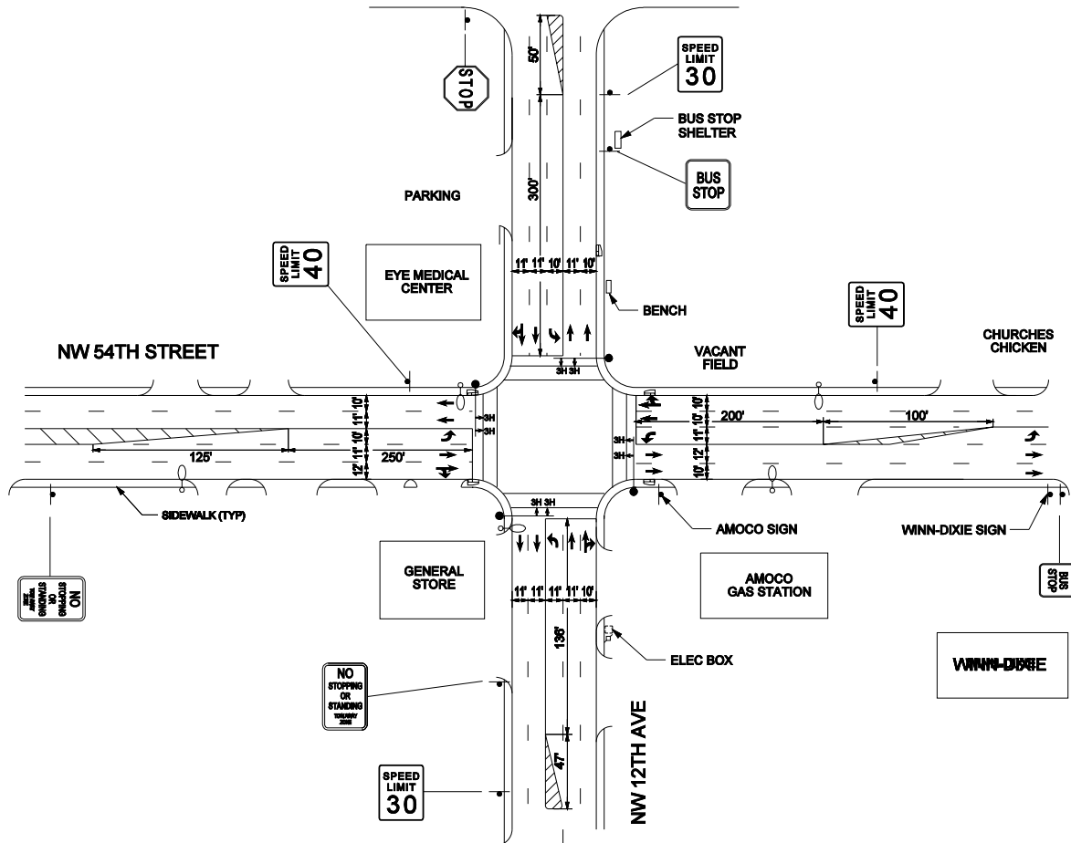
Figure 7-5 Example intersection condition diagram.
