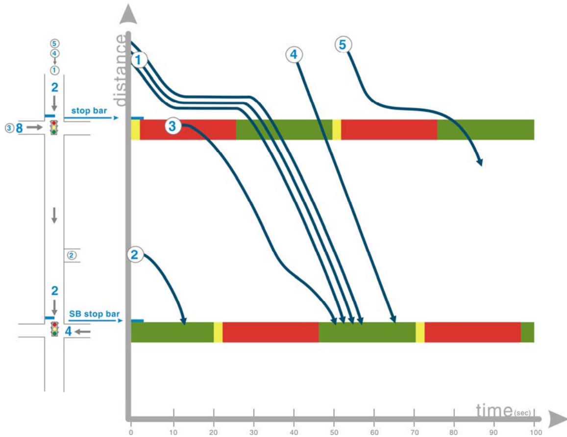
Figure 6-10 Time-Space Diagram – One-Way Street Operation
